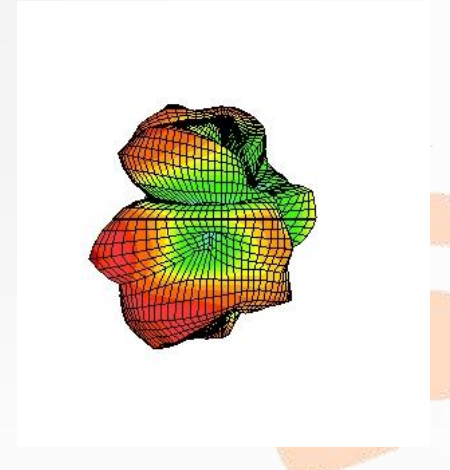
2.5GHzUp-Down View
