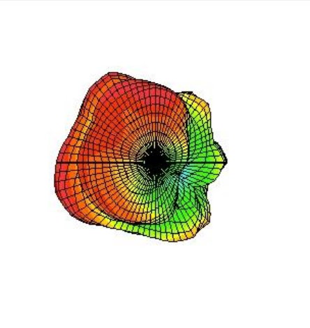
2.5GHzFront-Back View
