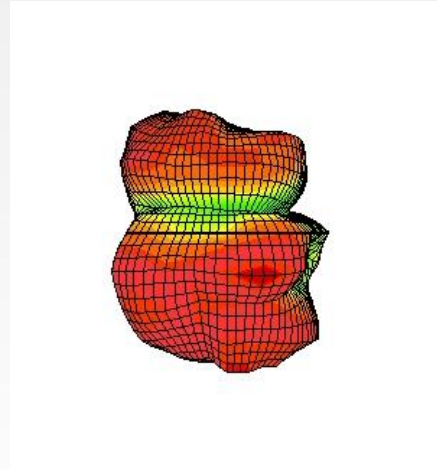
2.5GHzLeft-Right View
