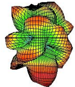
2.5GHzUp-Down View
