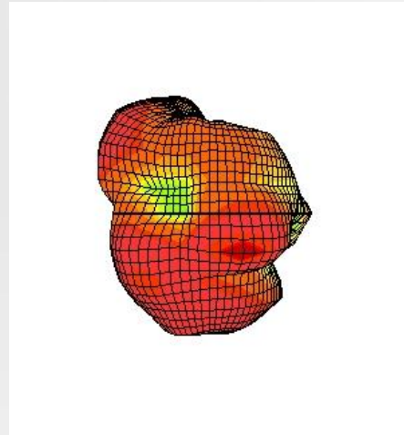
2.5GHzLeft-Right View
