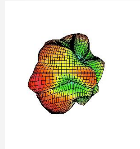
2.5GHzUp-Down View
