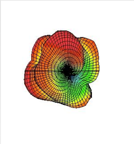
2.5GHzFront-Back View
