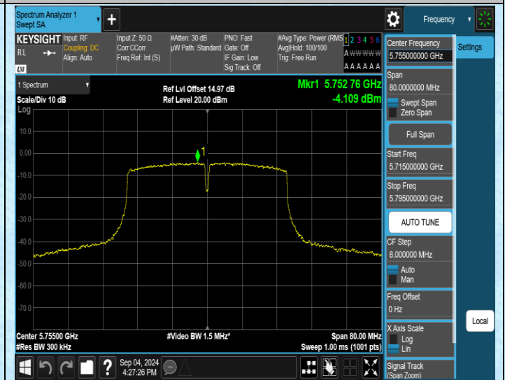
11AC40MIMO-Ant2-5755-PASS
