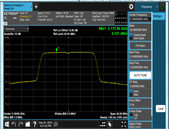
11AC20MIMO-Ant2-5180-PASS
