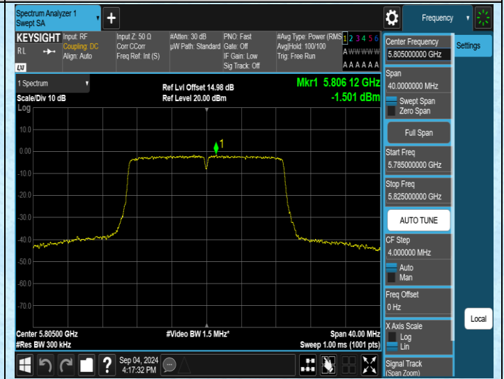
11AC20MIMO-Ant2-5805-PASS
