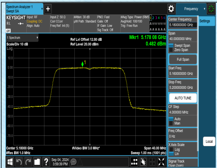
11AC20MIMO-Ant1-5180-PASS
