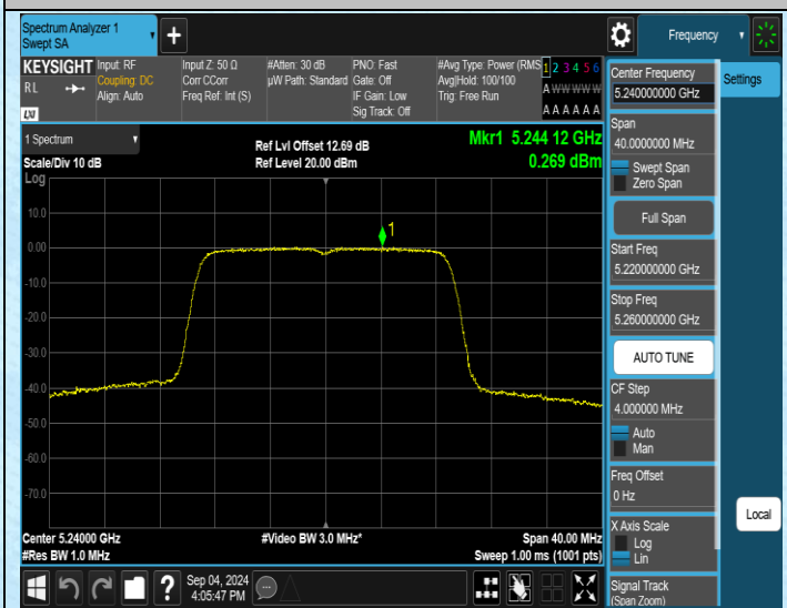
11AC20MIMO-Ant1-5240-PASS
