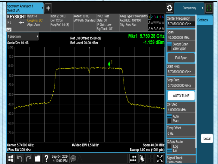
11AC20MIMO-Ant2-5745-PASS
