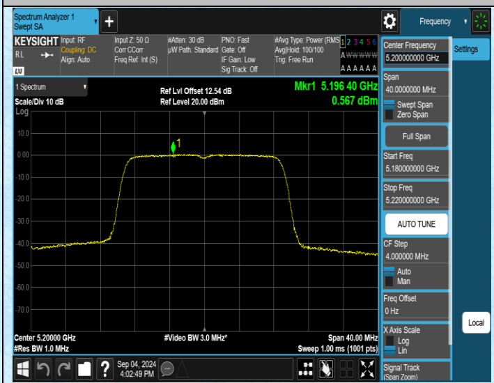
11AC20MIMO-Ant1-5200-PASS
