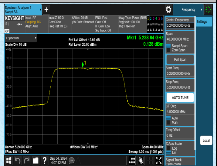
11AC20MIMO-Ant2-5240-PASS
