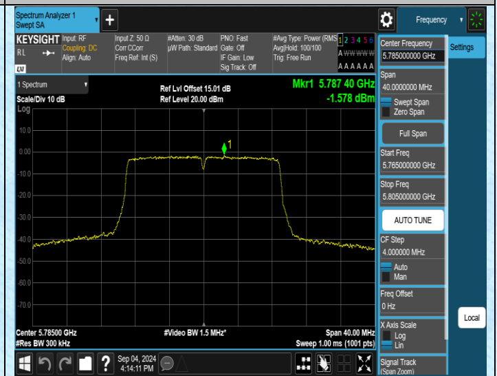
11AC20MIMO-Ant2-5785-PASS
