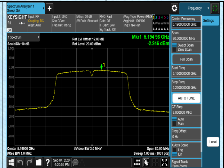
11AC40MIMO-Ant2-5190-PASS
