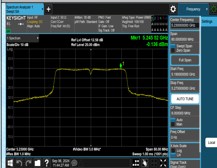
11AC40SISO-Ant3-5230-PASS
