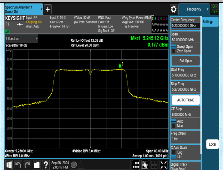
11AC40SISO-Ant4-5230-PASS
