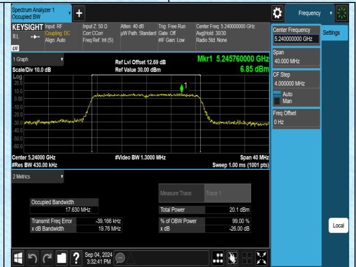
11AC20SISO-Ant2-5240
