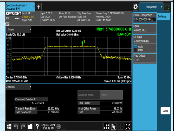
11AC20SISO-Ant2-5745
