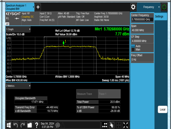
11AC20SISO-Ant2-5785
