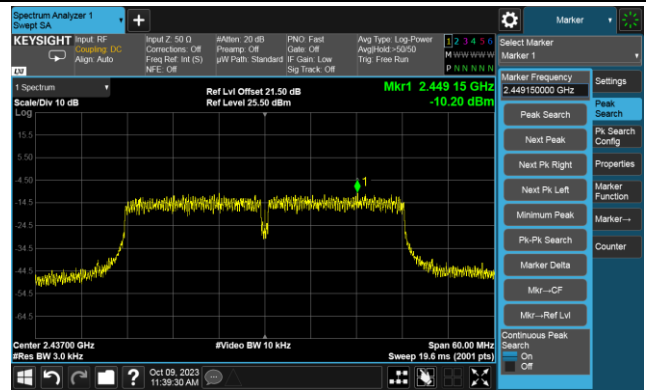
Channel 06 (2437MHz)
