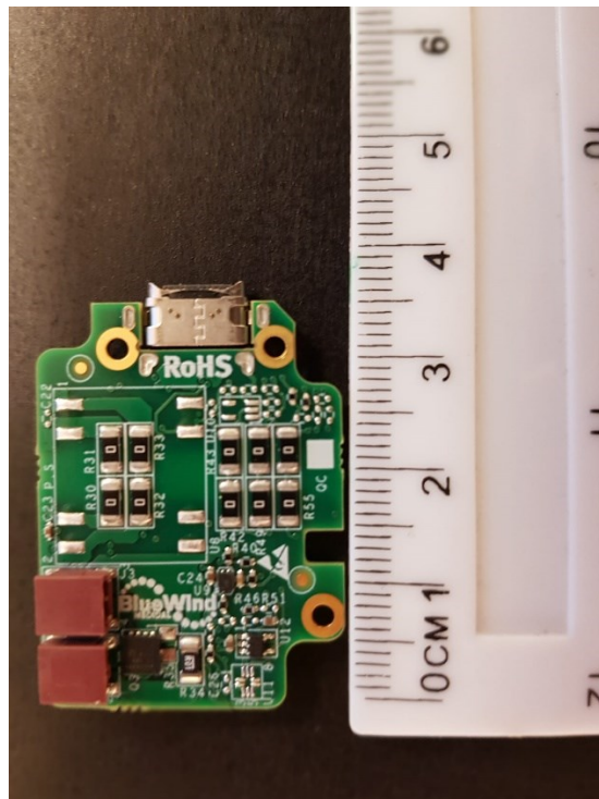
Figure 14 - ECU HW USB PCBA (Side 2)
