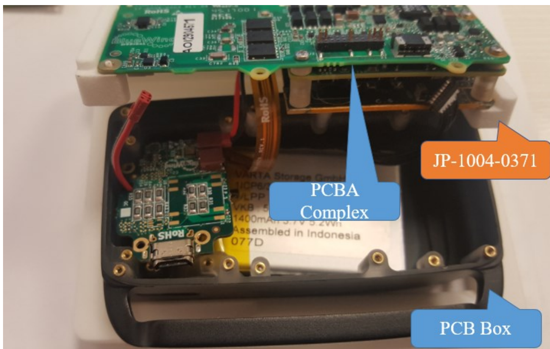
Figure 15 - ECU HW BOX Internal view
