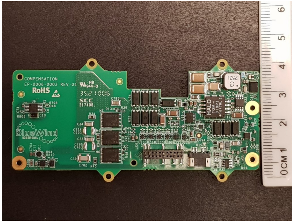
Figure 5 - ECU HW Compensation PCBA (Side 1)
