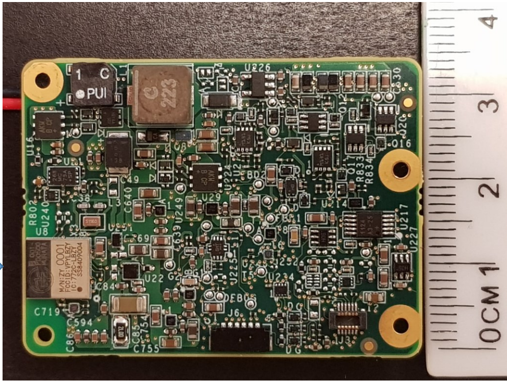
Figure 7 - ECU HW Main PCBA (Side 1)
