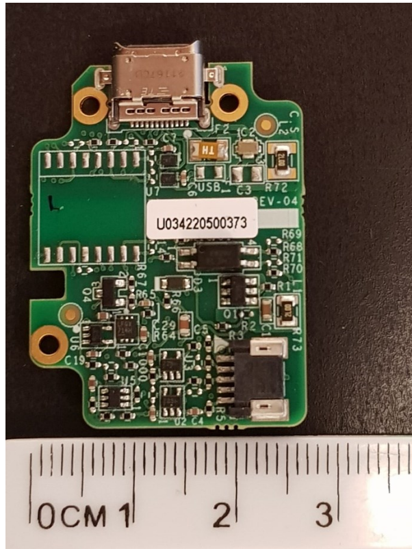
Figure 13 - ECU HW USB PCBA (Side 1)
