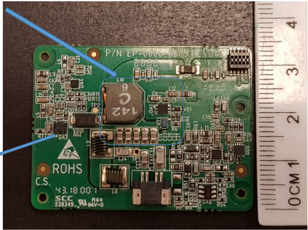
Figure 9 - ECU HW PA PCBA (Side 1)
