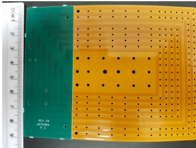
Figure 2 - ECU Antenna PCB - print side
