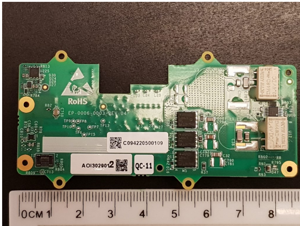
Figure 6 - ECU HW Compensation PCBA (Side 2)
