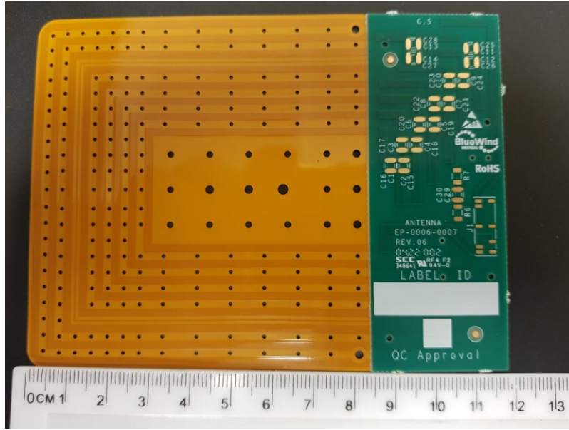
Figure 1 - ECU Antenna PCB - component side
