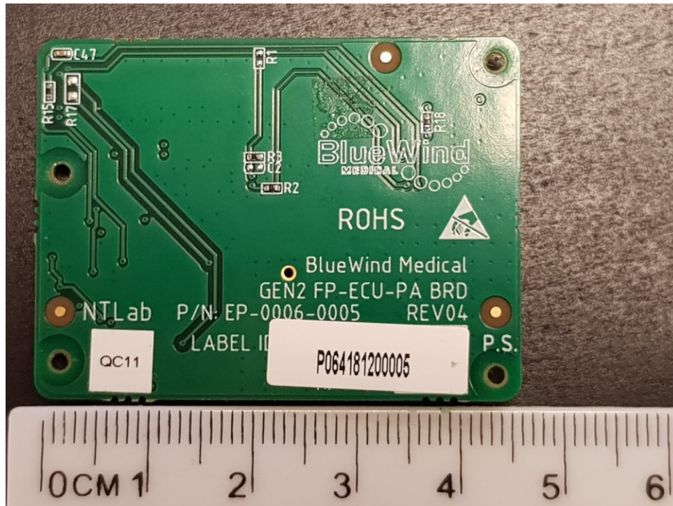
Figure 10 - ECU HWPA PCBA (Side 2)
