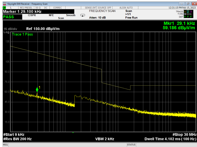
Plot 6.9 Radiated emission measurements, 9 kHz to 30 MHz, BLE high frequency Perpendicular
