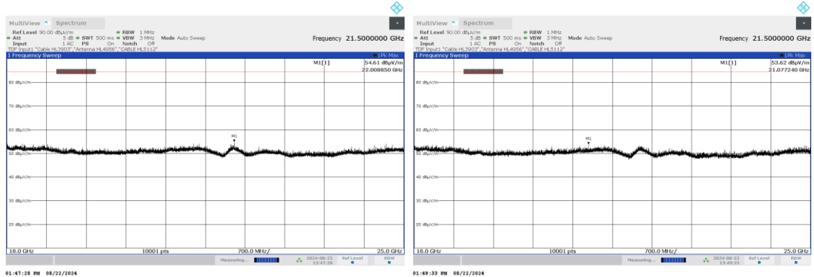
Plot 7.1.11 Radiated emission measurements from 18000 to 25000 MHz with LTE MF
