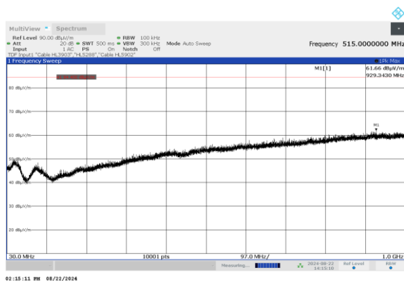
Plot 7.1.6 Radiated emission measurements from 30 to 1000 MHz with LTE HF
