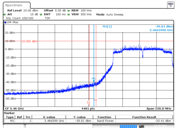
BE-NR-LOW, MIMO-B, 802.11ac80-VHT0, Ch106
