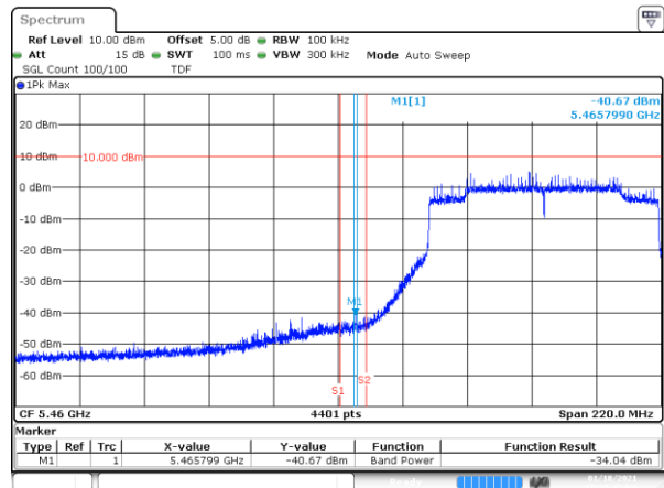
BE-NR-LOW, MIMO-B, 802.11ax80-HE0, Ch106
