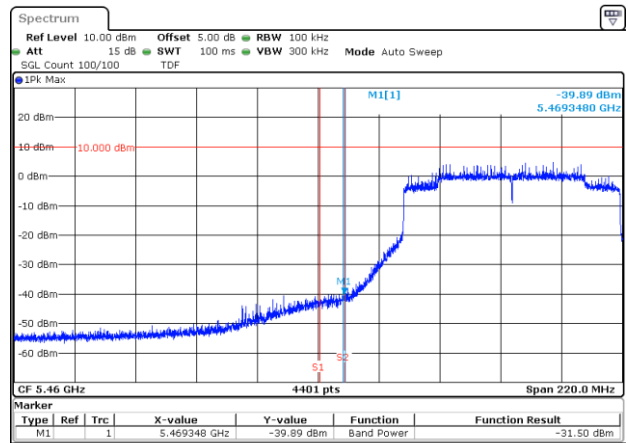
BE-NR-LOW, MIMO-A, 802.11ax80-HE0, Ch106
