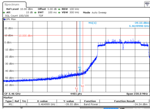
BE-NR-LOW, MIMO-A, 802.11ac80-VHT0, Ch106
