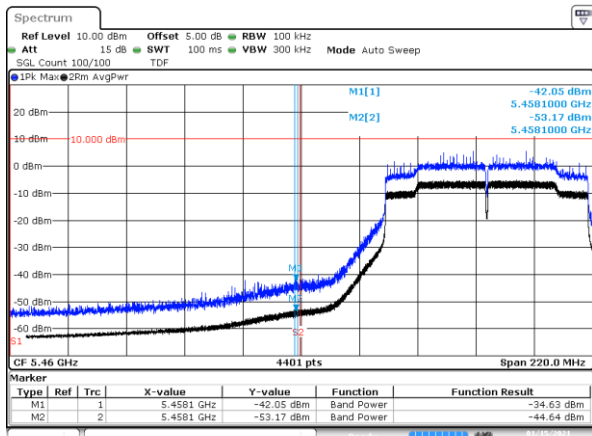
BE-R-LOW, MIMO-A, 802.11ac80-VHT0, Ch106
