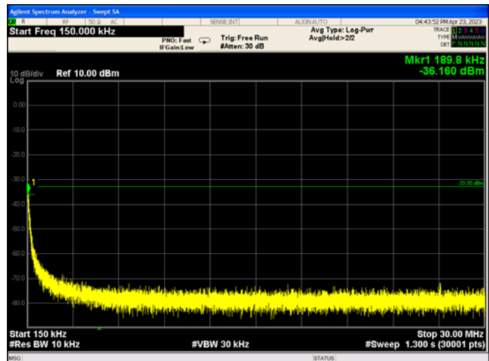
Band66_1.4MHz_QPSK_131979_1RB#5
