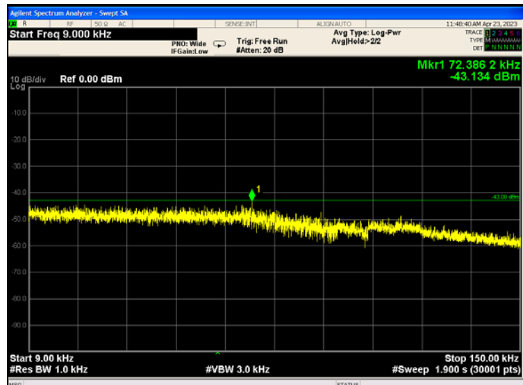
Band66_1.4MHz_QPSK_131979_1RB#5
