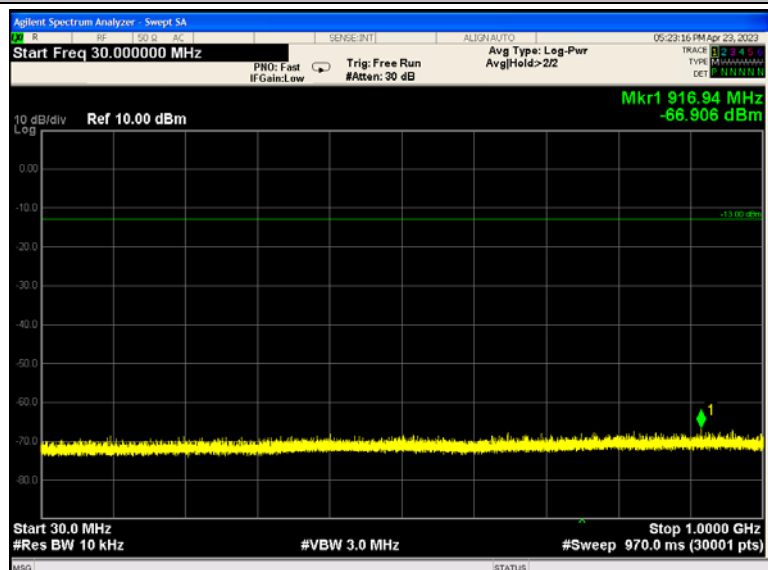
Band66_1.4MHz_QPSK_131979_1RB#5
