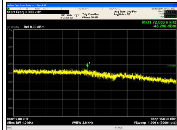
Band13_5MHz_QPSK_23205_1RB#12
