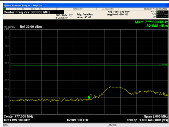
Band13_5MHz_QPSK_23205_1RB#24
