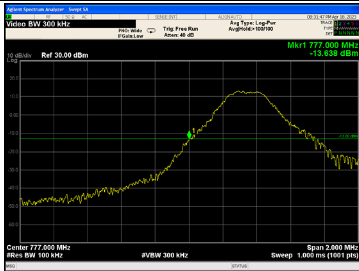
Band13_5MHz_QPSK_23205_1RB#12
