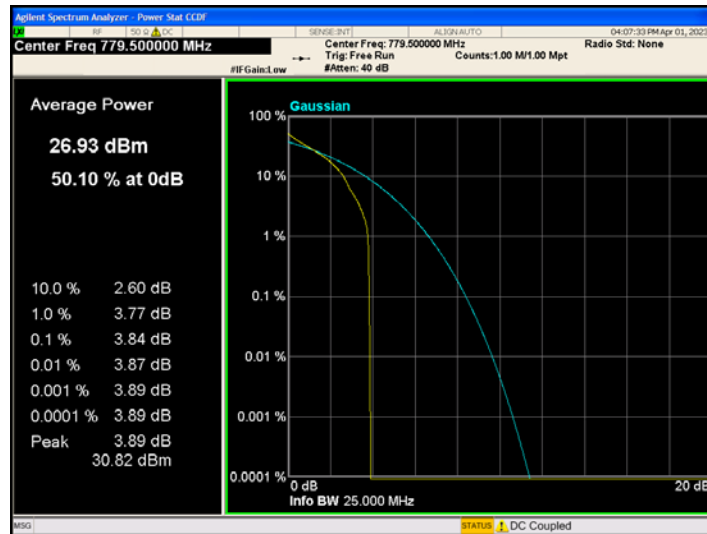
Band13_5MHz_QPSK_23205_25RB#0
