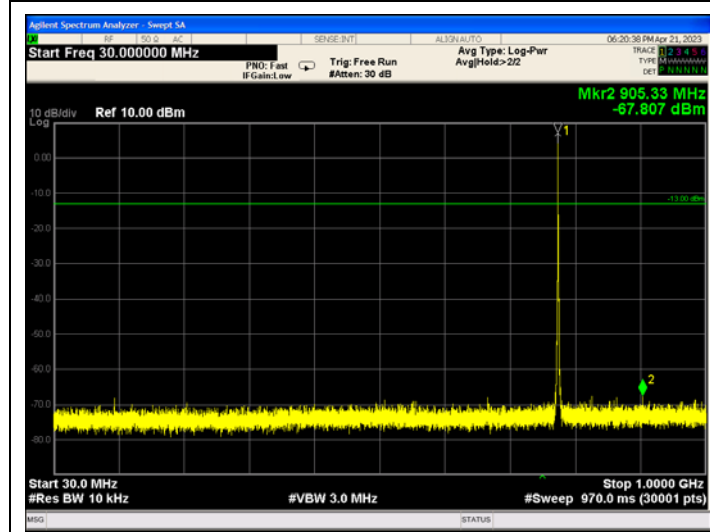
Band13_5MHz_QPSK_23205_1RB#12
