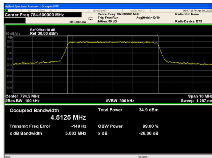
Band13_5MHz_QPSK_23255_25RB#0
