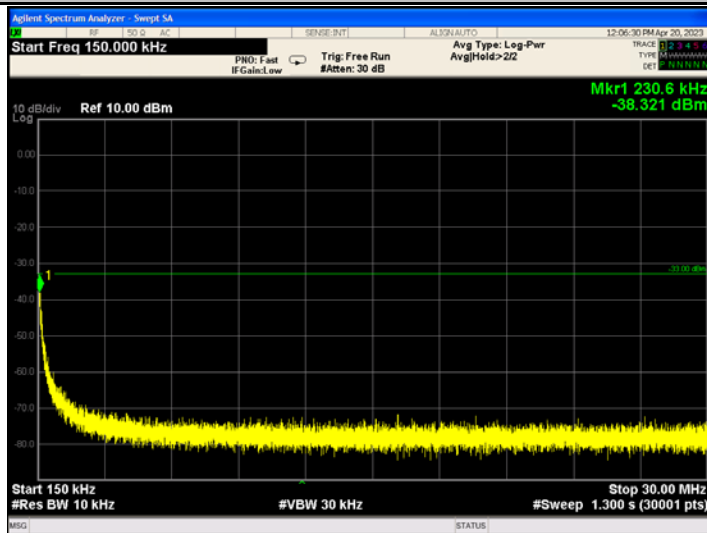
Band4_15MHz_16QAM_20325_1RB#38
