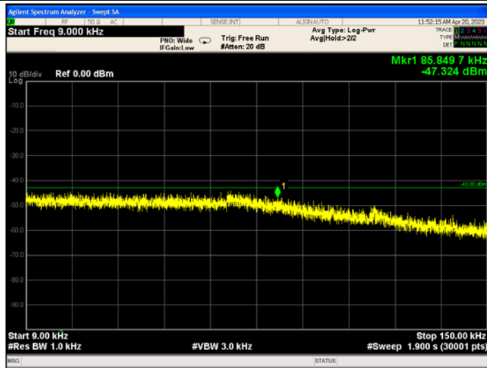
Band4_15MHz_16QAM_20325_1RB#38
