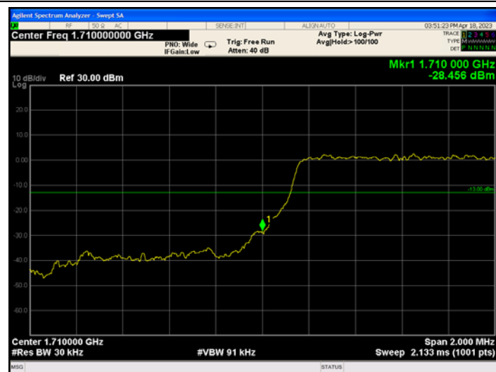
Band4-1.4MHz-QPSK-19957-6RB#0
