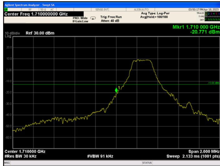
Band4-1.4MHz-QPSK-19957-1RB#5
