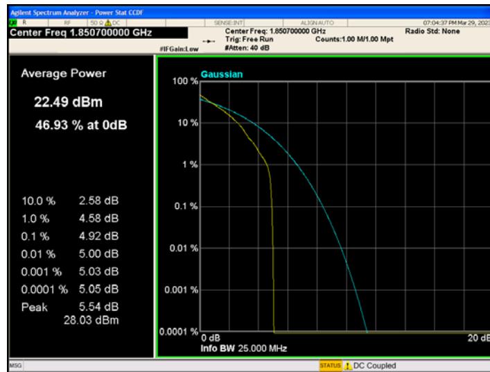
Band2-1.4MHz-QPSK-18607-6RB#0
