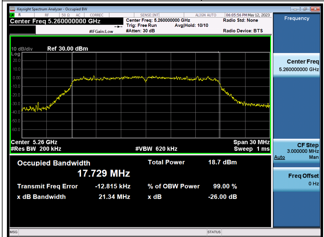
802.11n20_ANT1_5260_MCS0_OBW
