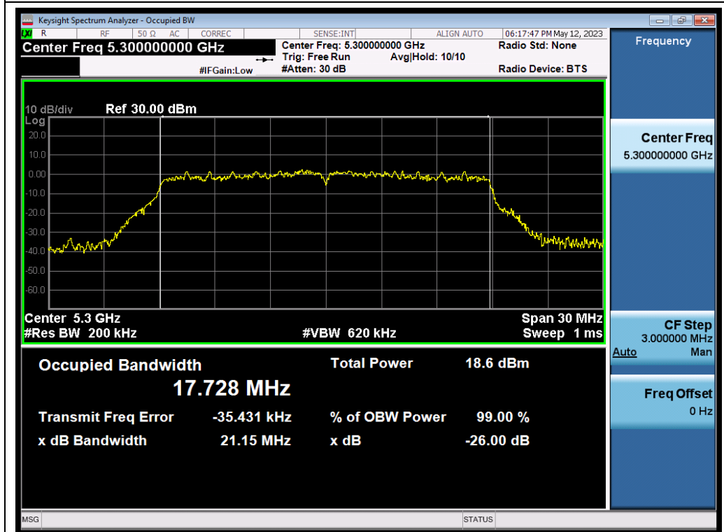
802.11ac20_ANT1_5300_MCS0_OBW
