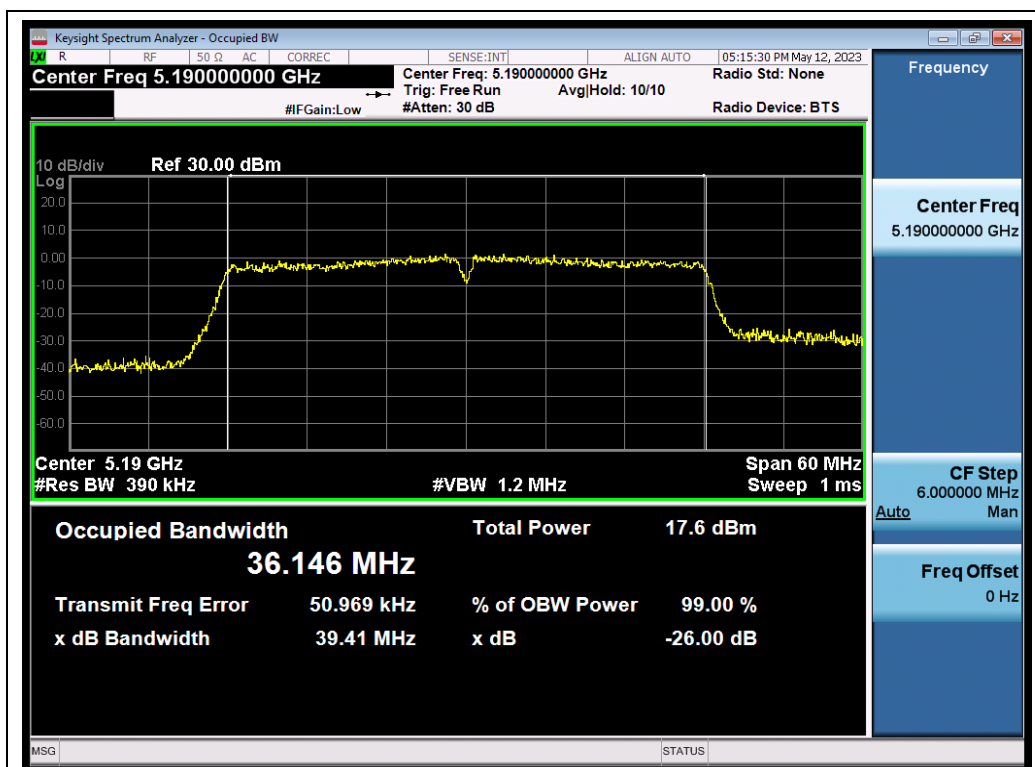
802.11n40_ANT1_5190_MCS0_OBW
