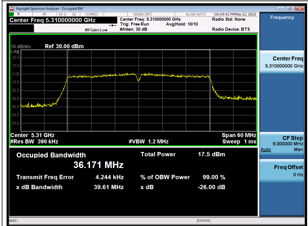
802.11n40_ANT1_5310_MCS0_OBW
