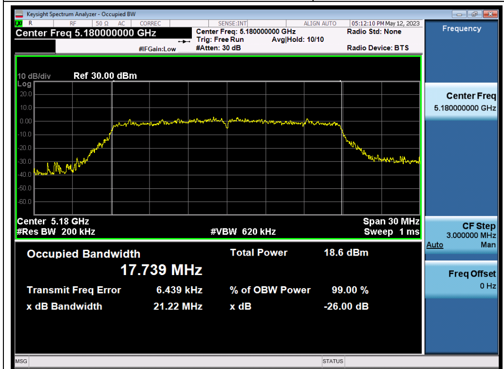
802.11n20_ANT1_5180_MCS0_OBW
