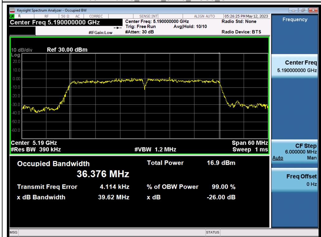
802.11ac40_ANT1_5190_MCS0_OBW
