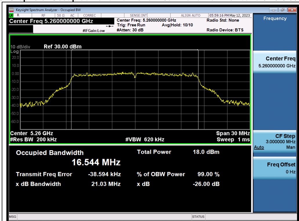
802.11a_ANT1_5260_6Mbps_OBW
