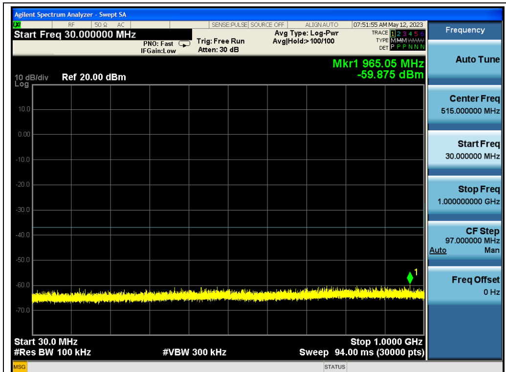
802.11ac80 ANT1 5210 MCS0 Frequency Band 1
