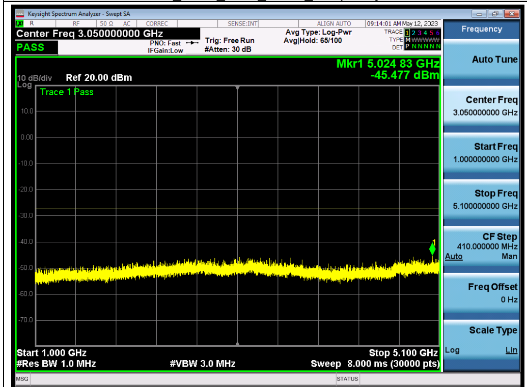
802.11n40_ANT1_5310_MCS0_Frequency Band 2
