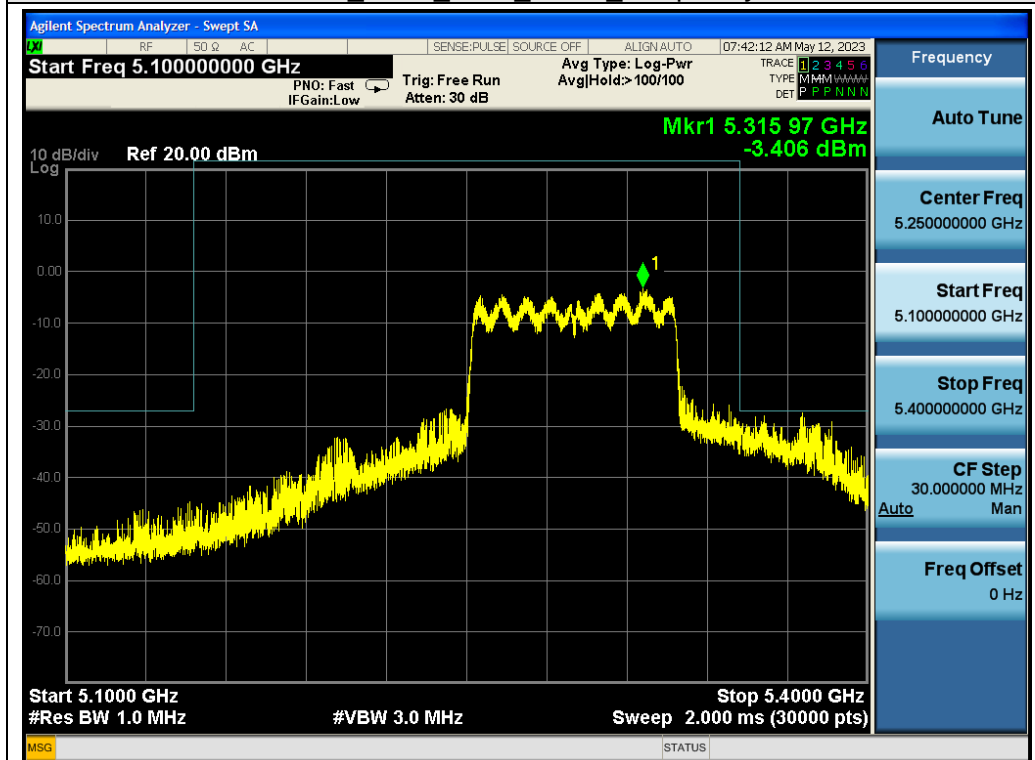
802.11ac80 ANT1_5290_MCS0 Frequency Band 3
