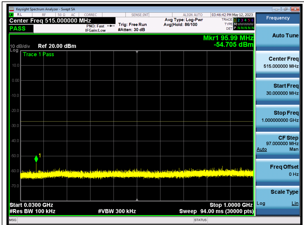
802.11a_ANT1_5745_6Mbps_Frequency Band1
