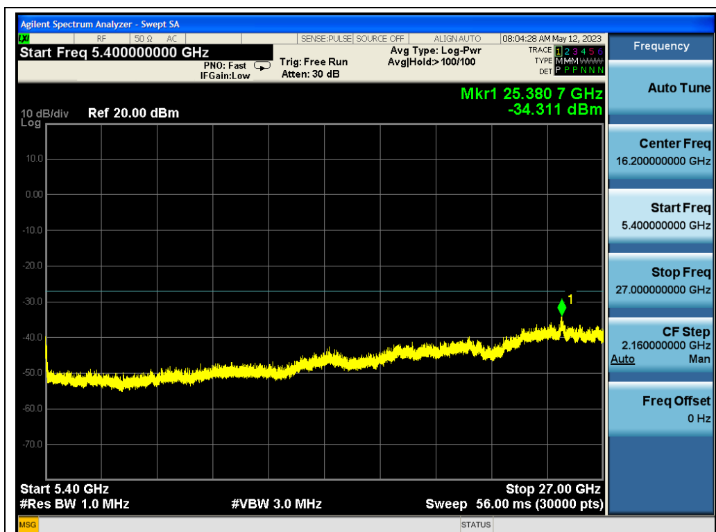
802.11ac80 ANT1 5290 MCS0 Frequency Band 4
