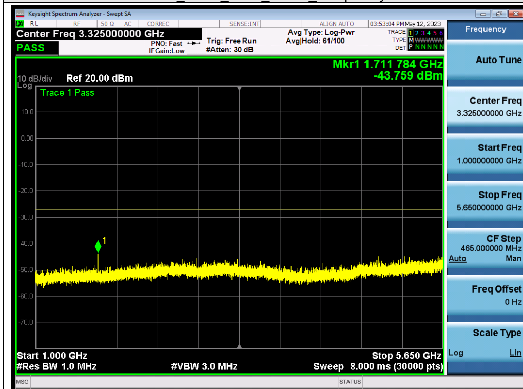
802.11n40_ANT1_5755_MCS0_Frequency Band2
