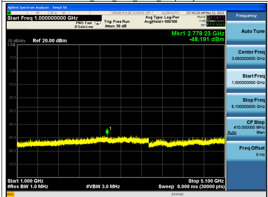
802.11ac80 ANT1 5210 MCS0 Frequency Band 2
