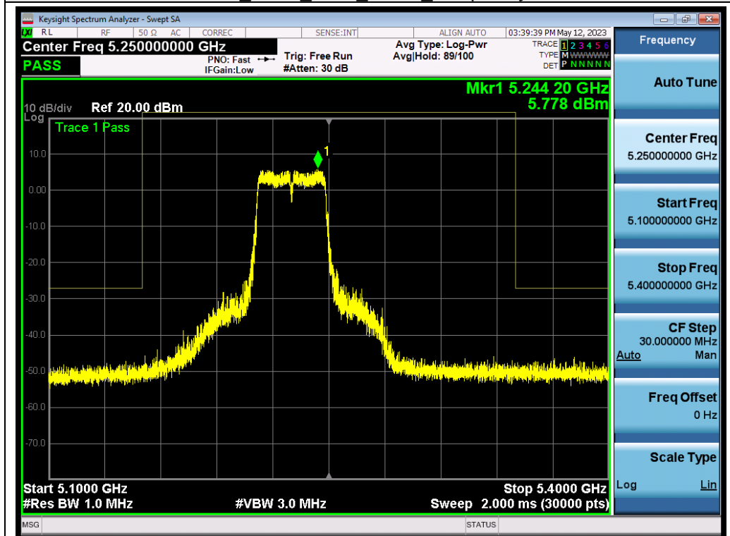
802.11n40_ANT1_5230_MCS0_Frequency Band 3
