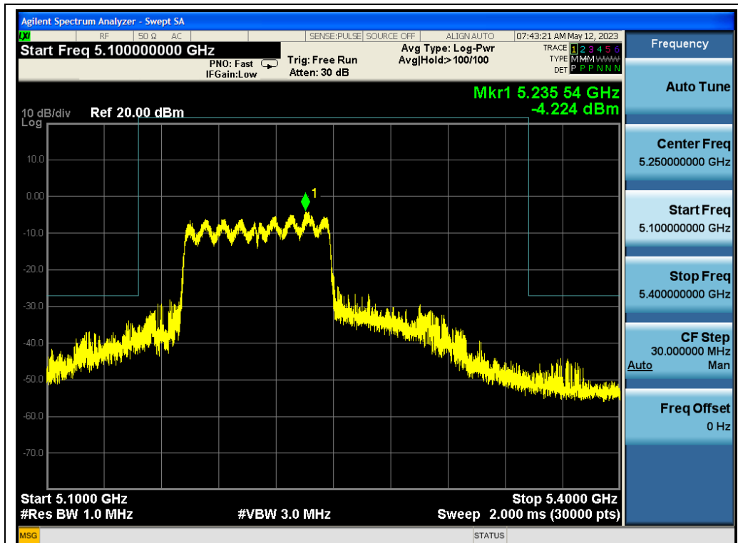
802.11ac80_ANT1_5210_MCS0_Frequency Band 3
