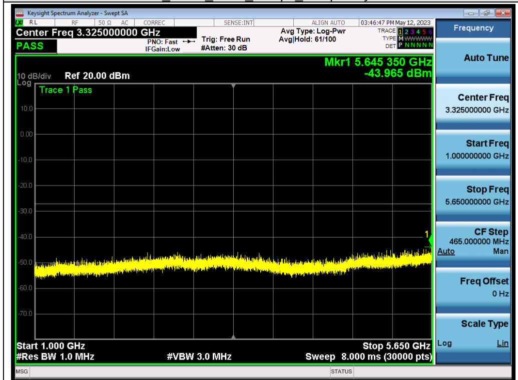
802.11a_ANT1_5745_6Mbps_Frequency Band2
