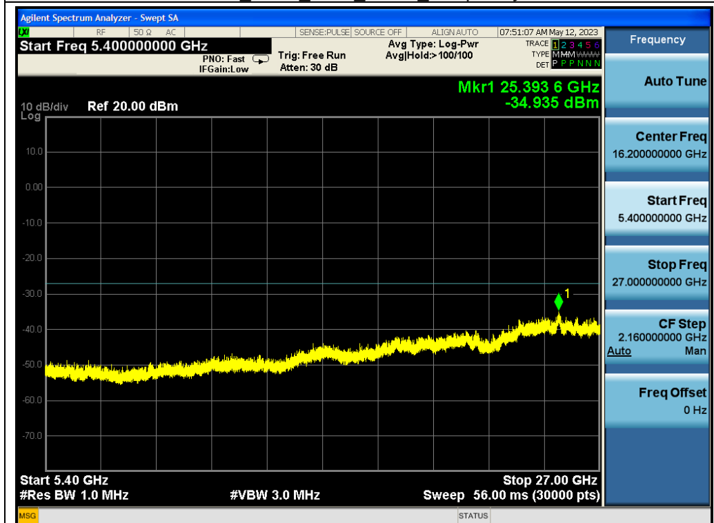
802.11ac80_ANT1_5210_MCS0_Frequency Band 4
