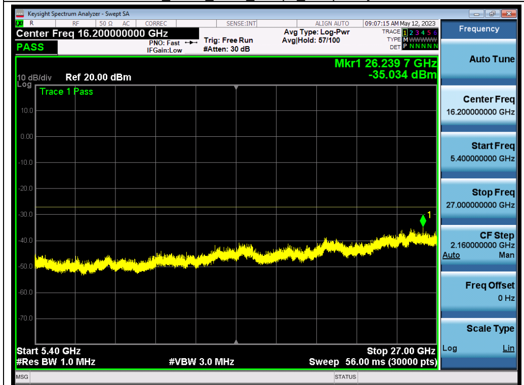
802.11a ANT1_5320_6Mbps Frequency Band 4
