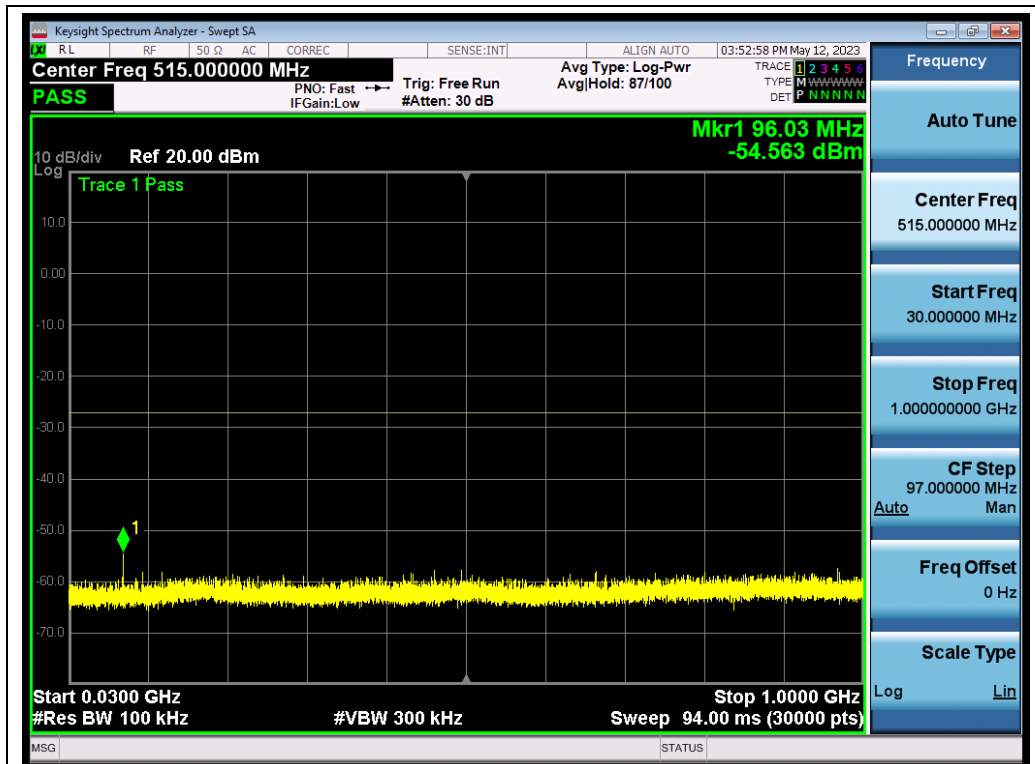
802.11n40_ANT1_5755_MCS0_Frequency Band1
