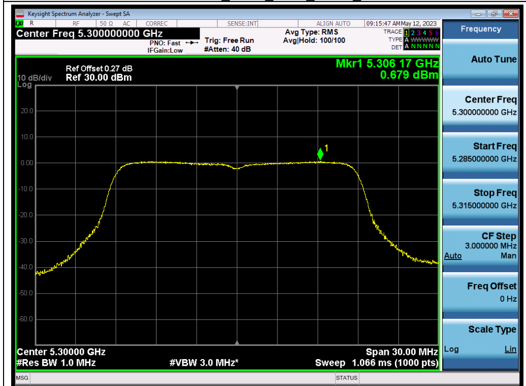
802.11ac20_ANT1_5300_MCS0_PSD
