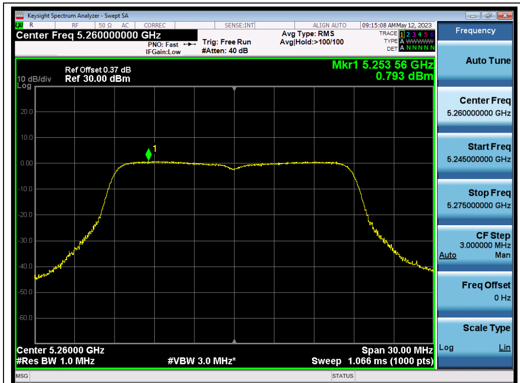
802.11ac20_ANT1_5260_MCS0_PSD
