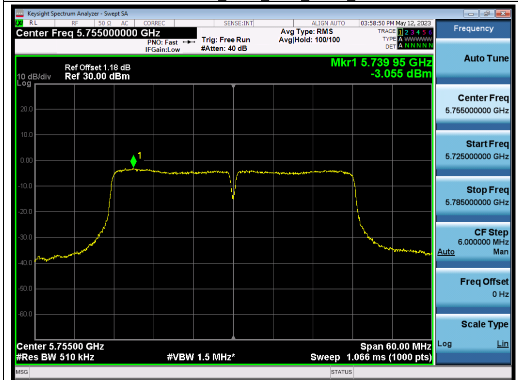
802.11ac40_ANT1_5755_MCS0_PSD
