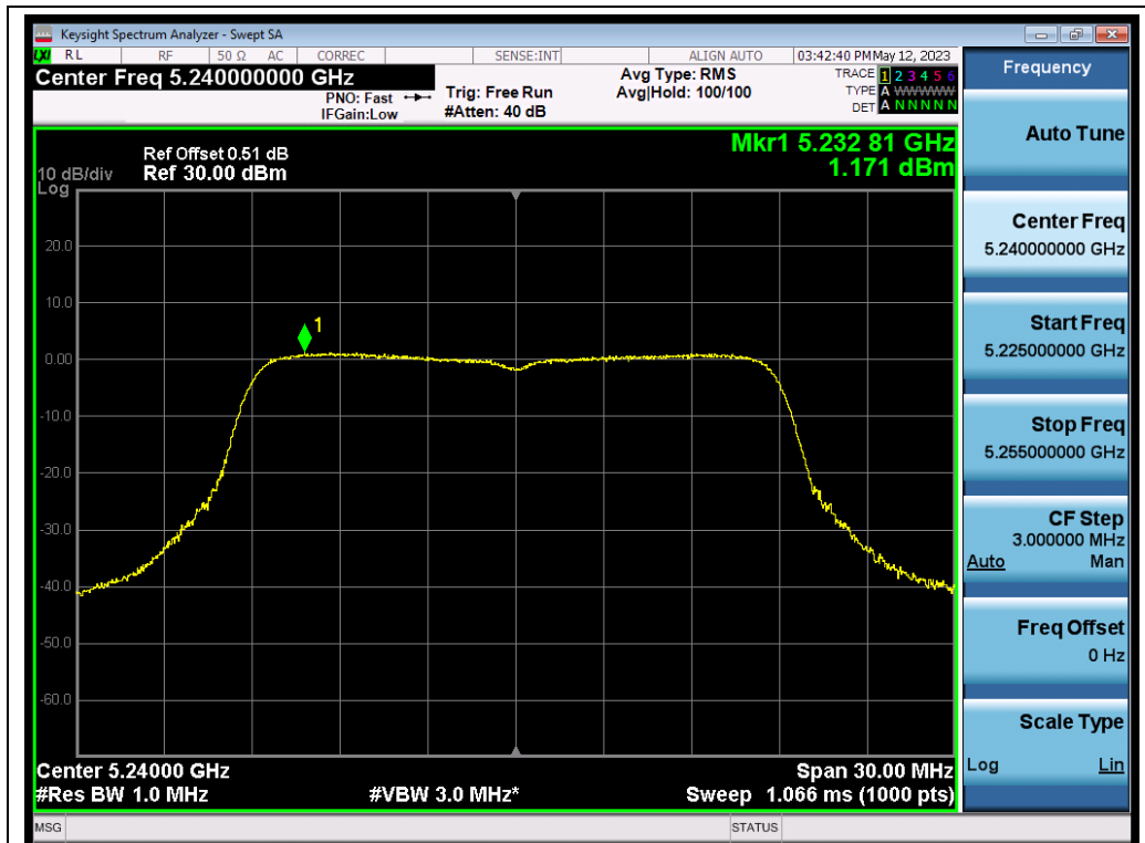
802.11ac20_ANT1_5240_MCS0_PSD
