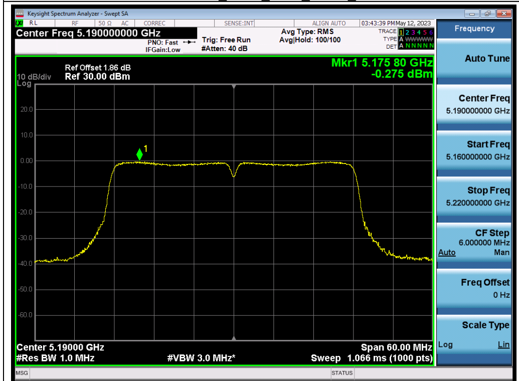
802.11ac40_ANT1_5190_MCS0_PSD
