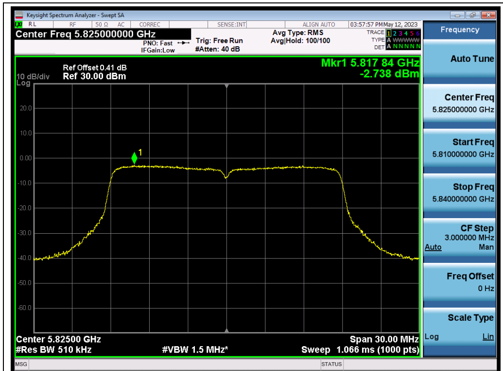
802.11ac20_ANT1_5825_MCS0_PSD
