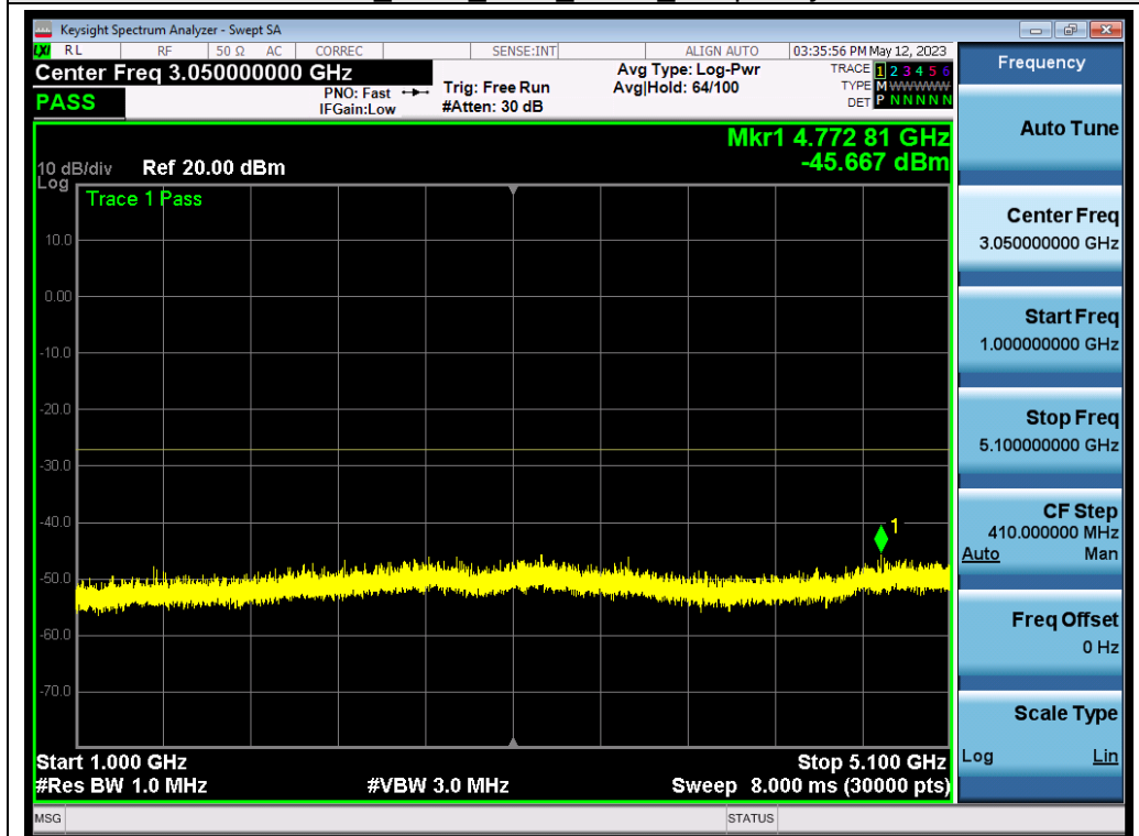
802.11n40_ANT1_5190_MCS0_Frequency Band 2
