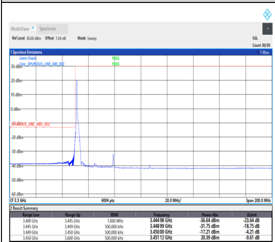
1-N78-3450-3550--30-30-L-1-DFT-PI2BPSK-Edge_1RB_Left-1@0-Ant1-1---see graph
