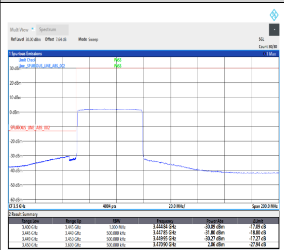
1-N78-3450-3550--30-50-L-6-CP-QPSK-Outer_Full-133@0-Ant1-1---see graph
