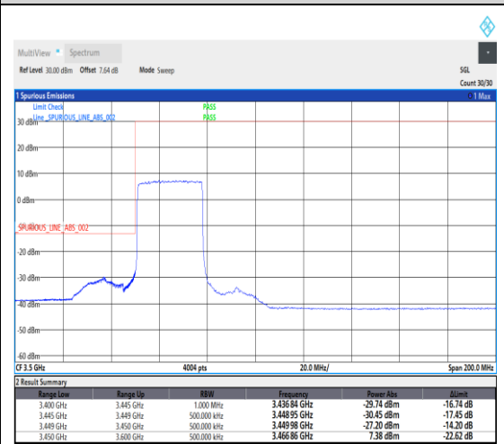
1-N78-3450-3550--30-30-L-3-DFT-PI2BPSK-Outer_Full-75@0-Ant1-1---see graph
