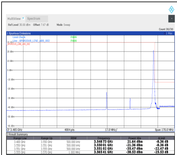
1-N78-3450-3550--30-50-H-2-DFT-PI2BPSK-Edge_1RB_Right-1@132-Ant1-1---see graph
