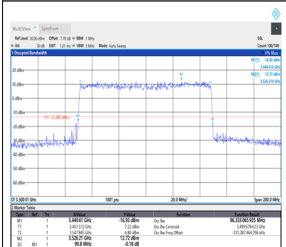
1-N78-3450-3550--30-100-H-4-DFT-64QAM- Outer_Full-270@0-Ant1-96.333-99.800-≤100 -
