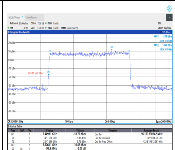
1-N78-3450-3550--30-100-H-5-DFT-256QAM -Outer_Full-270@0-Ant1-96.16-99.800-≤100- -
