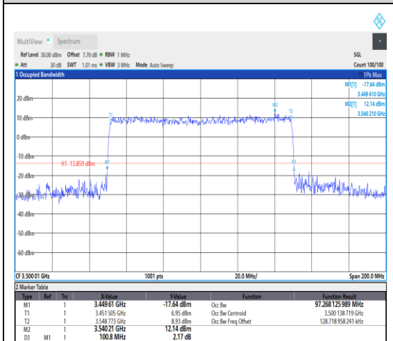
1-N78-3450-3550--30-100-H-6-CP-QPSK-Ou
