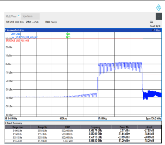
1-N78-3450-3550--30-50-H-6-CP-QPSK-Outer_Full-133@0-Ant1-1---see graph
