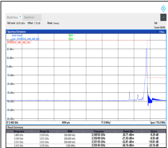
1-N78-3450-3550--30-20-H-2-DFT-PI2BPSK-Edge_1RB_Right-1@50-Ant1-1---see graph
