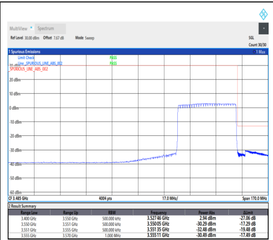
1-N78-3450-3550--30-40-H-6-CP-QPSK-Out_er_Full-106@0-Ant1-1---see graph
