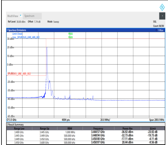
1-N78-3450-3550--30-60-L-1-DFT-PI2BPSK-Edge_1RB_Left-1@0-Ant1-1---see graph
