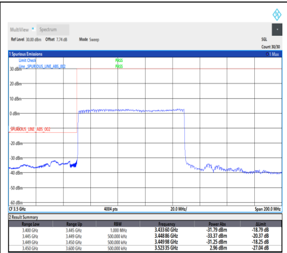
1-N78-3450-3550--30-80-L-3-DFT-PI2BPSK-Outer_Full-216@0-Ant1-1---see graph
