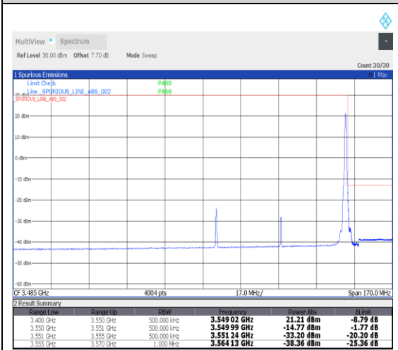
1-N78-3450-3550--30-60-H-5-CP-QPSK-Edge_1RB_Right-1@161-Ant1-1---see graph
