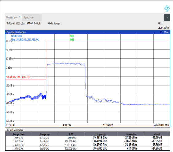
1-N78-3450-3550--30-50-L-3-DFT-PI2BPSK-Outer_Full-128@0-Ant1-1---see graph
