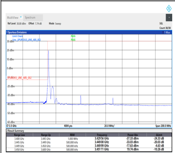
1-N78-3450-3550--30-80-L-4-CP-QPSK-Edge_1RB_Left-1@0-Ant1-1---see graph
