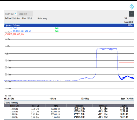
1-N78-3450-3550--30-30-H-3-DFT-PI2BPSK-Outer_Full-75@0-Ant1-1---see graph
