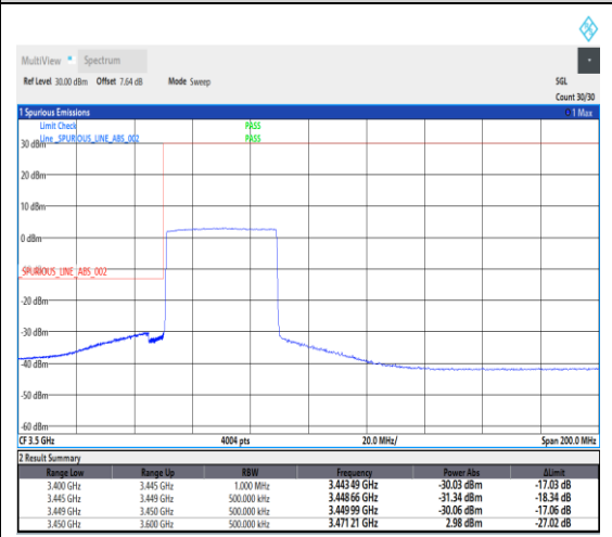
1-N78-3450-3550--30-40-L-6-CP-QPSK-Outer_Full-106@0-Ant1-1---see graph
