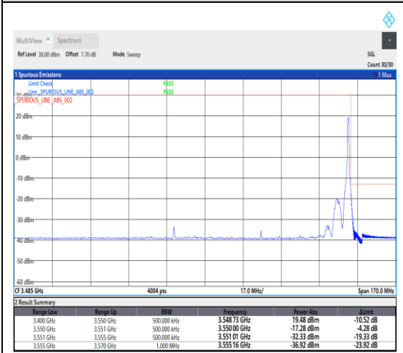
1-N78-3450-3550--30-80-H-2-DFT-PI2BPSK-Edge_1RB_Right-1@216-Ant1-1---see graph
