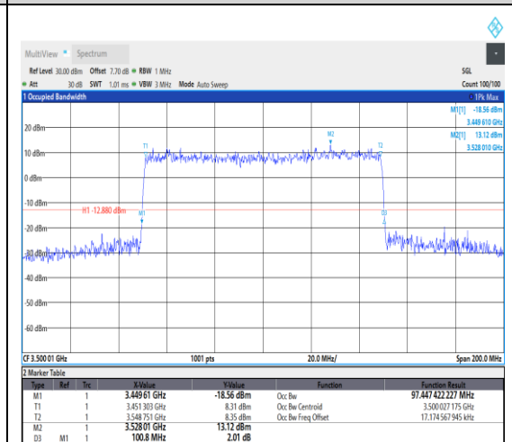
1-N78-3450-3550--30-100-H-7-CP-16QAM-O
