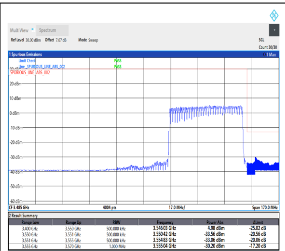
1-N78-3450-3550--30-50-H-3-DFT-PI2BPSK-Outer_Full-128@0-Ant1-1---see graph
