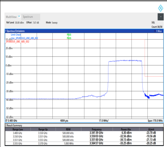
1-N78-3450-3550--30-40-H-3-DFT-PI2BPSK-Outer_Full-100@0-Ant1-1---see graph
