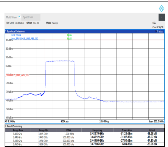
1-N78-3450-3550--30-40-L-3-DFT-PI2BPSK-Outer_Full-100@0-Ant1-1---see graph
