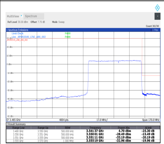
1-N78-3450-3550--30-60-H-3-DFT-PI2BPSK-Outer_Full-162@0-Ant1-1---see graph
