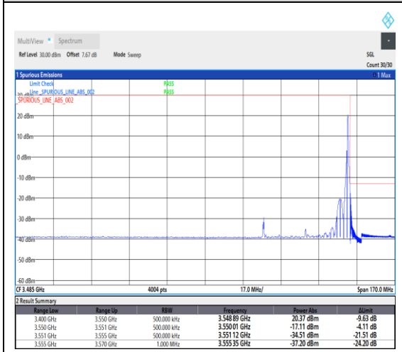
1-N78-3450-3550--30-40-H-2-DFT-PI2BPSK-Edge_1RB_Right-1@105-Ant1-1---see graph
