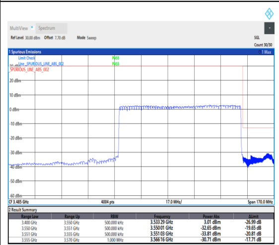
1-N78-3450-3550--30-80-H-3-DFT-PI2BPSK-Outer_Full-216@0-Ant1-1---see graph
