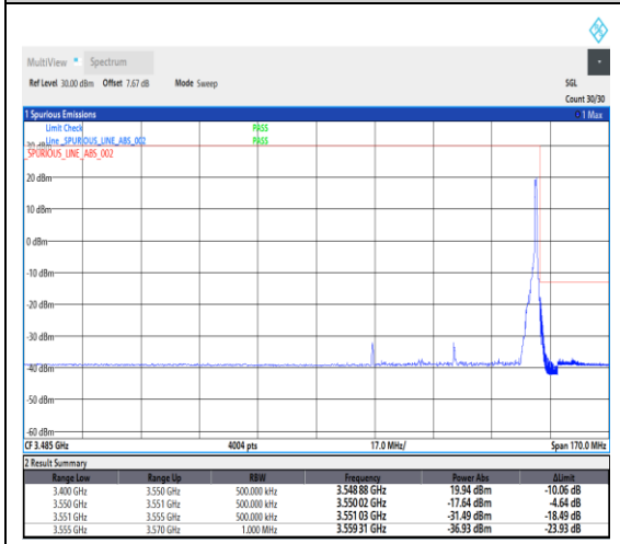
1-N78-3450-3550--30-50-H-5-CP-QPSK-Edge_1RB_Right-1@132-Ant1-1---see graph
