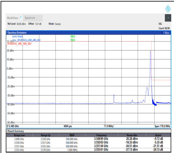
1-N78-3450-3550--30-40-H-5-CP-QPSK-Edge_1RB_Right-1@105-Ant1-1---see graph
