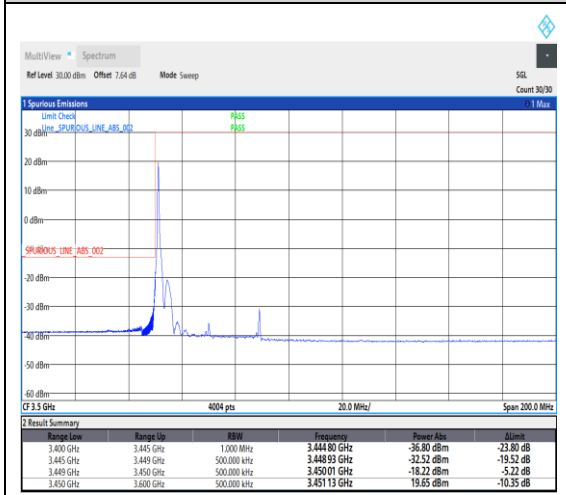
1-N78-3450-3550--30-40-L-4-CP-QPSK-Edge_1RB_Left-1@0-Ant1-1---see graph
