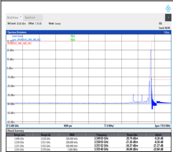
1-N78-3450-3550--30-20-H-5-CP-QPSK-Edge_1RB_Right-1@50-Ant1-1---see graph
