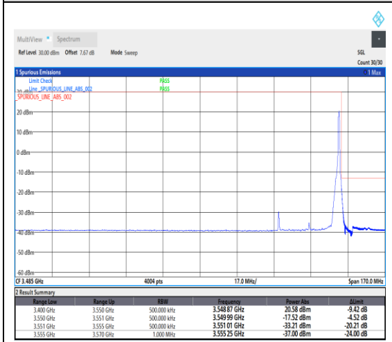
1-N78-3450-3550--30-30-H-2-DFT-PI2BPSK-Edge_1RB_Right-1@77-Ant1-1---see graph
