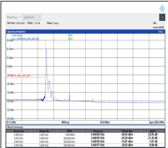
1-N78-3450-3550--30-60-L-4-CP-QPSK-Edge_1RB_Left-1@0-Ant1-1---see graph
