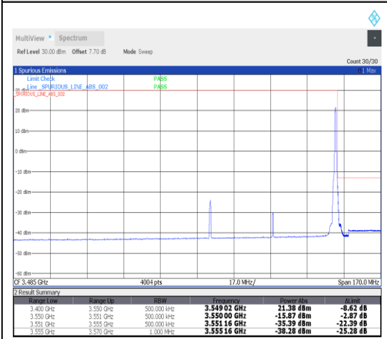
1-N78-3450-3550--30-60-H-2-DFT-PI2BPSK-Edge_1RB_Right-1@161-Ant1-1---see graph
