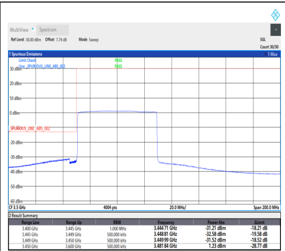
1-N78-3450-3550--30-60-L-6-CP-QPSK-Outer_Full-162@0-Ant1-1---see graph
