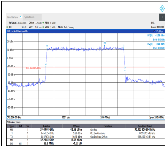
1-N78-3450-3550--30-100-H-2-DFT-PI2BPS K-Outer_Full-270@0-Ant1-96.324-99.800-≤1 00-
