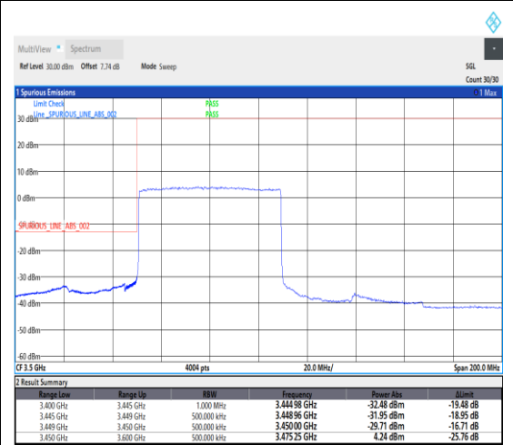
1-N78-3450-3550--30-60-L-3-DFT-PI2BPSK-Outer_Full-162@0-Ant1-1---see graph
