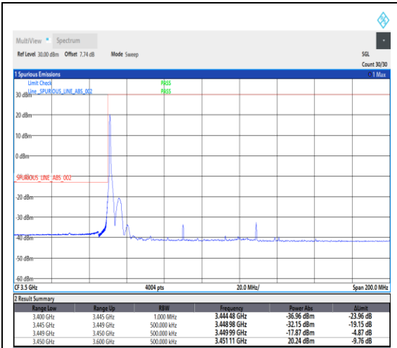
1-N78-3450-3550--30-80-L-1-DFT-PI2BPSK-Edge_1RB_Left-1@0-Ant1-1---see graph
