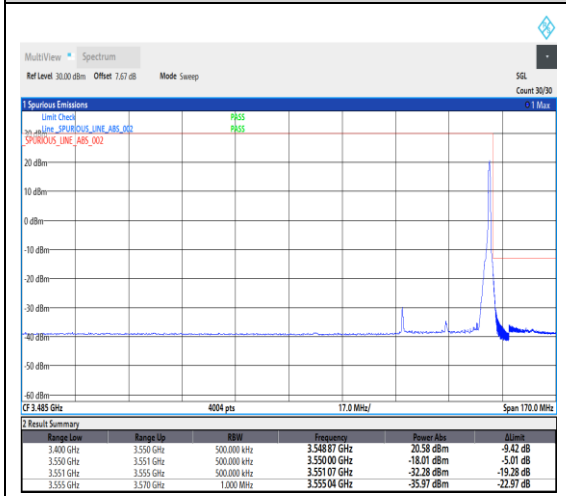
1-N78-3450-3550--30-30-H-5-CP-QPSK-Edge_1RB_Right-1@77-Ant1-1---see graph
