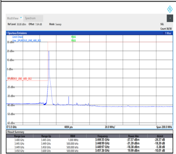
1-N78-3450-3550--30-50-L-4-CP-QPSK-Edge_1RB_Left-1@0-Ant1-1---see graph
