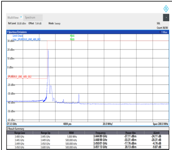
1-N78-3450-3550--30-40-L-1-DFT-PI2BPSK-Edge_1RB_Left-1@0-Ant1-1---see graph
