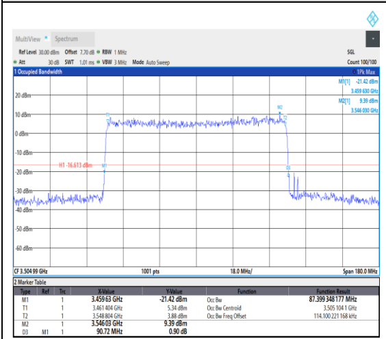
1-N78-3450-3550--30-90-H-9-CP-256QAM-Outer_Full-245@0-Ant1-87.399-90.720≤90-
