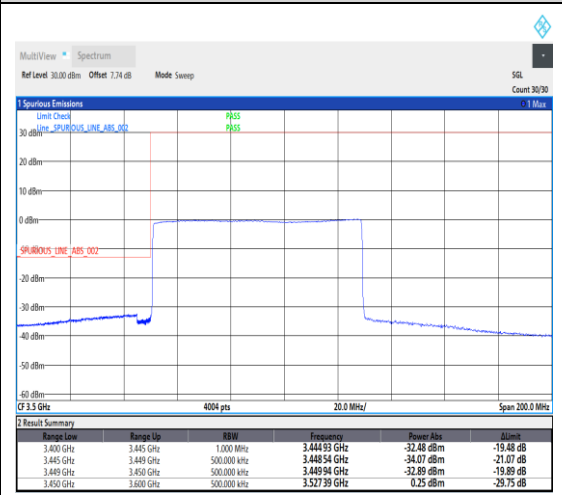
1-N78-3450-3550--30-80-L-6-CP-QPSK-Outer_Full-217@0-Ant1-1---see graph
