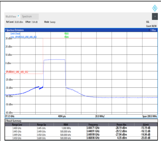
1-N78-3450-3550--30-30-L-6-CP-QPSK-Outer_Full-78@0-Ant1-1---see graph
