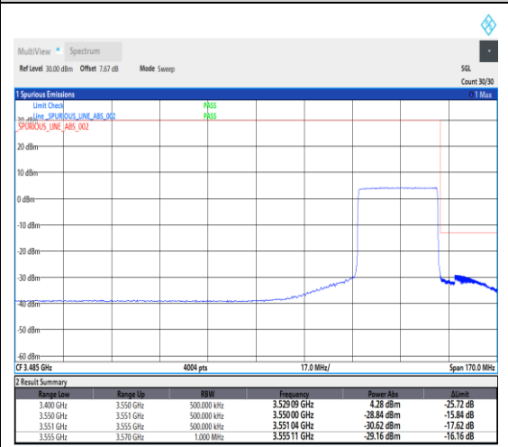
1-N78-3450-3550--30-30-H-6-CP-QPSK-Outer_Full-78@0-Ant1-1---see graph
