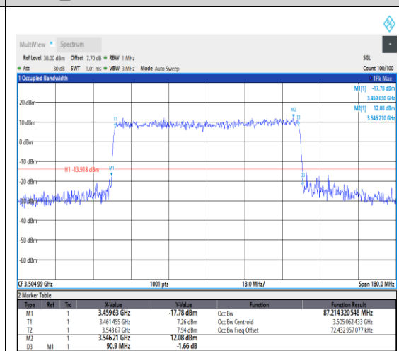
1-N78-3450-3550--30-90-H-6-CP-QPSK-Outer_Full-245@0-Ant1-87.214-90.900-≤90-
