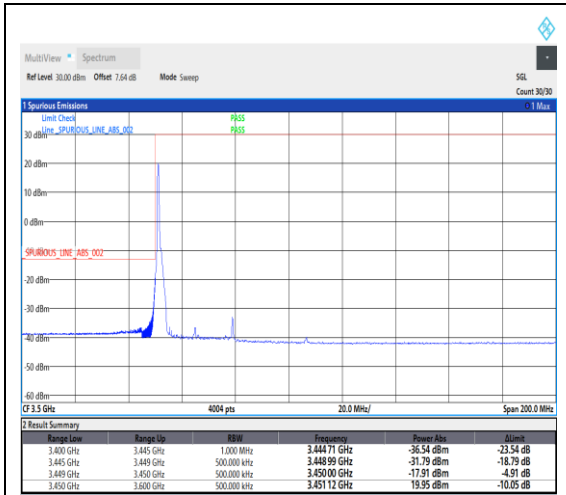
1-N78-3450-3550--30-30-L-4-CP-QPSK-Edge_1RB_Left-1@0-Ant1-1---see graph
