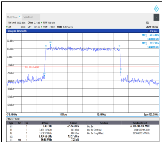
1-N78-3450-3550--30-60-L-1-DFT-QPSK-Out er_Full-162@0-Ant1-57.786-59.880-<=60-
