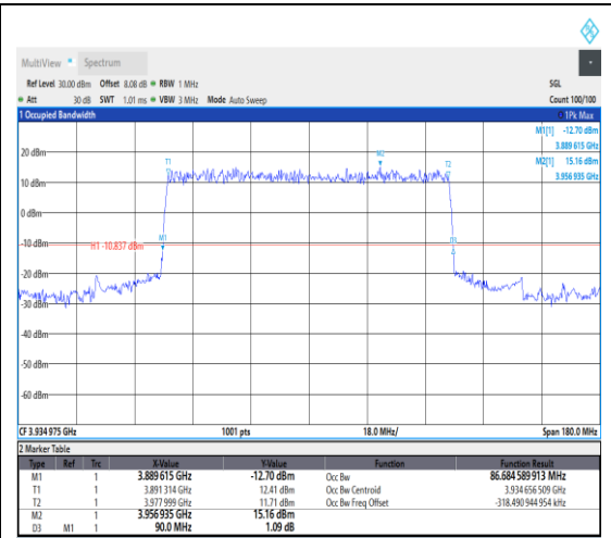
1-N77-3700-3980--30-90-H-2-DFT-PI2BPSK-Outer_Full-243@0-Ant1-86.685-90.000-<=90-PASS
