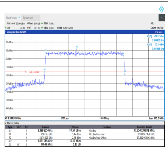
1-N77-3700-3980--30-80-H-9-CP-256QAM-Out_Full-217@0-Ant1-77.355-80.480-≤80-PA SS
