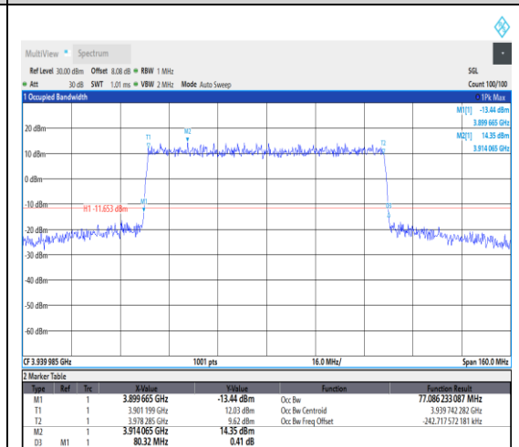
1-N77-3700-3980--30-80-H-3-DFT-16QAM-Outer_Full-216@0-Ant1-76.979-80.320-≤80-PA SS
