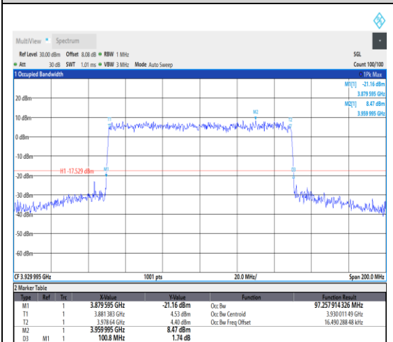
1-N77-3700-3980--30-100-H-9-CP-256QAM-
