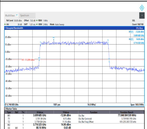
1-N77-3700-3980--30-80-L-1-DFT-QPSK-Out
