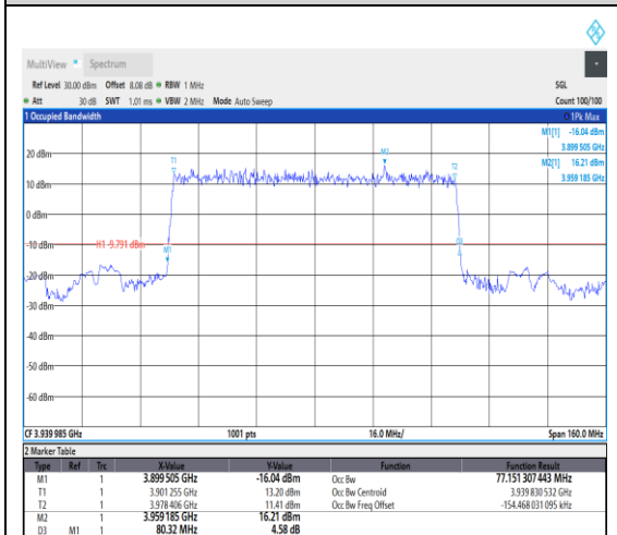
1-N77-3700-3980--30-80-H-2-DFT-PI2BPSK-Outer_Full-216@0-Ant1-76.979-80.320-≤80-PA SS
