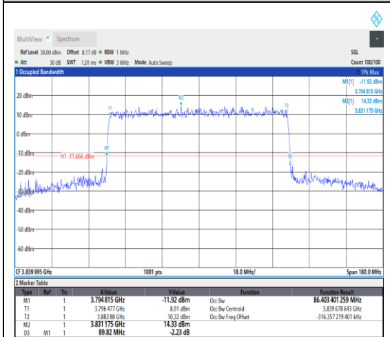
1-N77-3700-3980--30-90-M-4-DFT-64QAM-O
