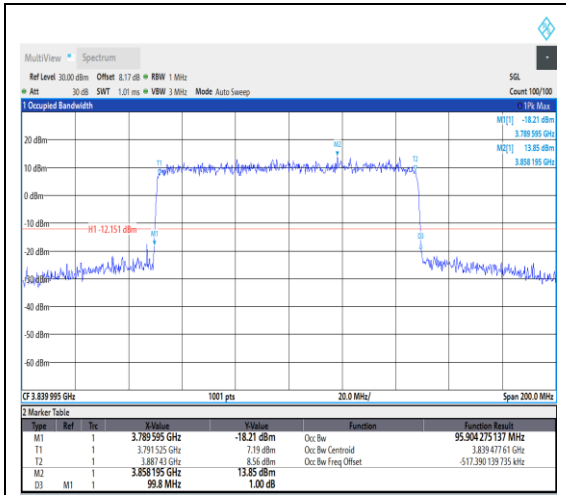
1-N77-3700-3980--30-100-M-3-DFT-16QAM-Outer_Full-270@0-Ant1-95.904-99.800-≤100 -PASS
