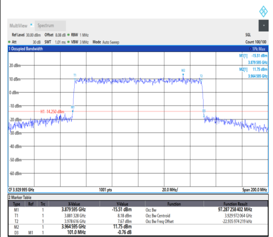
1-N77-3700-3980--30-100-H-7-CP-16QAM-Outer_Full-273@0-Ant1-97.287-101.000-≤100-PASS
