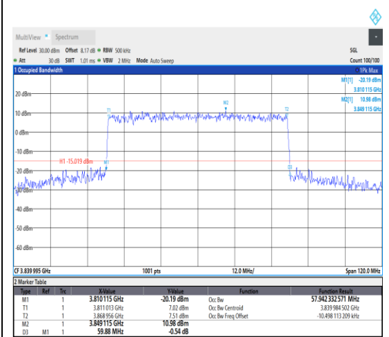
1-N77-3700-3980--30-60-M-7-CP-16QAM-Outer_Full-162@0-Ant1-57.942-59.880-≤60-PASS
