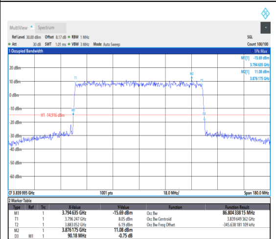
1-N77-3700-3980--30-90-M-5-DFT-256QAM-
