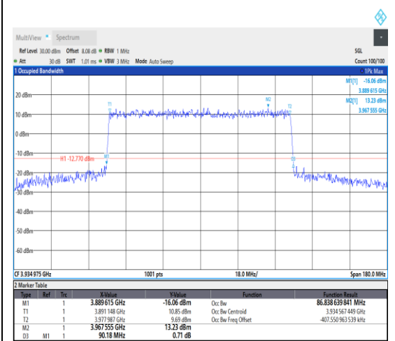
1-N77-3700-3980--30-90-H-3-DFT-16QAM-Outer_Full-243@0-Ant1-86.839-90.180-<=90-PA SS
