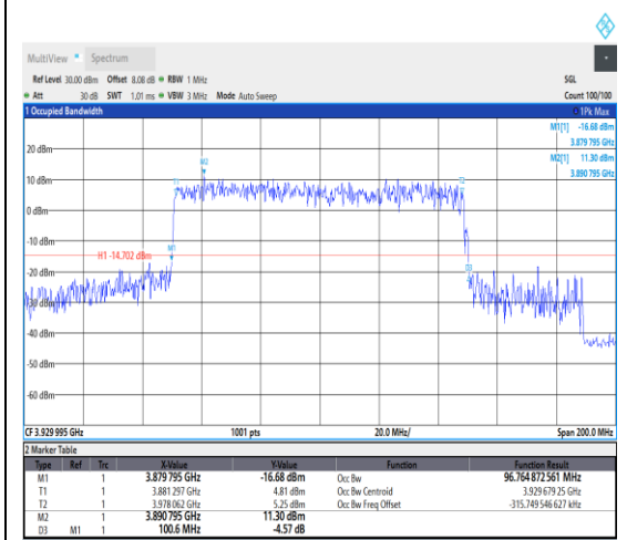
1-N77-3700-3980--30-100-H-6-CP-QPSK-Outer_Full-273@0-Ant1-96.765-100.600-≤100-PASS
