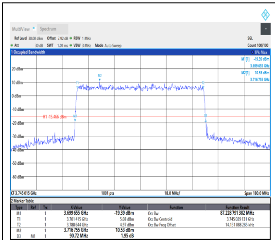
1-N77-3700-3980--30-90-L-9-CP-256QAM-Outer_Full-245@0-Ant1-87.229-90.720-≤90-PA SS
