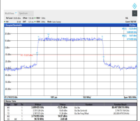
1-N77-3700-3980--30-90-L-2-DFT-PI2BPSK-Out_Full-243@0-Ant1-86.447-90.180-≤90-PASS PASS
