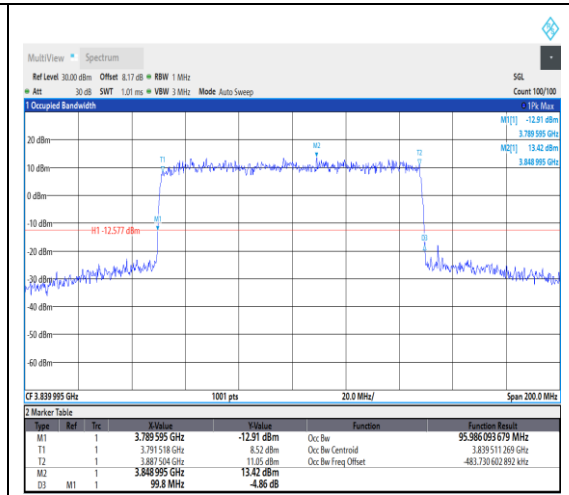
1-N77-3700-3980--30-100-M-4-DFT-64QAM-Outer_Full-270@0-Ant1-95.986-99.800-≤100 -PASS
