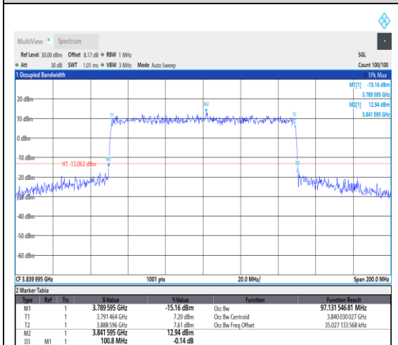
1-N77-3700-3980--30-100-M-7-CP-16QAM-Outer_Full-270@0-Ant1-97.161-100.800-≤100-P PASS
