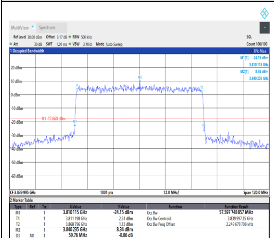
1-N77-3700-3980--30-60-M-9-CP-256QAM-Outer_Full-162@0-Ant1-57.732-59.880-≤60-PASS
