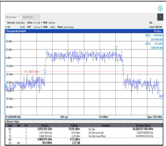
1-N77-3700-3980--30-60-M-6-CP-QPSK-Out er_Full-162@0-Ant1-56.829-59.400-≤60-PASS
