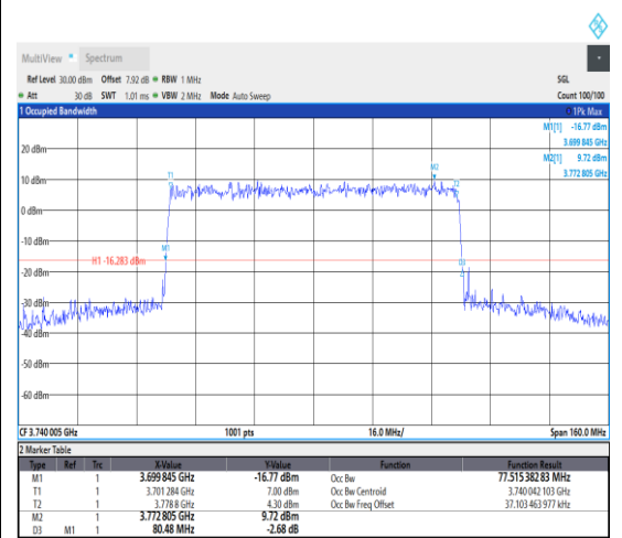
1-N77-3700-3980--30-80-L-9-CP-256QAM-Outer_Full-217@0-Ant1-77.515-80.480-≤80-PA SS
