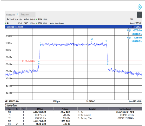
1-N77-3700-3980--30-90-H-5-DFT-256QAM-Outer_Full-243@0-Ant1-86.774-90.180-<=90-PA SS
