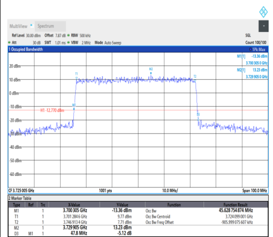
1-N77-3700-3980--30-50-L-4-DFT-64QAM-Outer_Full-128@0-Ant1-45.629-47.800-≤50-PASS
