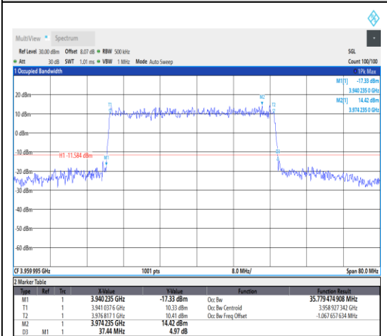
1-N77-3700-3980--30-40-H-4-DFT-64QAM-O
