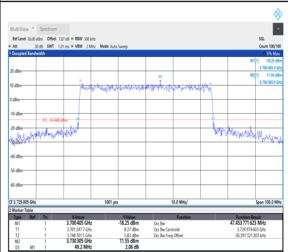
1-N77-3700-3980--30-50-L-6-CP-QPSK-Outer_Full-128@0-Ant1-45.716-47.600-≤50-PASS
