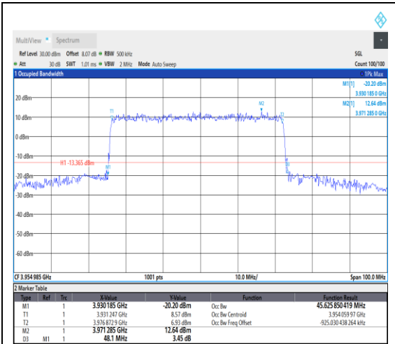
1-N77-3700-3980--30-50-H-3-DFT-16QAM-Outer_Full-128@0-Ant1-45.626-48.100-<=50-PA SS
