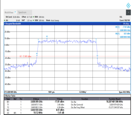
1-N77-3700-3980--30-20-M-9-CP-256QAM-Outer_Full-51@0-Ant1-18.207-19.120-<=20-PASS
