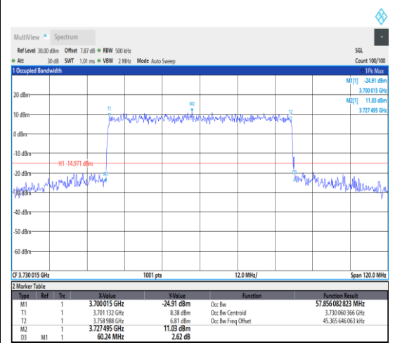
1-N77-3700-3980--30-60-L-7-CP-16QAM-Outer_Full-162@0-Ant1-57.856-60.240-≤60-PA SS
