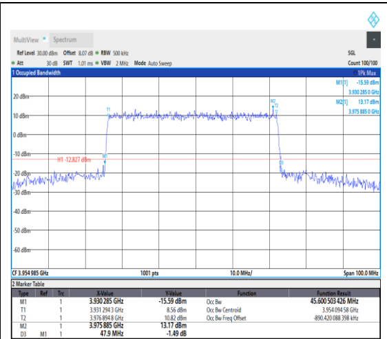
1-N77-3700-3980--30-50-H-4-DFT-64QAM-Outer_Full-128@0-Ant1-45.601-47.900-<=50-PA SS
