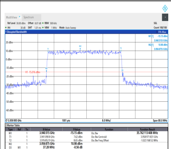
1-N77-3700-3980--30-40-H-5-DFT-256QAM-
