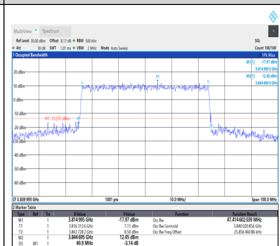
1-N77-3700-3980--30-50-M-7-CP-16QAM-O
