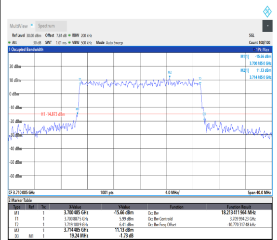
1-N77-3700-3980--30-20-L-8-CP-64QAM-Outer_Full-51@0-Ant1-18.213-19.240-≤20-PASS
