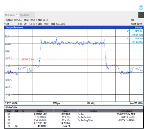
1-N77-3700-3980--30-50-L-2-DFT-PI2BPSK-Outer_Full-128@0-Ant1-45.535-48.000-≤50-PASS
