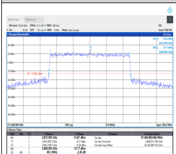
1-N77-3700-3980--30-50-M-6-CP-QPSK-Out
