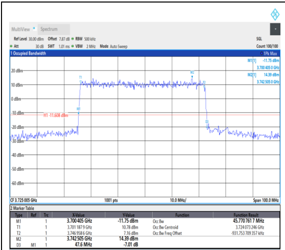
1-N77-3700-3980--30-50-L-1-DFT-QPSK-Out er_Full-128@0-Ant1-45.771-47.600-≤50-PASS
