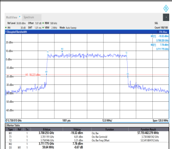
1-N77-3700-3980--30-60-L-9-CP-256QAM-Outer_Full-162@0-Ant1-57.755-60.240-≤60-PA SS
