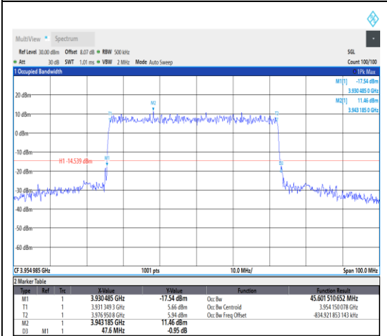
1-N77-3700-3980--30-50-H-5-DFT-256QAM-Outer_Full-128@0-Ant1-45.602-47.600-<=50-PASS
