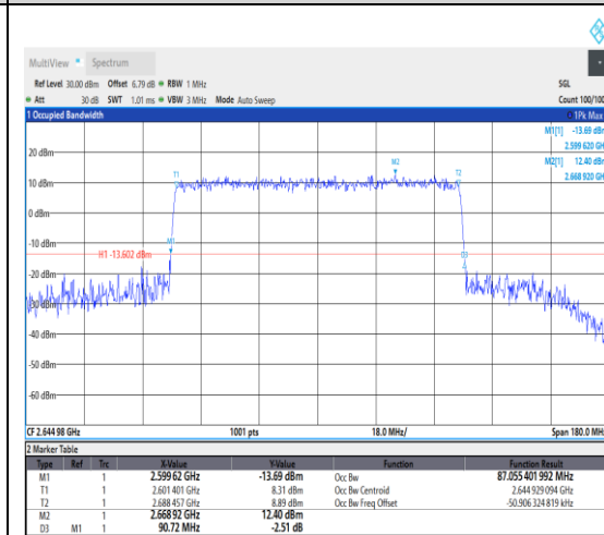
1-N41--30-90-H-6-CP-QPSK-Outer_Full-245@0-Ant1-87.055-90.720-<90-PASS
