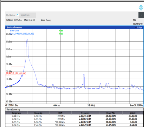
1-N41--30-50-L-1-DFT-PI2BPSK-Edge_1RB_Left-1@0-Ant1-1--PASS-see graph
