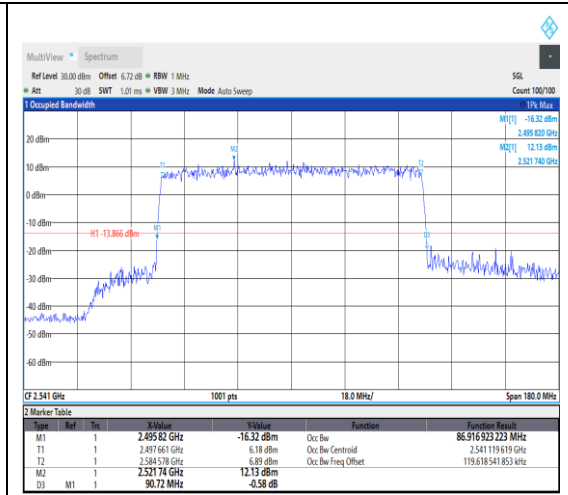
1-N41--30-90-L-8-CP-64QAM-Outer_Full-245 @0-Ant1-86.917-90.720-<=90-PASS
