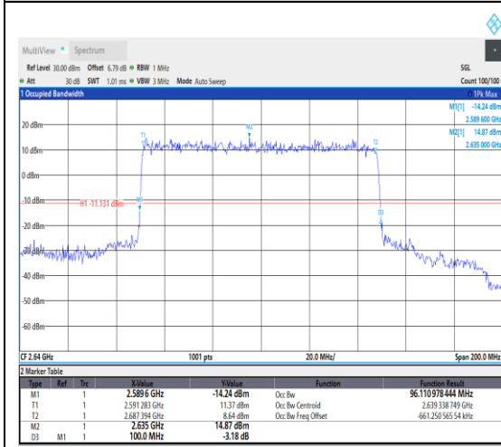
1-N41--30-100-H-2-DFT-PI2BPSK-Outer_Full-270@0-Ant1-96.111-100.000-≤100-PASS
