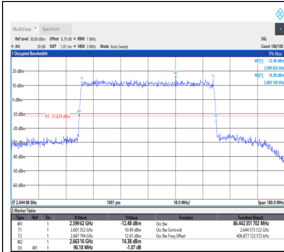
1-N41--30-90-H-1-DFT-QPSK-Outer_Full-24 3@0-Ant1-86.442-90.180-<90-PASS
