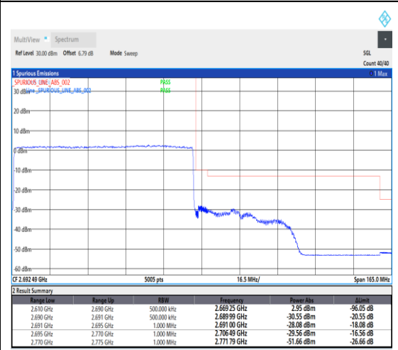
1-N41--30-80-H-3-DFT-PI2BPSK-Outer_Full-216@0-Ant1-1--PASS-see graph
