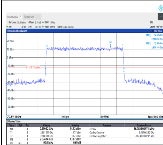
1-N41--30-90-H-3-DFT-16QAM-Outer_Full-243@0-Ant1-86.703-90.000-<90-PASS
