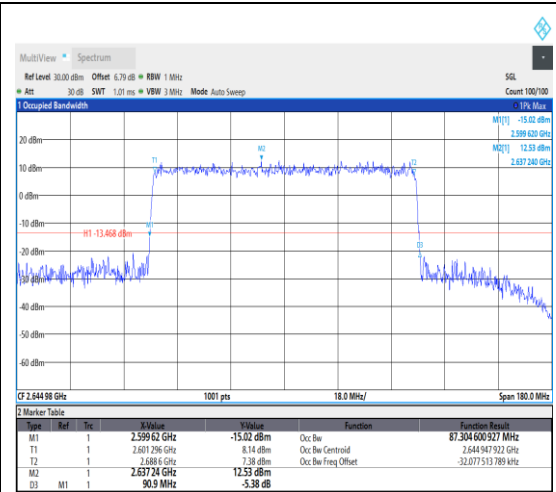
1-N41--30-90-H-8-CP-64QAM-Outer_Full-24 5@0-Ant1-87.305-90.900-≤90-PASS
