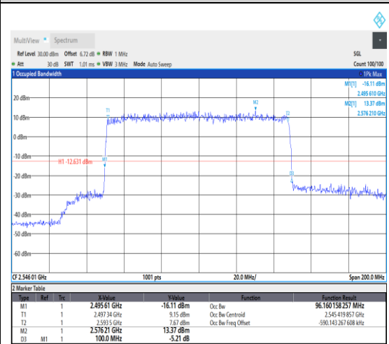
1-N41--30-100-L-3-DFT-16QAM-Outer_Full-270@0-Ant1-96.16-100.000-≤100-PASS
