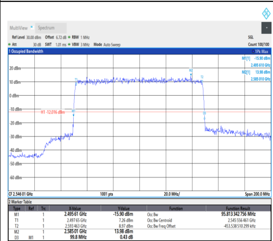
1-N41--30-100-L-1-DFT-QPSK-Outer_Full-27 0@0-Ant1-95.813-99.800-≤100-PASS
