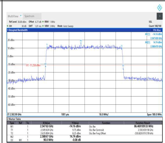
1-N41--30-90-M-1-DFT-QPSK-Outer_Full-243 @0-Ant1-86.47-90.000-<=90-PASS
