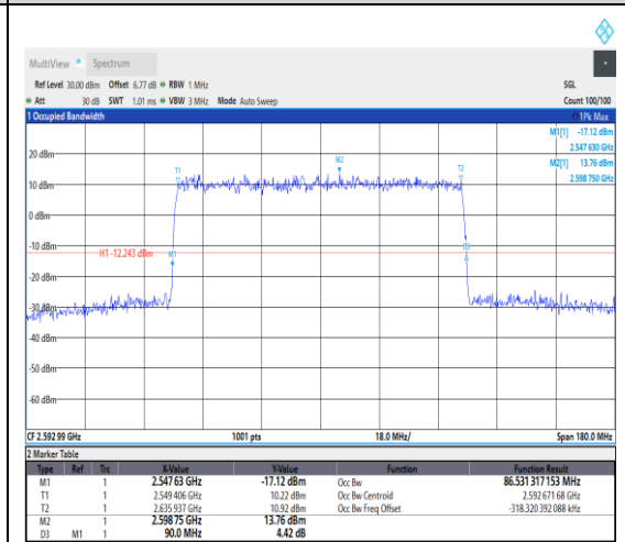
1-N41--30-90-M-3-DFT-16QAM-Outer_Full-243 @0-Ant1-86.531-90.000-<=90-PASS
