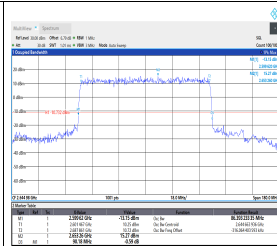
1-N41--30-90-H-2-DFT-PI2BPSK-Outer_Full-243@0-Ant1-86.393-90.180-<90-PASS
