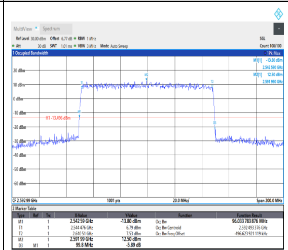
1-N41--30-100-M-4-DFT-64QAM-Outer_Full-270@0-Ant1-96.034-99.800-≤100-PASS
