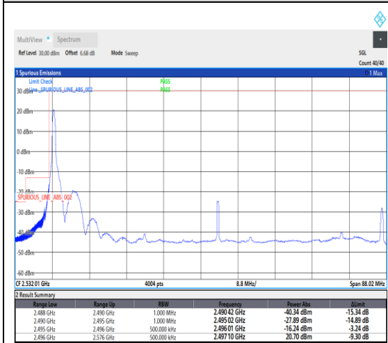
1-N41--30-80-L-4-CP-QPSK-Edge_1RB_Left-1@0-Ant1-1--PASS-see graph
