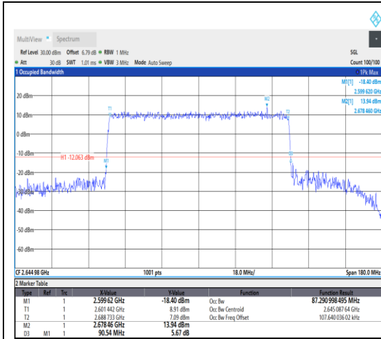
1-N41--30-90-H-7-CP-16QAM-Outer_Full-24 5@0-Ant1-87.291-90.540-≤90-PASS
