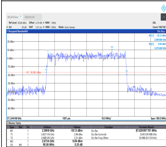
1-N41--30-90-H-9-CP-256QAM-Outer_Full-2 45@0-Ant1-87.029-90.360-≤90-PASS
