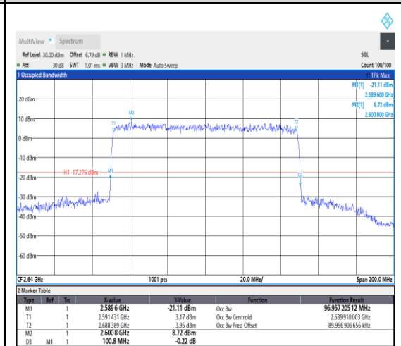
1-N41--30-100-H-9-CP-256QAM-Outer_Full-273@0-Ant1-96.957-100.800-≤100-PASS
