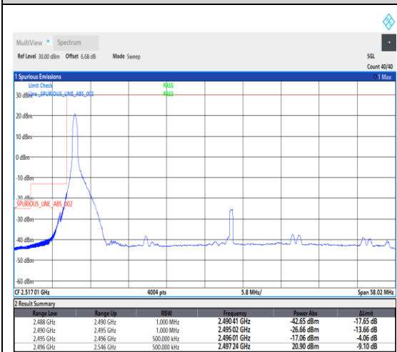
1-N41--30-50-L-4-CP-QPSK-Edge_1RB_Left-1@0-Ant1-1--PASS-see graph
