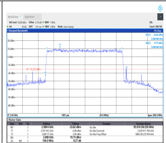
1-N41--30-100-H-5-DFT-256QAM-Outer_Full-270@0-Ant1-95.917-104.000-≤100-PASS
