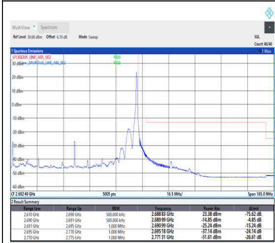
1-N41--30-80-H-2-DFT-PI2BPSK-Edge_1RB_Right-1@216-Ant1-1--PASS-see graph
