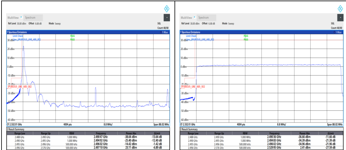
1-N41--30-80-L-1-DFT-PI2BPSK-Edge_1RB_Left-1@0-Ant1-1--PASS-see graph
