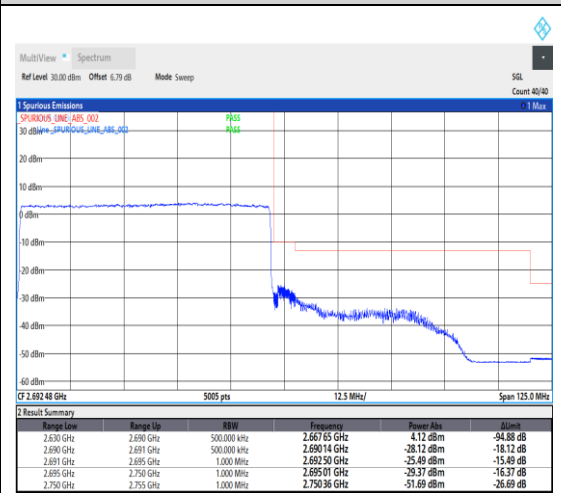
1-N41--30-60-H-3-DFT-PI2BPSK-Outer_Full-162@0-Ant1-1--PASS-see graph
