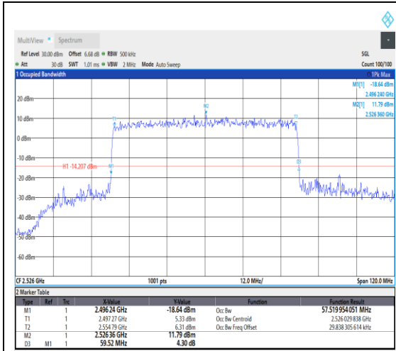
1-N41--30-60-L-7-CP-16QAM-Outer_Full-162 @0-Ant1-57.52-59.520-≤60-PASS
