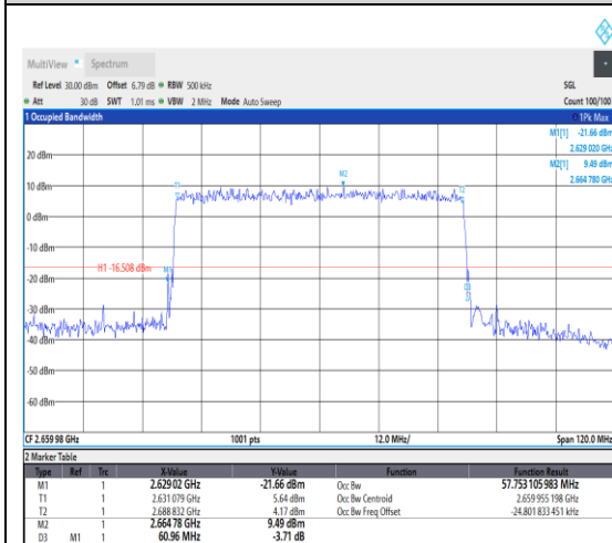
1-N41--30-60-H-5-DFT-256QAM-Outer_Full-162@0-Ant1-57.753-60.960-≤60-PASS
