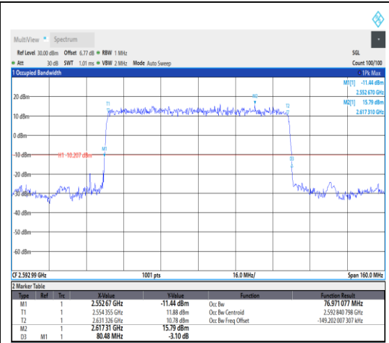
1-N41--30-80-M-2-DFT-PI2BPSK-Outer_Full-216@0-Ant1-76.971-80.480-≤80-PASS
