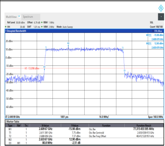
1-N41--30-80-H-7-CP-16QAM-Outer_Full-21 7@0-Ant1-77.315-80.800-≤80-PASS
