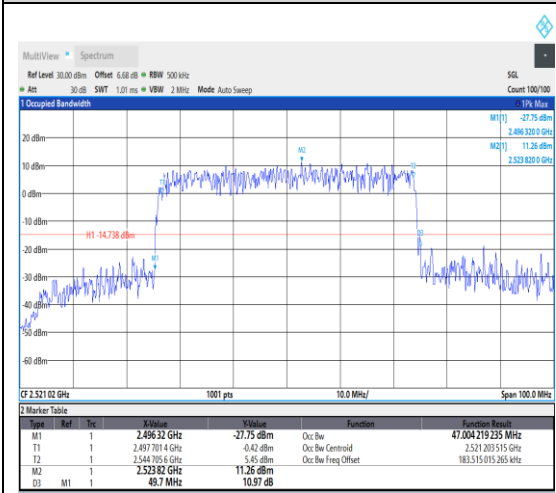
1-N41--30-50-L-6-CP-QPSK-Outer_Full-133 @0-Ant1-47.004-49.700-≤50-PASS
