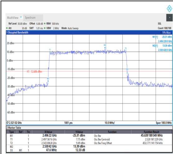
1-N41--30-50-L-4-DFT-64QAM-Outer_Full-12 8@0-Ant1-45.639-47.600-≤50-PASS
