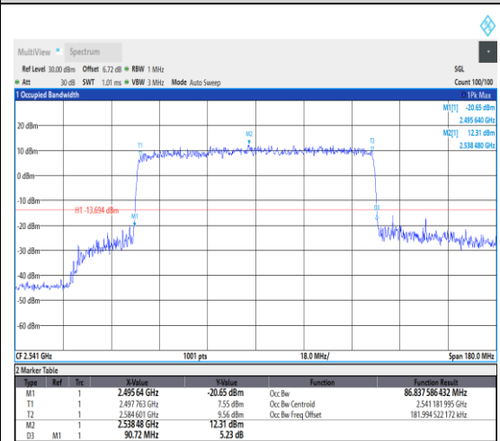
1-N41--30-90-L-6-CP-QPSK-Outer_Full-245 @0-Ant1-86.838-90.720-≤90-PASS
