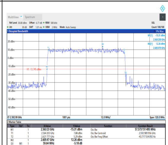
1-N41--30-60-M-3-DFT-16QAM-Outer_Full-1 62@0-Ant1-57.573-59.640-≤60-PASS
