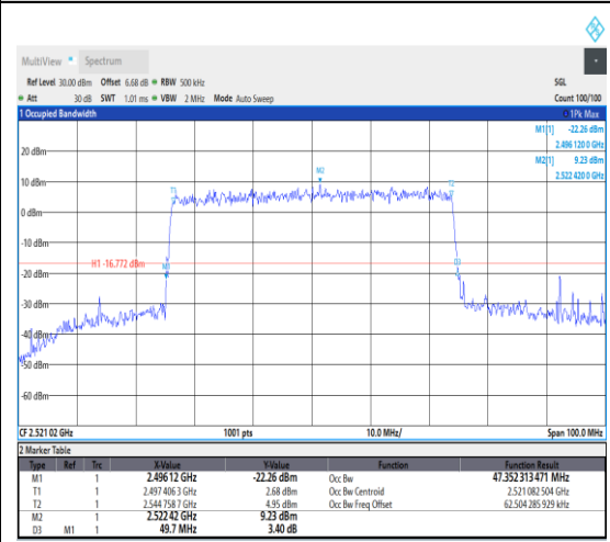
1-N41--30-50-L-9-CP-256QAM-Outer_Full-13 3@0-Ant1-47.352-49.700-≤50-PASS
