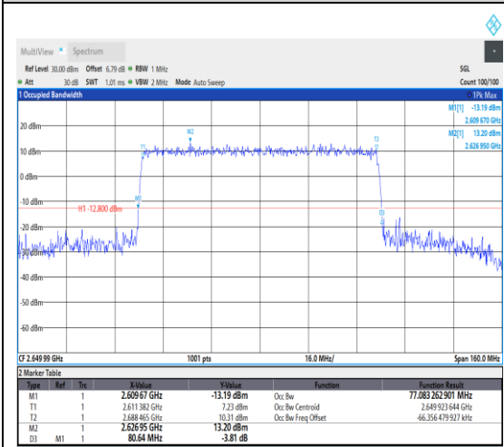
1-N41--30-80-H-6-CP-QPSK-Outer_Full-217 @0-Ant1-77.083-80.640-≤80-PASS
