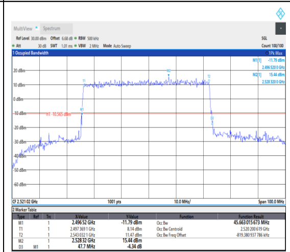
1-N41--30-50-L-1-DFT-QPSK-Outer_Full-128 @0-Ant1-45.663-47.700-≤50-PASS
