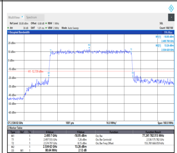
1-N41--30-80-L-7-CP-16QAM-Outer_Full-217 @0-Ant1-77.242-80.640-<80-PASS
