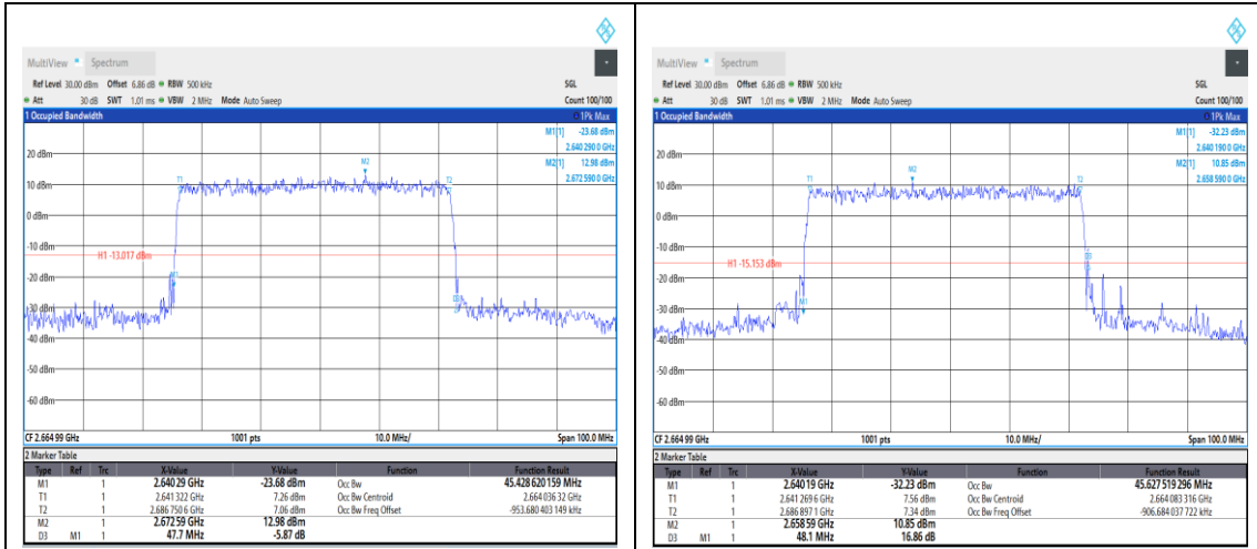
1-N41--30-50-H-4-DFT-64QAM-Outer_Full-1 28@0-Ant1-45.429-47.700-<math>\leq 50</math>-PASS 1-N41--30-50-H-5-DFT-256QAM-Outer_Full-128@0-Ant1-45.628-48.100-<math>\leq 50</math>-PASS
