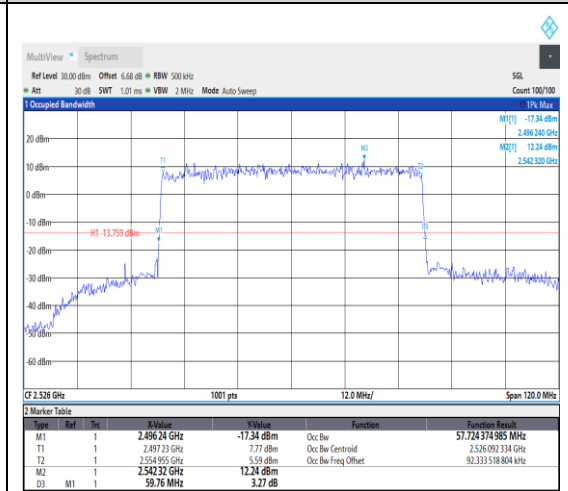
1-N41--30-60-L-4-DFT-64QAM-Outter_Full-16 2 @0-Ant1-57.724-59.760-≤60-PASS
