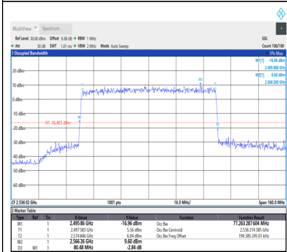
1-N41--30-80-L-6-CP-QPSK-Outer_Full-217 @0-Ant1-25.676-27.200-<80-PASS
