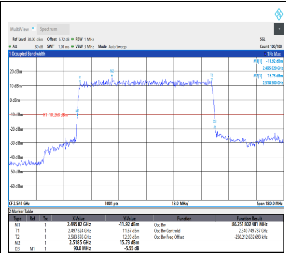
1-N41--30-90-L-2-DFT-PI2BPSK-Outer_Full-243 @0-Ant1-86.252-90.000-≤90-PASS
