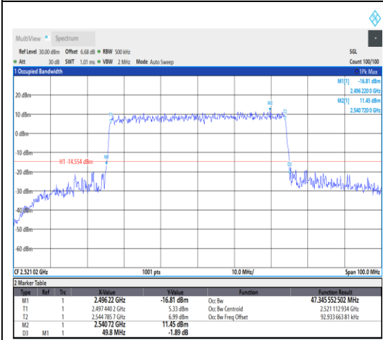
1-N41--30-50-L-8-CP-64QAM-Outer_Full-133 @0-Ant1-47.346-49.800-≤50-PASS
