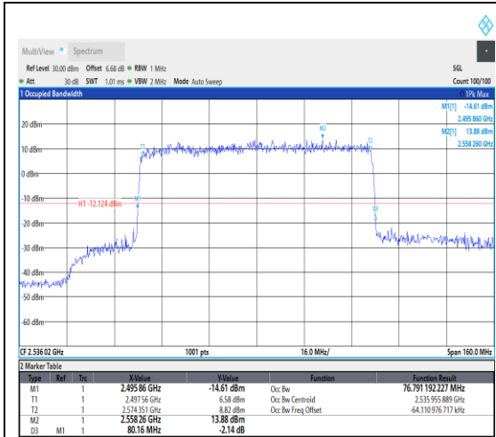
1-N41--30-80-L-4-DFT-64QAM-Outer_Full-21 6@0-Ant1-76.791-80.160-<80-PASS
