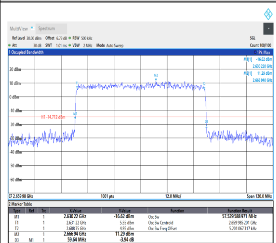
1-N41--30-60-H-6-CP-QPSK-Outer_Full-162@0-Ant1-57.53-59.640-≤60-PASS
