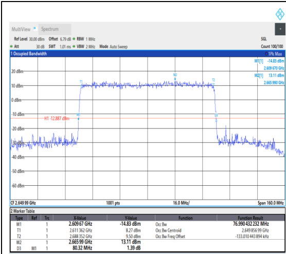
1-N41--30-80-H-4-DFT-64QAM-Outer_Full-2 16@0-Ant1-76.99-80.320-≤80-PASS
