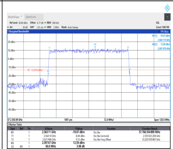
1-N41--30-60-M-1-DFT-QPSK-Outer_Full-16 2@0-Ant1-57.766-60.000-≤60-PASS
