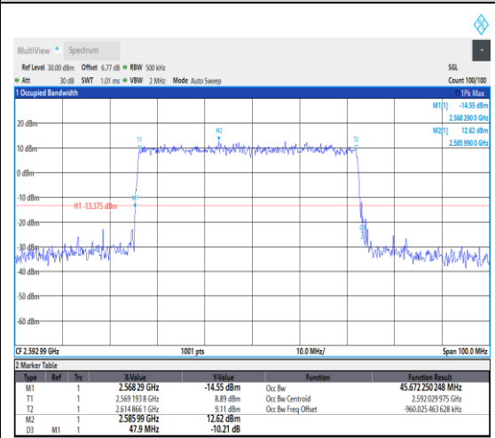
1-N41--30-50-M-4-DFT-64QAM-Outer_Full-1 28@0-Ant1-45.672-47.900-<=50-PASS
