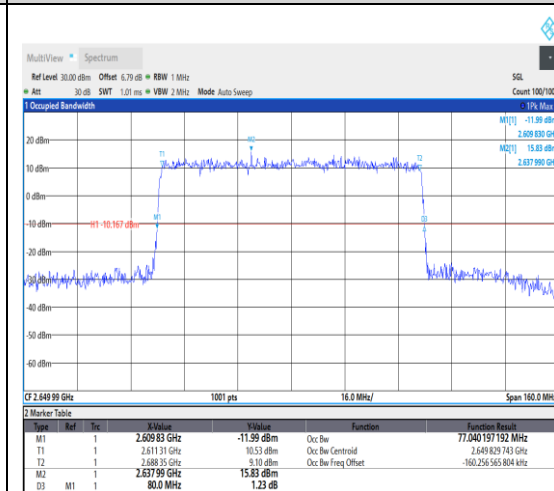
1-N41--30-80-H-3-DFT-16QAM-Outer_Full-2 16@0-Ant1-77.04-80.000-<80-PASS
