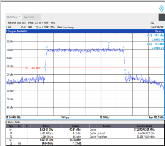
1-N41--30-80-H-8-CP-64QAM-Outer_Full-21 7@0-Ant1-77.294-80.640-≤80-PASS
