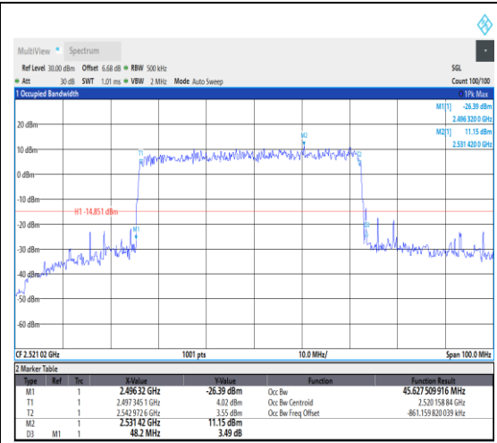
1-N41--30-50-L-5-DFT-256QAM-Outer_Full-1 28@0-Ant1-45.628-48.200-≤50-PASS
