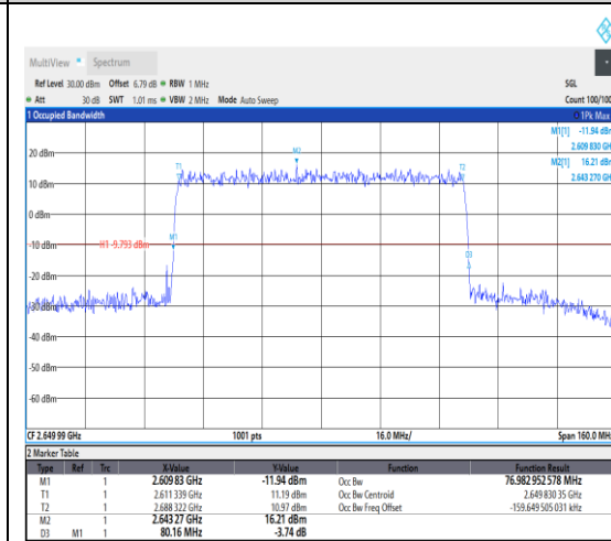
1-N41--30-80-H-1-DFT-QPSK-Outer_Full-21 6@0-Ant1-76.983-80.160-<80-PASS
