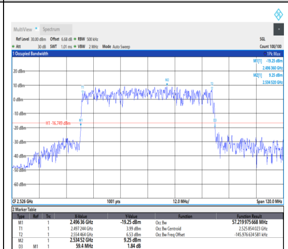
1-N41--30-60-L-6-CP-QPSK-Outter_Full-162 @0-Ant1-57.22-59.400-≤60-PASS
