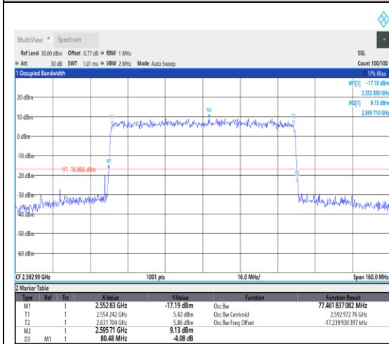
1-N41--30-80-M-9-CP-256QAM-Outer_Full-2 17@0-Ant1-77.462-80.480-<80-PASS
