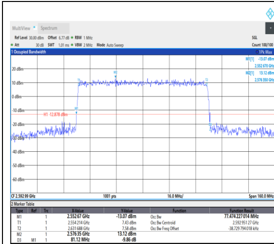
1-N41--30-80-M-7-CP-16QAM-Outer_Full-21 7@0-Ant1-77.474-81.120-<80-PASS
