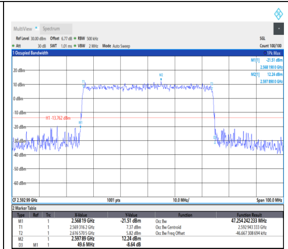
1-N41--30-50-M-8-CP-64QAM-Outer_Full-13 3@0-Ant1-47.254-49.600-≤50-PASS
