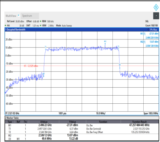
1-N41--30-50-L-7-CP-16QAM-Outer_Full-133 @0-Ant1-47.257-49.400-≤50-PASS
