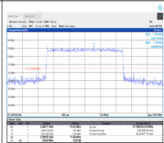
1-N41--30-60-M-7-CP-16QAM-Outer_Full-162@0-Ant1-57.789-59.640-<60-PASS
