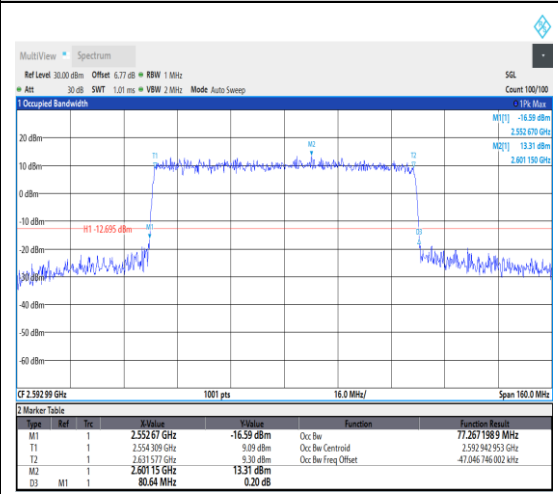
1-N41--30-80-M-6-CP-QPSK-Outer_Full-217 @0-Ant1-77.267-80.640-≤80-PASS
