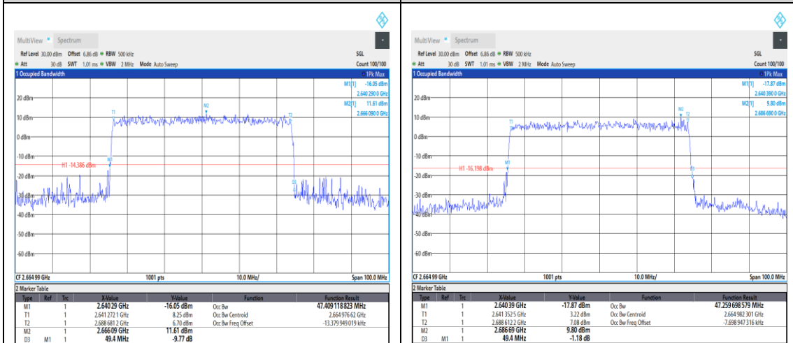
1-N41--30-50-H-8-CP-64QAM-Outer_Full-13 3@0-Ant1-47.409-49.400-<math>\leq 50</math>-PASS 1-N41--30-50-H-9-CP-256QAM-Outer_Full-1 33@0-Ant1-47.26-49.400-<math>\leq 50</math>-PASS
