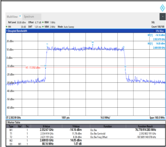
1-N41--30-80-M-3-DFT-16QAM-Outer_Full-2 16@0-Ant1-76.777-80.160-≤80-PASS
