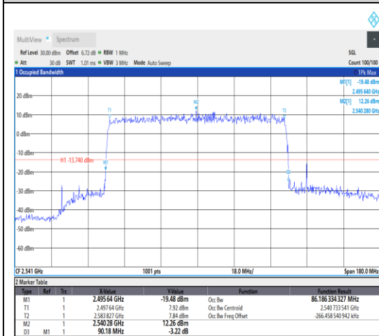
1-N41--30-90-L-5-DFT-256QAM-Outer_Full-243 @0-Ant1-86.186-90.180-≤90-PASS
