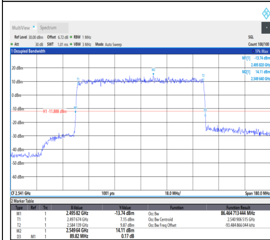
1-N41--30-90-L-3-DFT-16QAM-Outer_Full-243 @0-Ant1-86.465-89.820-≤90-PASS
