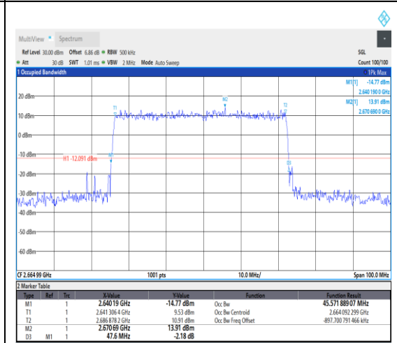
1-N41--30-50-H-3-DFT-16QAM-Outer_Full-1 28@0-Ant1-45.572-47.600-≤50-PASS
