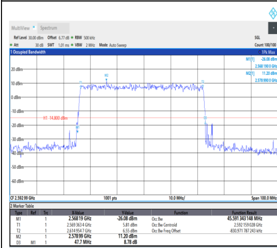
1-N41--30-50-M-5-DFT-256QAM-Outer_Full-1 128@0-Ant1-45.591-47.700-<=50-PASS
