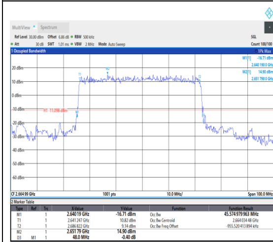
1-N41--30-50-H-2-DFT-PI2BPSK-Outer_Full-128 128@0-Ant1-45.575-48.000-≤50-PASS
