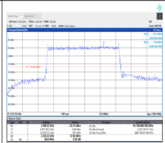
1-N41--30-50-L-3-DFT-16QAM-Outer_Full-12 8@0-Ant1-45.747-48.000-≤50-PASS
