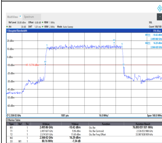
1-N41--30-80-L-2-DFT-PI2BPSK-Outer_Full-216 216@0-Ant1-76.893-80.160-≤80-PASS
