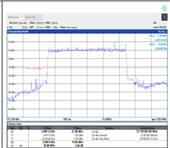
1-N41--30-60-L-2-DFT-PI2BPSK-Outter_Full-162 @0-Ant1-57.778-59.880-≤60-PASS
