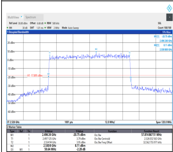
1-N41--30-60-L-9-CP-256QAM-Outer_Full-16 2@0-Ant1-57.815-59.640-≤60-PASS
