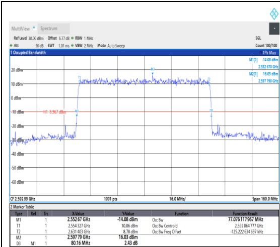
1-N41--30-80-M-1-DFT-QPSK-Outer_Full-21 6@0-Ant1-77.076-80.160-≤80-PASS
