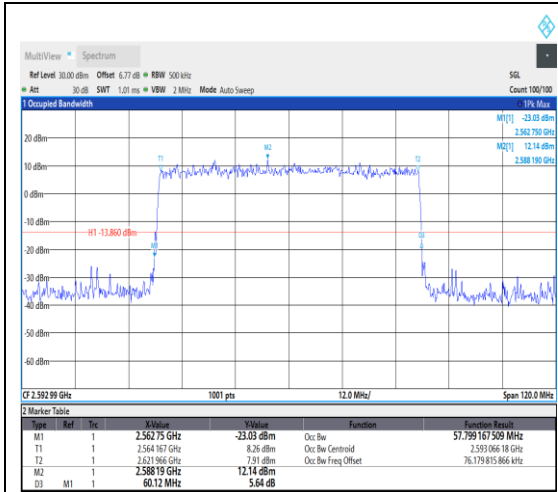
1-N41--30-60-M-4-DFT-64QAM-Outer_Full-1 62@0-Ant1-57.799-60.120-<60-PASS
