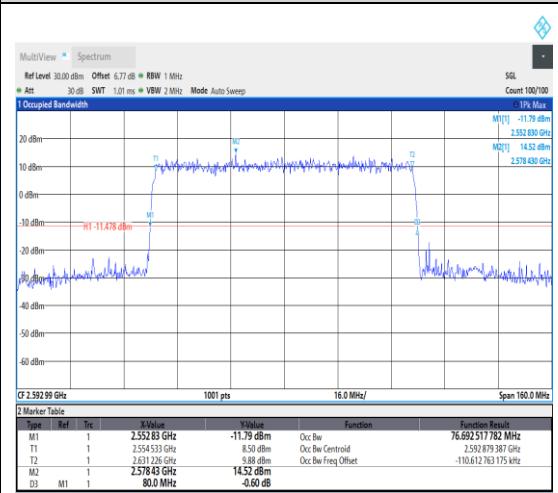
1-N41--30-80-M-4-DFT-64QAM-Outer_Full-2 16@0-Ant1-76.693-80.000-≤80-PASS
