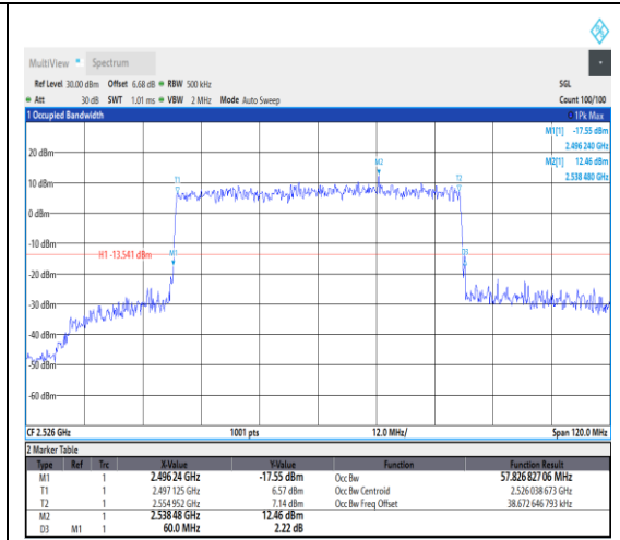
1-N41--30-60-L-8-CP-64QAM-Outer_Full-162 @0-Ant1-57.827-60.000-≤60-PASS
