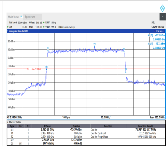
1-N41--30-80-L-5-DFT-256QAM-Outer_Full-2 16@0-Ant1-76.985-80.160-<80-PASS
