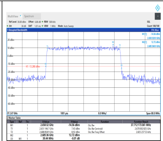
1-N41--30-40-H-8-CP-64QAM-Outer_Full-10 6@0-Ant1-37.712-39.440-≤40-PASS
