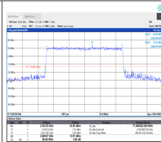
1-N41--30-80-M-8-CP-64QAM-Outer_Full-21 7@0-Ant1-77.361-80.960-<80-PASS
