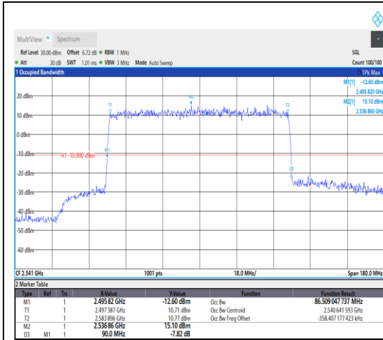
1-N41--30-90-L-1-DFT-QPSK-Outer_Full-243 @0-Ant1-86.509-90.000-≤90-PASS
