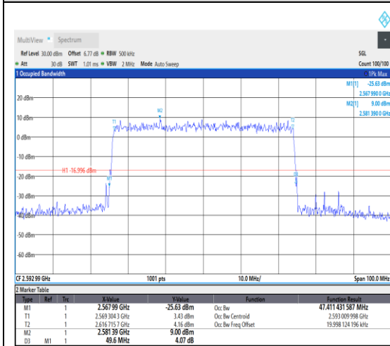
1-N41--30-50-M-9-CP-256QAM-Outer_Full-1 33@0-Ant1-47.411-49.600-≤50-PASS
