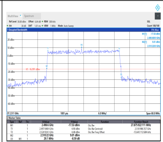
1-N41--30-30-L-9-CP-256QAM-Outer_Full-78 @0-Ant1-27.876-29.100-≤30-PASS
