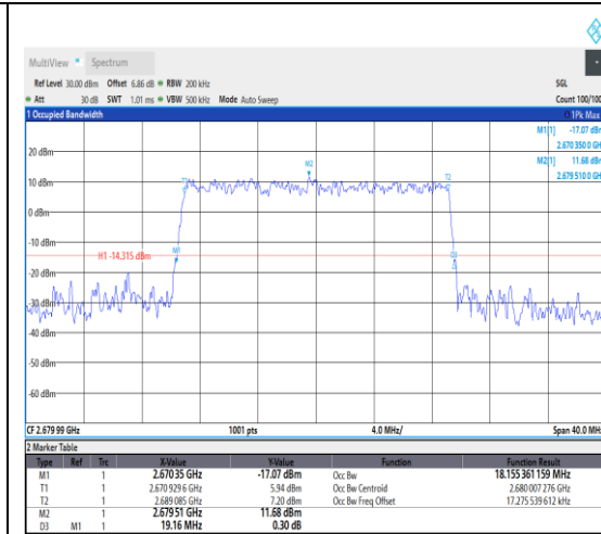
1-N41--30-20-H-8-CP-64QAM-Outer_Full-51 @0-Ant1-18.155-19.160-<20-PASS
