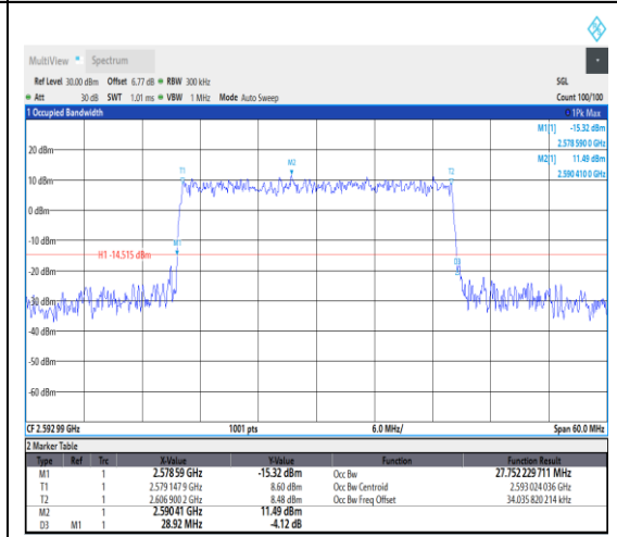
1-N41--30-30-M-6-CP-QPSK-Outer_Full-78 @0-Ant1-27.752-28.920-≤30-PASS
