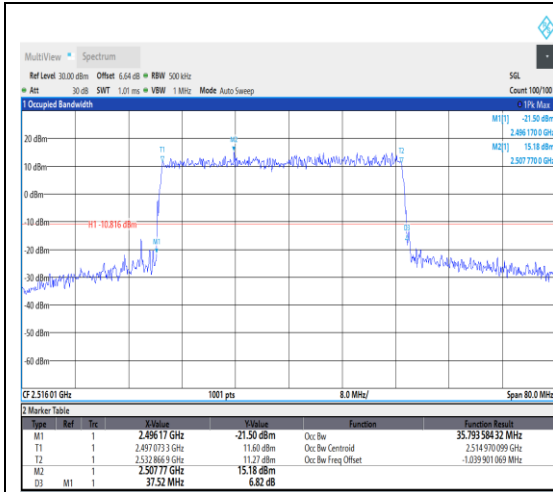
1-N41--30-40-L-1-DFT-QPSK-Outter_Full-100 @0-Ant1-35.794-37.520-<40-PASS
