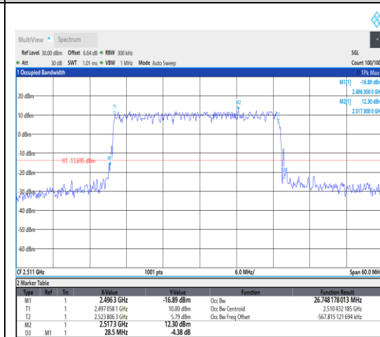
1-N41--30-30-L-3-DFT-16QAM-Outer_Full-75 @0-Ant1-26.748-28.500-<30-PASS
