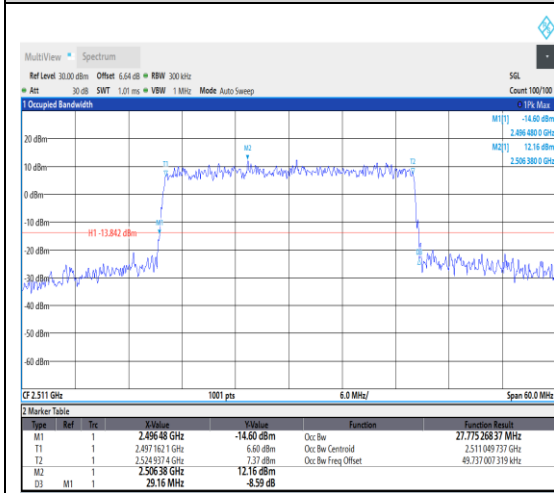
1-N41--30-30-L-6-CP-QPSK-Outer_Full-78 @0-Ant1-27.775-29.160-≤30-PASS
