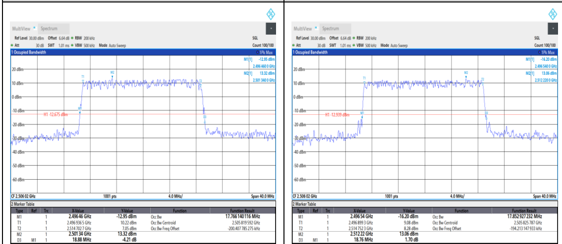
1-N41--30-20-L-3-DFT-16QAM-Outer_Full-50 @0-Ant1-17.766-18.880-≤20-PASS
