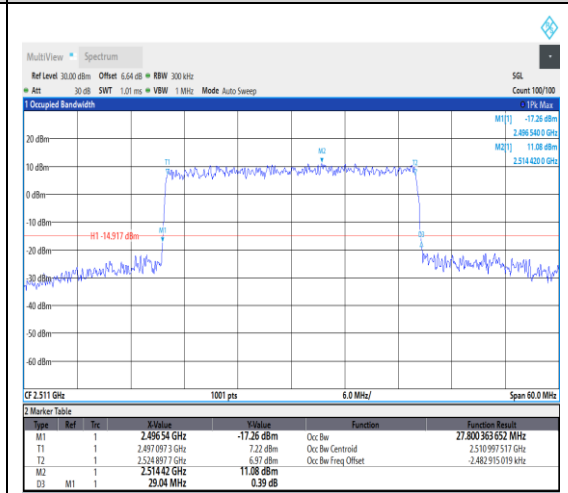
1-N41--30-30-L-7-CP-16QAM-Outer_Full-78 @0-Ant1-27.8-29.040-≤30-PASS
