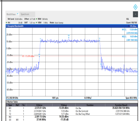
1-N41--30-40-M-3-DFT-16QAM-Outer_Full-100 @0-Ant1-35.823-37.440-<math>\leq 40</math>-PASS
