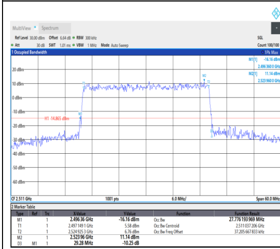
1-N41--30-30-L-8-CP-64QAM-Outer_Full-78 @0-Ant1-27.776-29.280-≤30-PASS
