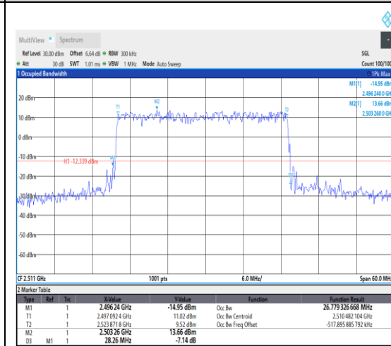
1-N41--30-30-L-1-DFT-QPSK-Outer_Full-75 @0-Ant1-26.779-28.260-<30-PASS
