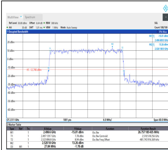
1-N41--30-30-L-4-DFT-64QAM-Outer_Full-75 @0-Ant1-26.757-27.840-≤30-PASS
