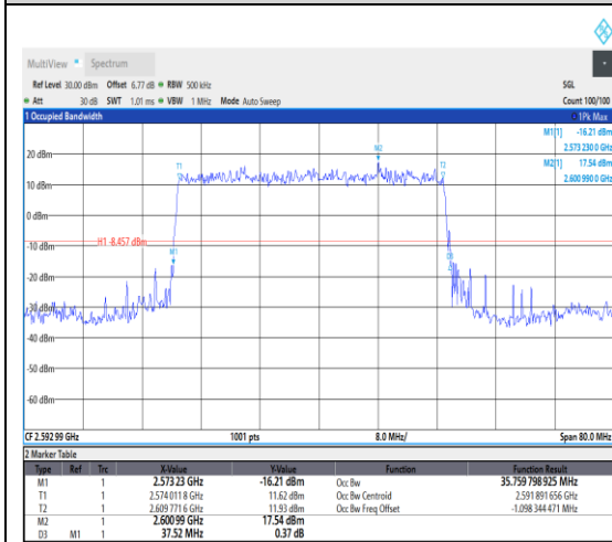
1-N41--30-40-M-2-DFT-PI2BPSK-Outer_Full-100 @0-Ant1-35.76-37.520-<math>\leq 40</math>-PASS
