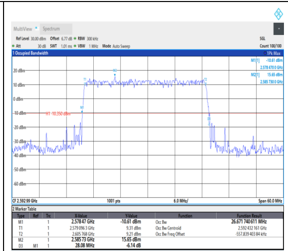
1-N41--30-30-M-2-DFT-PI2BPSK-Outer_Full-75 @0-Ant1-26.672-28.080-≤30-PASS
