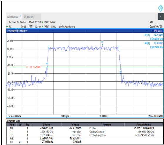
1-N41--30-30-M-1-DFT-QPSK-Outer_Full-75 @0-Ant1-26.689-27.960-≤30-PASS
