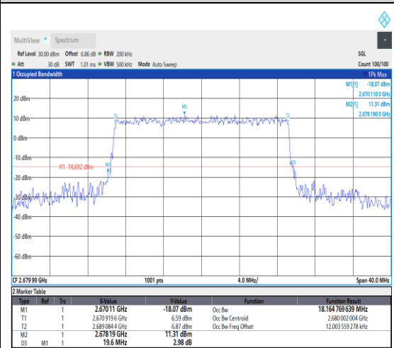
1-N41--30-20-H-6-CP-QPSK-Outer_Full-51 @0-Ant1-18.165-19.600-≤20-PASS
