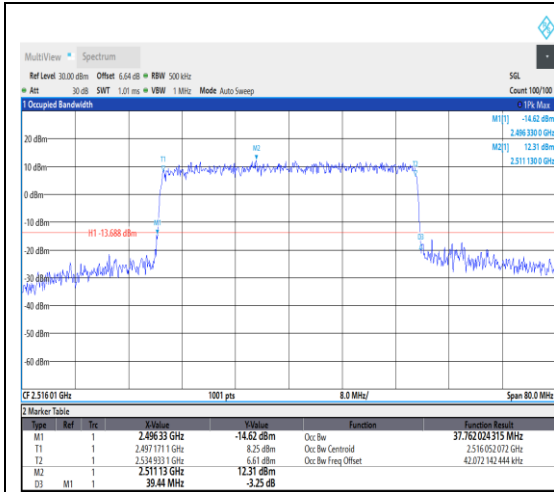
1-N41--30-40-L-7-CP-16QAM-Outer_Full-106 @0-Ant1-37.762-39.440-<math>\leq 40</math>-PASS
