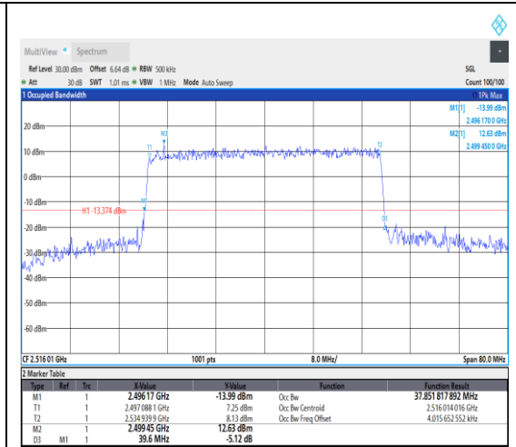
1-N41--30-40-L-8-CP-64QAM-Outer_Full-106 @0-Ant1-37.852-39.600-<math>\leq 40</math>-PASS
