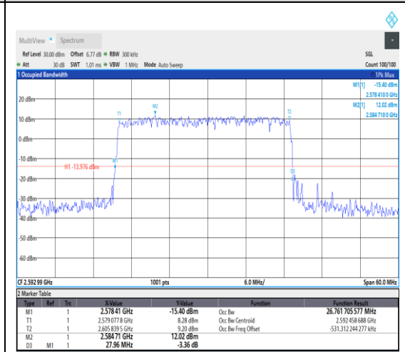
1-N41--30-30-M-4-DFT-64QAM-Outer_Full-75 @0-Ant1-26.762-27.960-≤30-PASS
