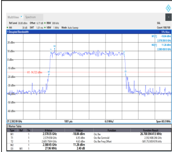
1-N41--30-30-M-5-DFT-256QAM-Outer_Full-75 @0-Ant1-26.7-27.960-≤30-PASS
