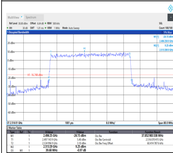
1-N41--30-40-L-9-CP-256QAM-Outer_Full-106 @0-Ant1-37.853-39.680-<math>\leq 40</math>-PASS
