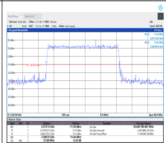
1-N41--30-40-M-1-DFT-QPSK-Outer_Full-106 @0-Ant1-35.646-37.680-<math>\leq 40</math>-PASS
