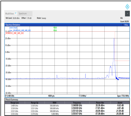
1-N78-3450-3550--30-80-H-5-CP-QPSK-Edge_1RB_Right-1@216-Ant1-1---see graph
