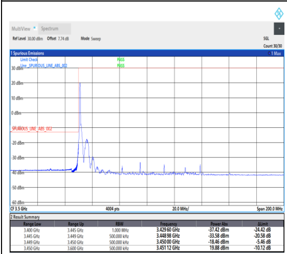
1-N78-3450-3550--30-90-L-1-DFT-PI2BPSK-Edge_1RB_Left-1@0-Ant1-1---see graph
