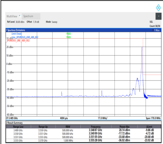
1-N78-3450-3550--30-90-H-5-CP-QPSK-Edge_1RB_Right-1@244-Ant1-1---see graph
