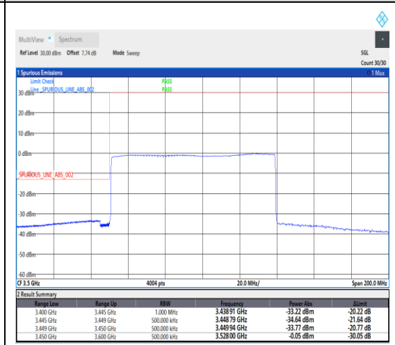
1-N78-3450-3550--30-90-L-6-CP-QPSK-Outer_Full-245@0-Ant1-1---see graph
