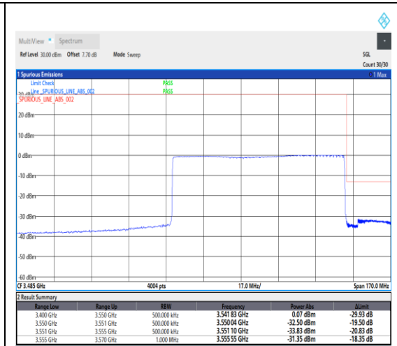
1-N78-3450-3550--30-80-H-6-CP-QPSK-Out_er_Full-217@0-Ant1-1---see graph
