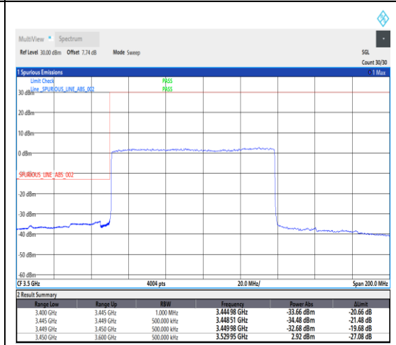
1-N78-3450-3550--30-90-L-3-DFT-PI2BPSK-Outer_Full-243@0-Ant1-1---see graph
