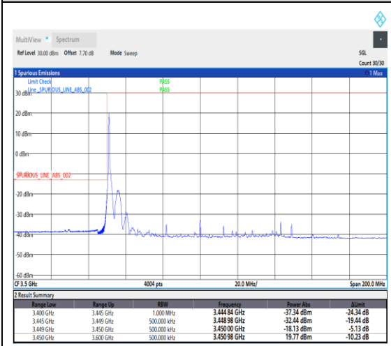
1-N78-3450-3550--30-100-L-1-DFT-PI2BPSK-Edge_1RB_Left-1@0-Ant1-1---see graph
