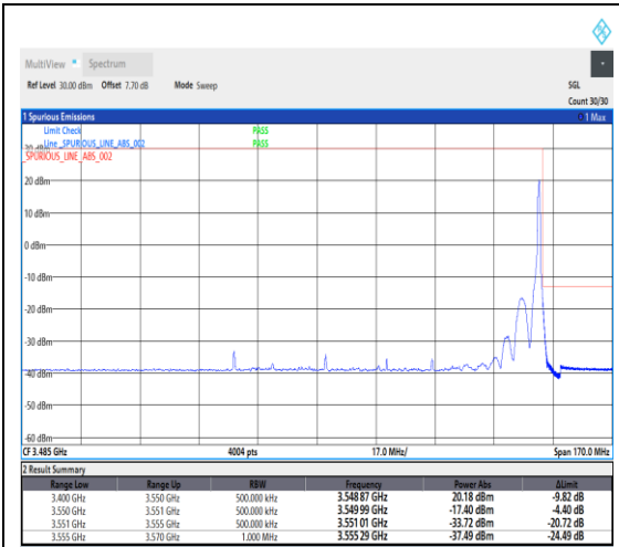
1-N78-3450-3550--30-90-H-2-DFT-PI2BPSK-Edge_1RB_Right-1@244-Ant1-1---see graph
