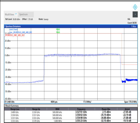
1-N78-3450-3550--30-100-L-6-CP-QPSK-Out_er_Full-273@0-Ant1-1---see graph
