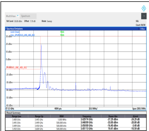
1-N78-3450-3550--30-100-L-4-CP-QPSK-Edge_1RB_Left-1@0-Ant1-1---see graph
