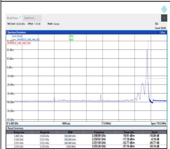
1-N78-3450-3550--30-100-H-5-CP-QPSK-Edge_1RB_Right-1@272-Ant1-1---see graph
