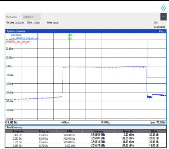
1-N78-3450-3550--30-90-H-6-CP-QPSK-Outer_Full-245@0-Ant1-1---see graph
