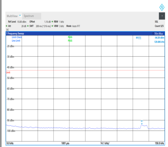
1-N78-3450-3550--30-100-M-1-DFT-PI2BPS K-Inner_1RB_Left-1@1-0.009-0.15-Ant1-0.1 3--94.39--43-
