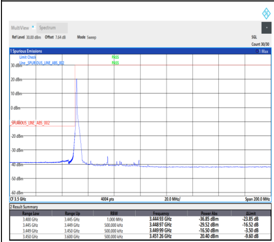
1-N78-3450-3550--30-50-L-1-DFT-PI2BPSK-Edge_1RB_Left-1@0-Ant1-1---see graph
