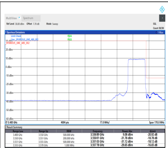
1-N78-3450-3550--30-20-H-3-DFT-PI2BPSK-Outer_Full-50@0-Ant1-1---see graph
