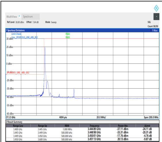
1-N78-3450-3550--30-40-L-1-DFT-PI2BPSK-Edge_1RB_Left-1@0-Ant1-1---see graph
