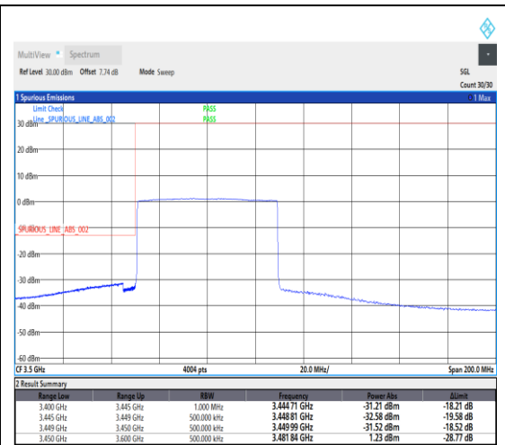
1-N78-3450-3550--30-60-L-6-CP-QPSK-Outer_Full-162@0-Ant1-1---see graph
