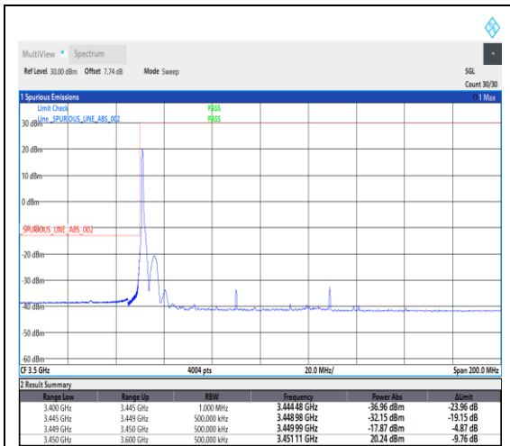
1-N78-3450-3550--30-80-L-1-DFT-PI2BPSK-Edge_1RB_Left-1@0-Ant1-1---see graph
