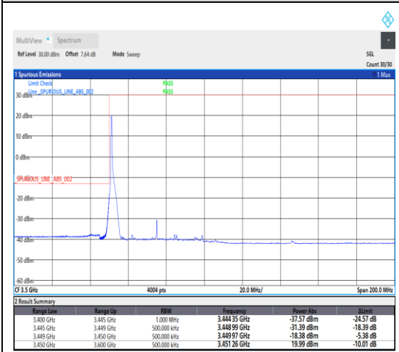
1-N78-3450-3550--30-50-L-4-CP-QPSK-Edge_1RB_Left-1@0-Ant1-1---see graph
