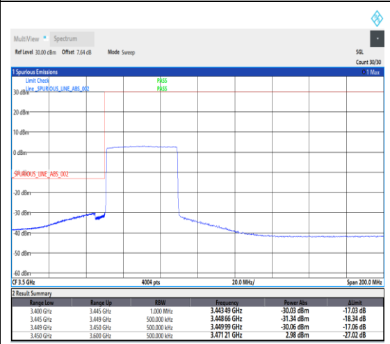
1-N78-3450-3550--30-40-L-6-CP-QPSK-Outer_Full-106@0-Ant1-1---see graph
