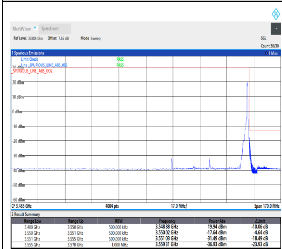
1-N78-3450-3550--30-50-H-5-CP-QPSK-Edge_1RB_Right-1@132-Ant1-1---see graph
