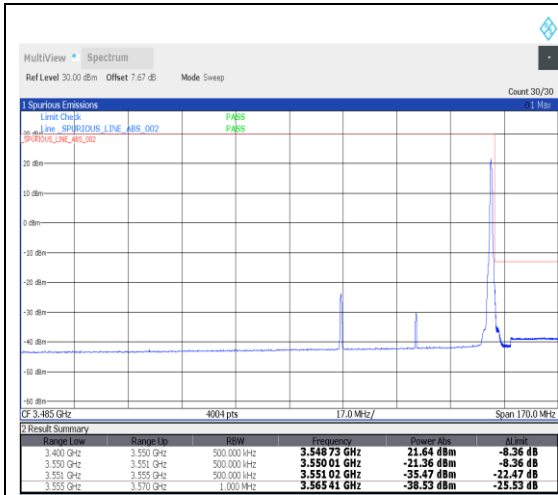
1-N78-3450-3550--30-50-H-2-DFT-PI2BPSK-Edge_1RB_Right-1@132-Ant1-1---see graph
