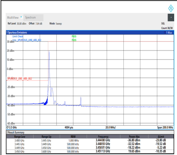
1-N78-3450-3550--30-40-L-4-CP-QPSK-Edge_1RB_Left-1@0-Ant1-1---see graph
