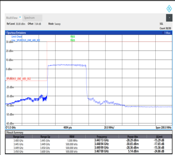
1-N78-3450-3550--30-50-L-3-DFT-PI2BPSK-Outer_Full-128@0-Ant1-1---see graph
