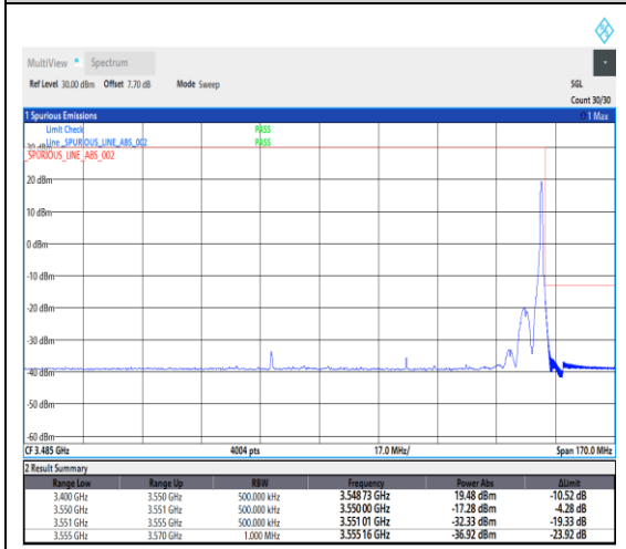
1-N78-3450-3550--30-80-H-2-DFT-PI2BPSK-Edge_1RB_Right-1@216-Ant1-1---see graph
