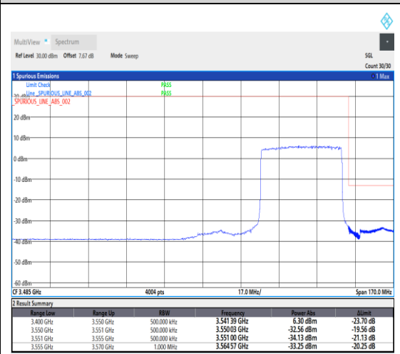
1-N78-3450-3550--30-40-H-3-DFT-PI2BPSK-Outer_Full-100@0-Ant1-1---see graph
