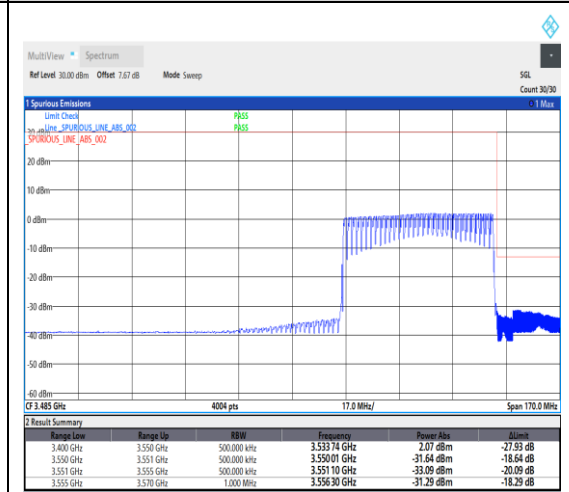
1-N78-3450-3550--30-50-H-6-CP-QPSK-Outer_Full-133@0-Ant1-1---see graph
