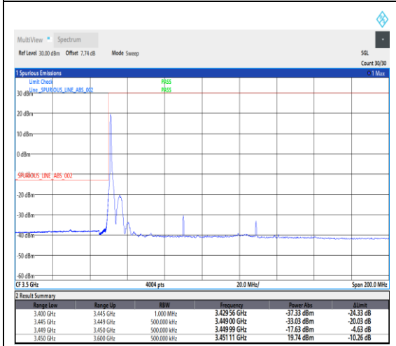
1-N78-3450-3550--30-80-L-4-CP-QPSK-Edge_1RB_Left-1@0-Ant1-1---see graph
