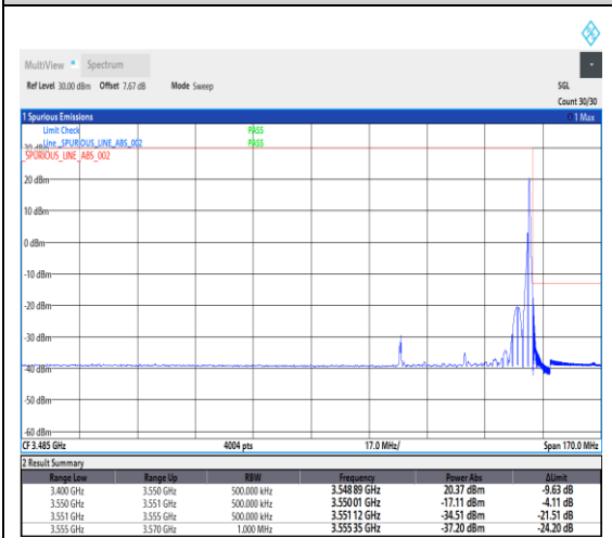
1-N78-3450-3550--30-40-H-2-DFT-PI2BPSK-Edge_1RB_Right-1@105-Ant1-1---see graph
