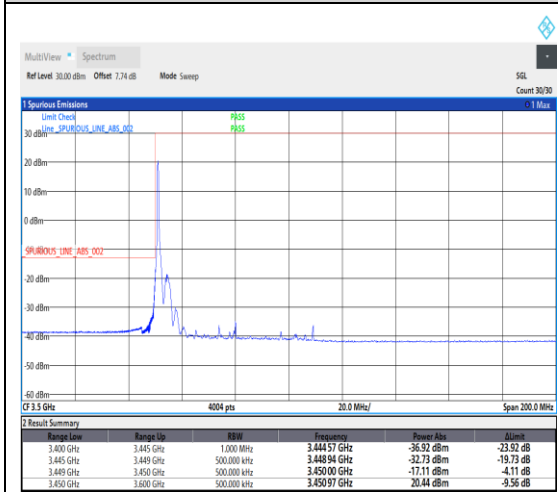
1-N78-3450-3550--30-60-L-1-DFT-PI2BPSK-Edge_1RB_Left-1@0-Ant1-1---see graph
