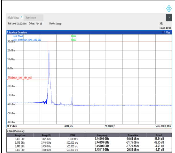
1-N78-3450-3550--30-30-L-1-DFT-PI2BPSK-Edge_1RB_Left-1@0-Ant1-1---see graph
