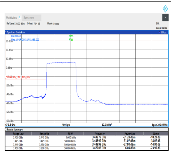
1-N78-3450-3550--30-40-L-3-DFT-PI2BPSK-Outer_Full-100@0-Ant1-1---see graph
