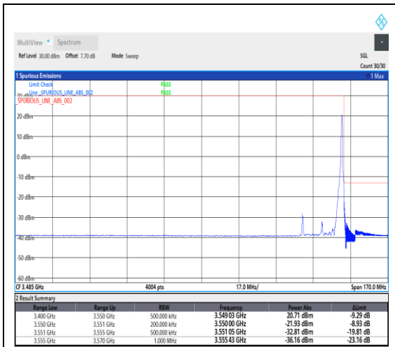
1-N78-3450-3550--30-20-H-2-DFT-PI2BPSK-Edge_1RB_Right-1@50-Ant1-1---see graph
