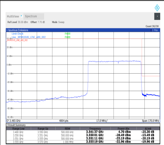
1-N78-3450-3550--30-60-H-3-DFT-PI2BPSK-Outer_Full-162@0-Ant1-1---see graph
