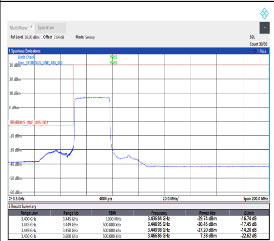
1-N78-3450-3550--30-30-L-3-DFT-PI2BPSK-Outer_Full-75@0-Ant1-1---see graph
