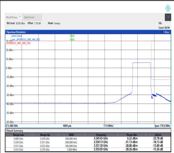
1-N78-3450-3550--30-20-H-6-CP-QPSK-Outer_Full-51@0-Ant1-1---see graph
