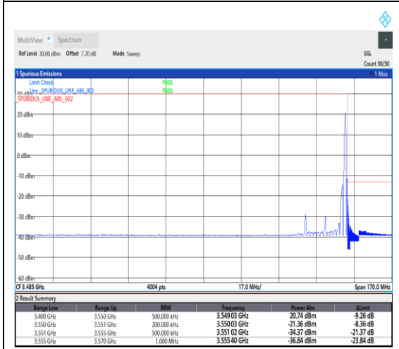
1-N78-3450-3550--30-20-H-5-CP-QPSK-Edge_1RB_Right-1@50-Ant1-1---see graph
