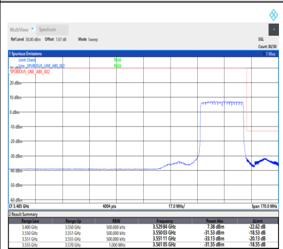
1-N78-3450-3550--30-30-H-3-DFT-PI2BPSK-Outer_Full-75@0-Ant1-1---see graph
