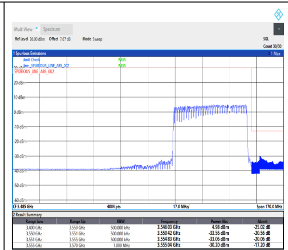
1-N78-3450-3550--30-50-H-3-DFT-PI2BPSK-Outer_Full-128@0-Ant1-1---see graph
