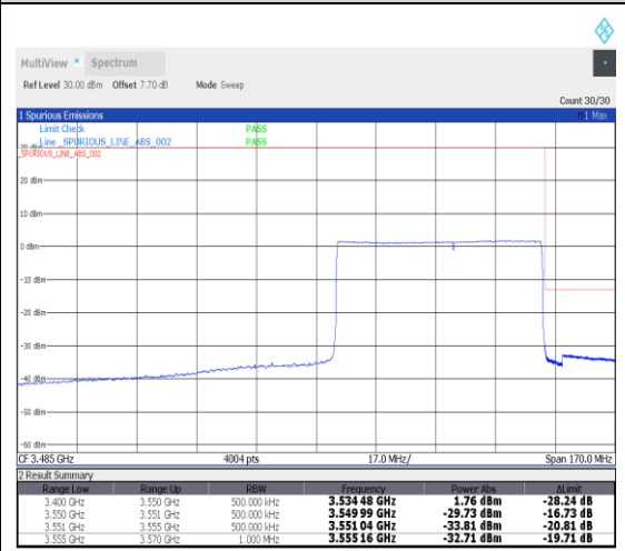
1-N78-3450-3550--30-60-H-6-CP-QPSK-Outer_Full-162@0-Ant1-1---see graph
