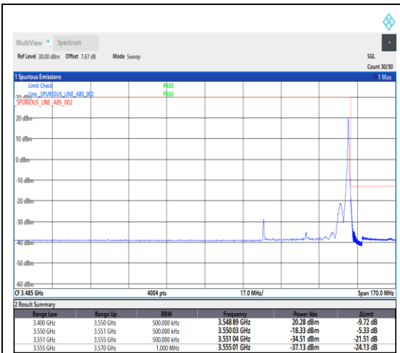
1-N78-3450-3550--30-40-H-5-CP-QPSK-Edge_1RB_Right-1@105-Ant1-1---see graph
