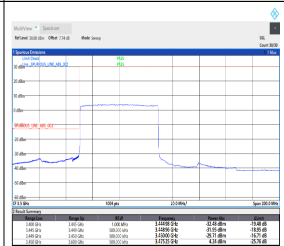
1-N78-3450-3550--30-60-L-3-DFT-PI2BPSK-Outer_Full-162@0-Ant1-1---see graph
