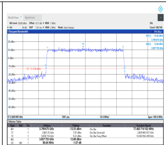
1-N77-3700-3980--30-80-M-8-CP-64QAM-Outer_Full-217@0-Ant1-77.464-80.640-≤80-PA SS
