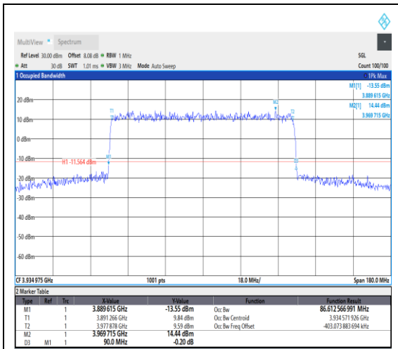
1-N77-3700-3980--30-90-H-1-DFT-QPSK-Outer_Full-243@0-Ant1-86.613-90.000-<=90-PA SS
