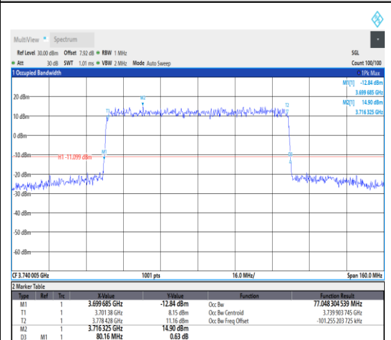
1-N77-3700-3980--30-80-L-1-DFT-QPSK-Out
