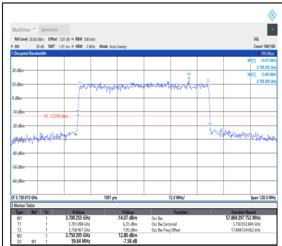
1-N77-3700-3980--30-60-L-4-DFT-64QAM-Outer_Full-162@0-Ant1-57.869-59.640-≤60-PA SS
