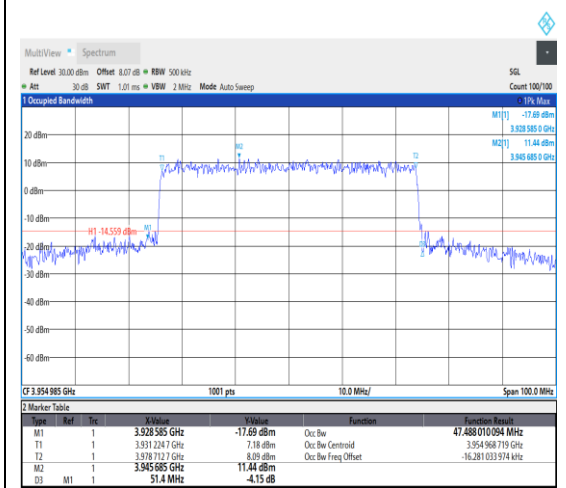
1-N77-3700-3980--30-50-H-7-CP-16QAM-Ou
