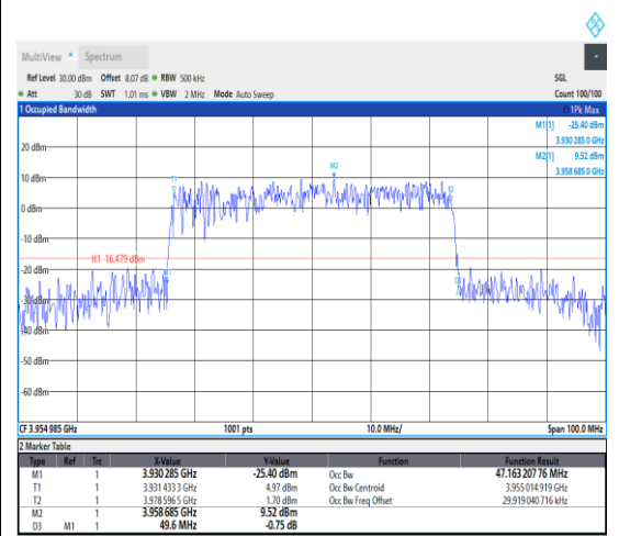
1-N77-3700-3980--30-50-H-8-CP-64QAM-Ou
