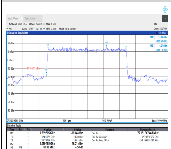
1-N77-3700-3980--30-80-H-2-DFT-PI2BPSK-
