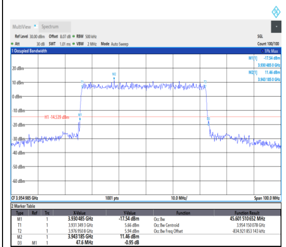
1-N77-3700-3980--30-50-H-5-DFT-256QAM-Outter_Full-128@0-Ant1-45.602-47.600-<=50-PASS
