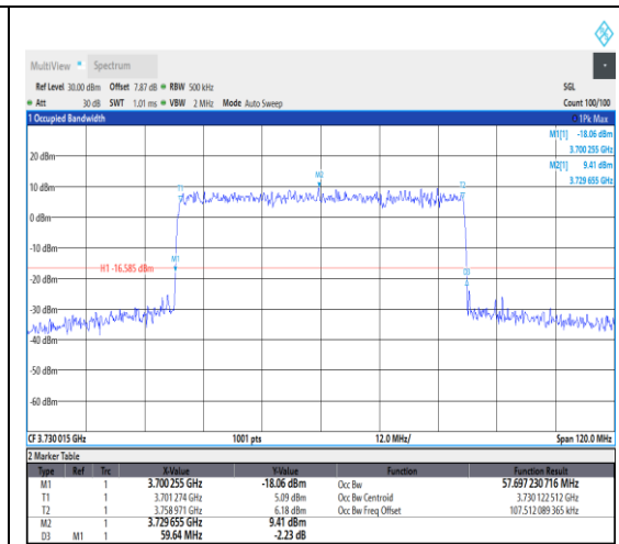
1-N77-3700-3980--30-60-L-5-DFT-256QAM-Outer_Full-162@0-Ant1-57.697-59.640-≤60-PASS
