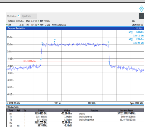
1-N77-3700-3980--30-60-H-1-DFT-QPSK-Outer_Full-162@0-Ant1-56.829-59.400-≤60-PASS
