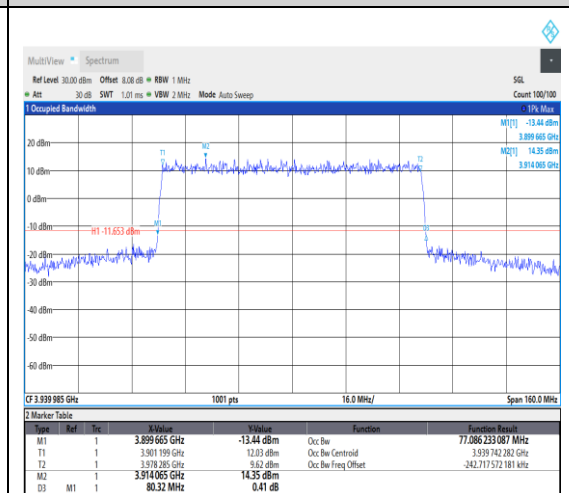
1-N77-3700-3980--30-80-H-3-DFT-16QAM-O
