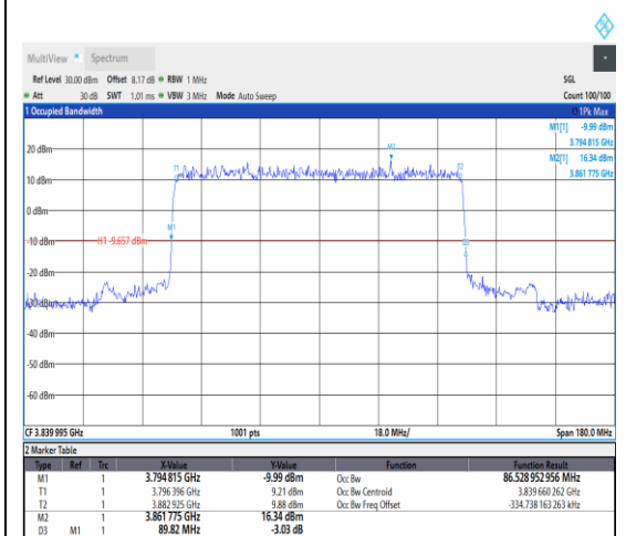
1-N77-3700-3980--30-90-M-2-DFT-PI2BPSK-Outer_Full-243@0-Ant1-86.529-89.820≤90-PASS
