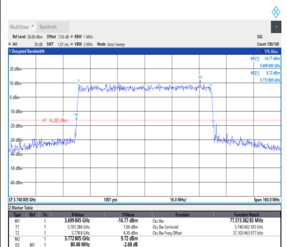
1-N77-3700-3980--30-80-L-9-CP-256QAM-Outer_Full-217@0-Ant1-77.515-80.480-≤80-PA SS
