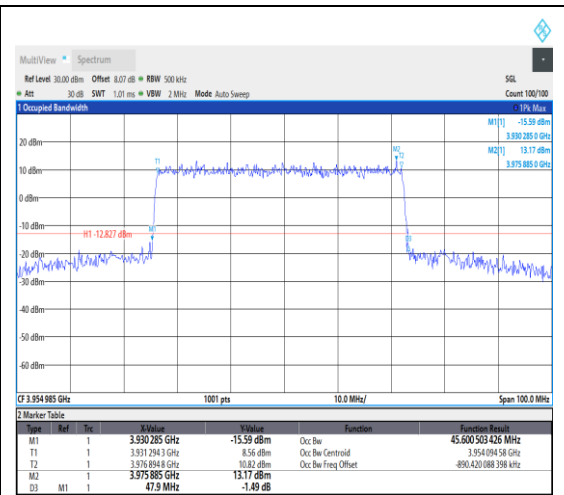
1-N77-3700-3980--30-50-H-4-DFT-64QAM-Outer_Full-128@0-Ant1-45.601-47.900-<=50-PA SS
