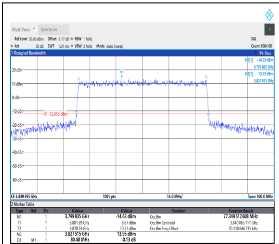
1-N77-3700-3980--30-80-M-7-CP-16QAM-Outer_Full-217@0-Ant1-77.35-80.480-≤80-PA SS
