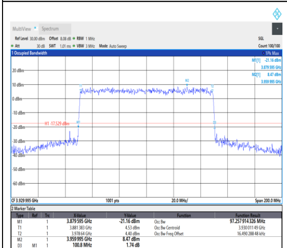
1-N77-3700-3980--30-100-H-9-CP-256QAM-
