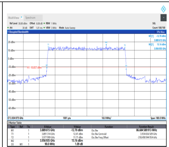
1-N77-3700-3980--30-90-H-2-DFT-PI2BPSK-Outer_Full-243@0-Ant1-86.685-90.000-<=90-PASS
