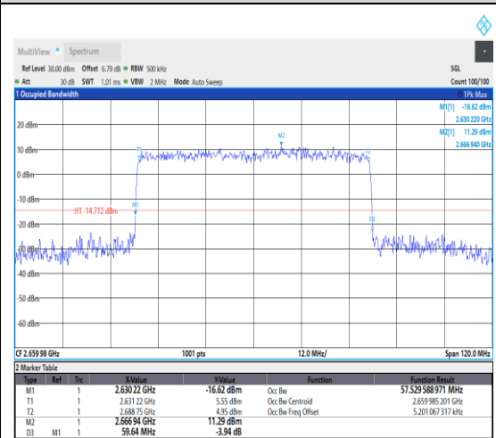
1-N41--30-60-H-6-CP-QPSK-Outer_Full-162 @0-Ant1-57.53-59.640-≤60-PASS
