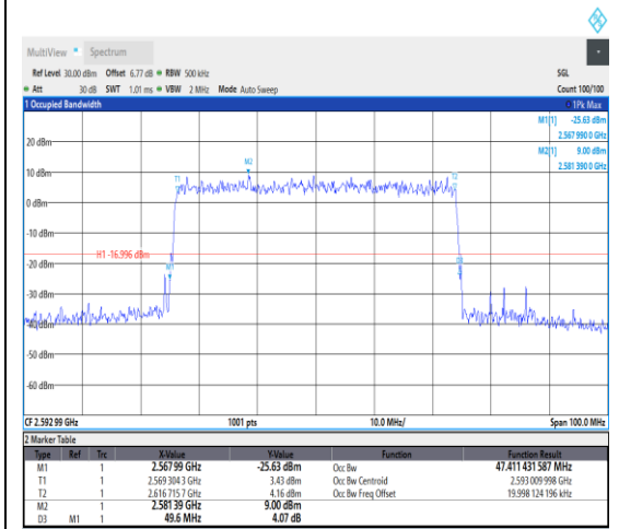
1-N41--30-50-M-9-CP-256QAM-Outer_Full-1 33@0-Ant1-47.411-49.600-≤50-PASS
