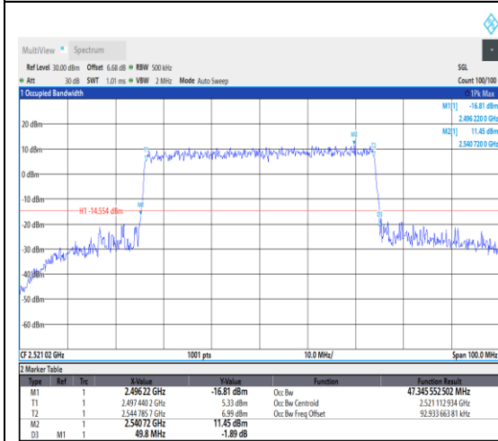
1-N41--30-50-L-8-CP-64QAM-Outer_Full-133 @0-Ant1-47.346-49.800-≤50-PASS
