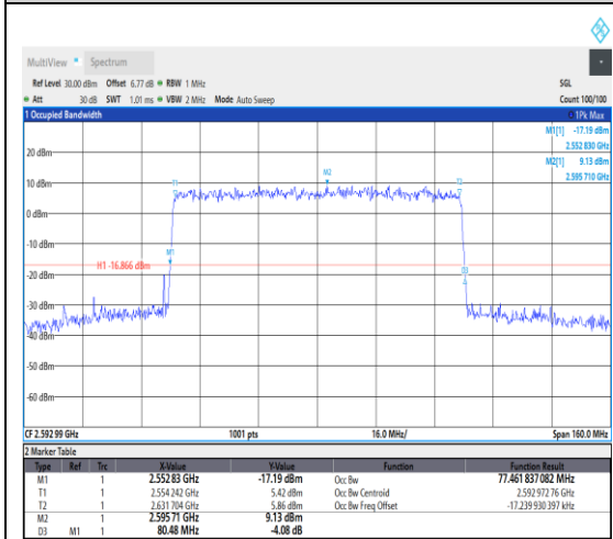
1-N41--30-80-M-9-CP-256QAM-Outer_Full-2 17@0-Ant1-77.462-80.480-≤80-PASS
