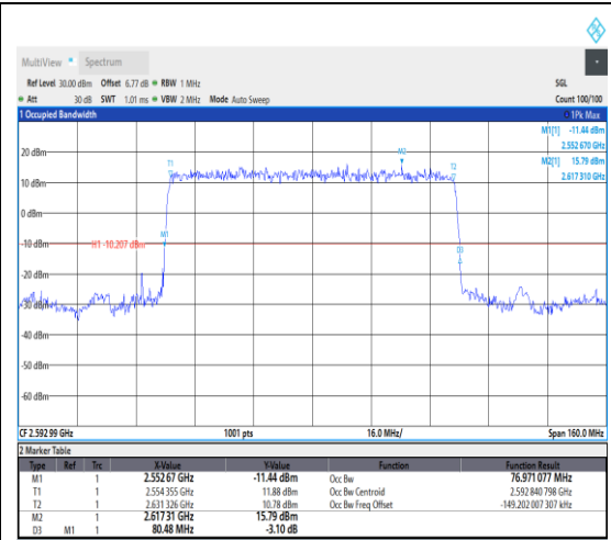
1-N41--30-80-M-2-DFT-PI2BPSK-Outer_Full-216@0-Ant1-76.971-80.480-≤80-PASS
