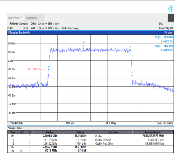
1-N41--30-80-H-1-DFT-QPSK-Outer_Full-21 6@0-Ant1-76.983-80.160-≤80-PASS
