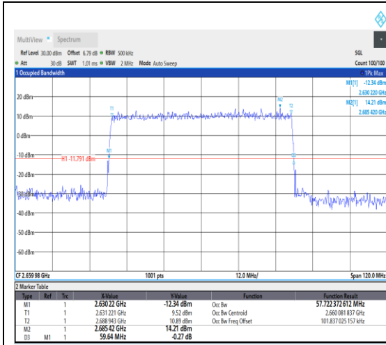
1-N41--30-60-H-1-DFT-QPSK-Outer_Full-16 2@0-Ant1-57.722-59.640-≤60-PASS
