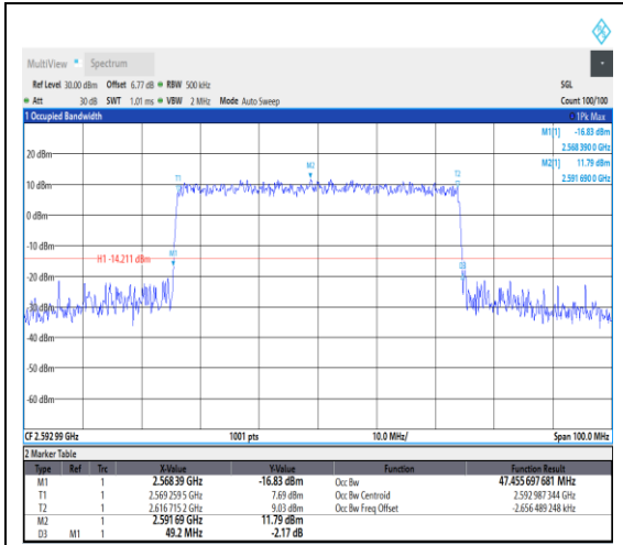
1-N41--30-50-M-7-CP-16QAM-Outer_Full-13 3@0-Ant1-47.456-49.200-≤50-PASS
