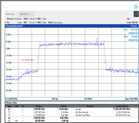
1-N41--30-80-L-6-CP-QPSK-Outer_Full-217 @0-Ant1-25.676-27.200-≤80-PASS
