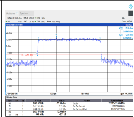
1-N41--30-80-H-7-CP-16QAM-Outer_Full-21 7@0-Ant1-77.315-80.800-≤80-PASS
