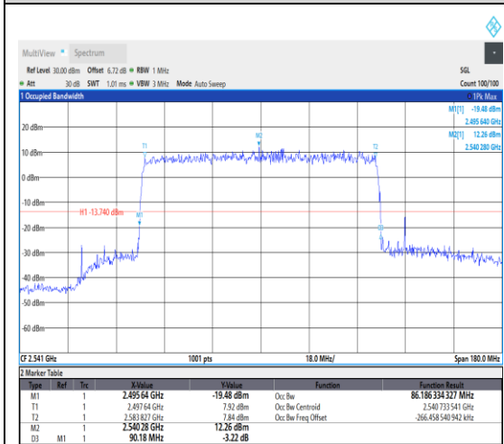
1-N41--30-90-L-5-DFT-256QAM-Outer_Full-243 @0-Ant1-86.186-90.180-≤90-PASS
