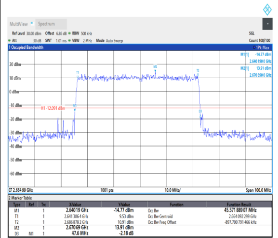
1-N41--30-50-H-3-DFT-16QAM-Outer_Full-1 28@0-Ant1-45.572-47.600-≤50-PASS
