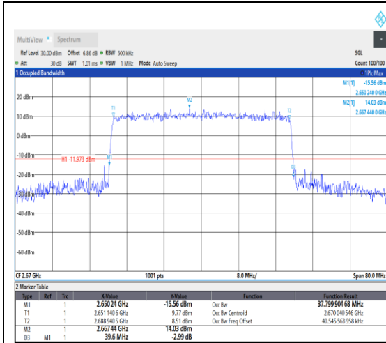
1-N41--30-40-H-7-CP-16QAM-Outer_Full-10 6@0-Ant1-37.8-39.600-≤40-PASS
