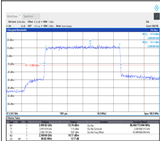
1-N41--30-90-L-3-DFT-16QAM-Outer_Full-243 @0-Ant1-86.465-89.820-≤90-PASS
