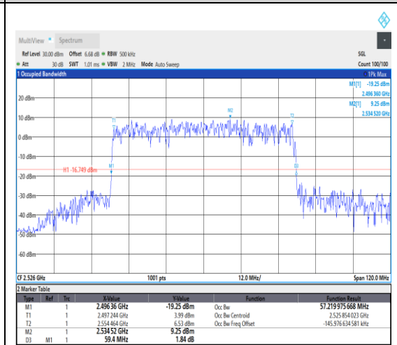
1-N41--30-60-L-6-CP-QPSK-Outer_Full-162 @0-Ant1-57.22-59.400-≤60-PASS
