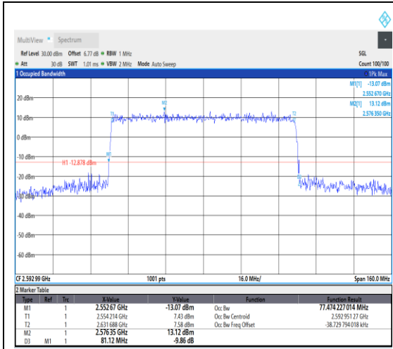
1-N41--30-80-M-7-CP-16QAM-Outer_Full-21 7@0-Ant1-77.474-81.120-≤80-PASS
