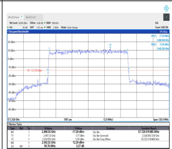
1-N41--30-60-L-4-DFT-64QAM-Outer_Full-16 2 @0-Ant1-57.724-59.760-≤60-PASS
