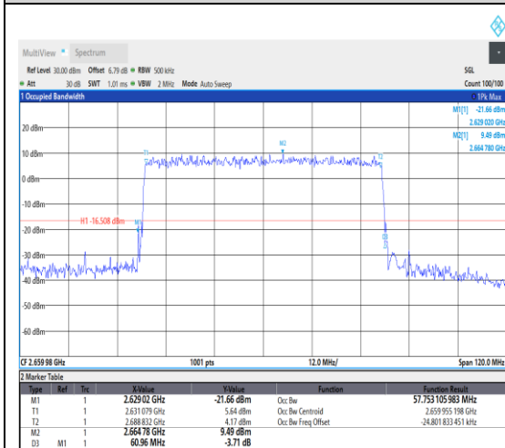
1-N41--30-60-H-5-DFT-256QAM-Outer_Full-1 162@0-Ant1-57.753-60.960-≤60-PASS
