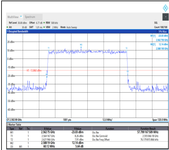
1-N41--30-60-M-4-DFT-64QAM-Outer_Full-1 62@0-Ant1-57.799-60.120-<60-PASS
