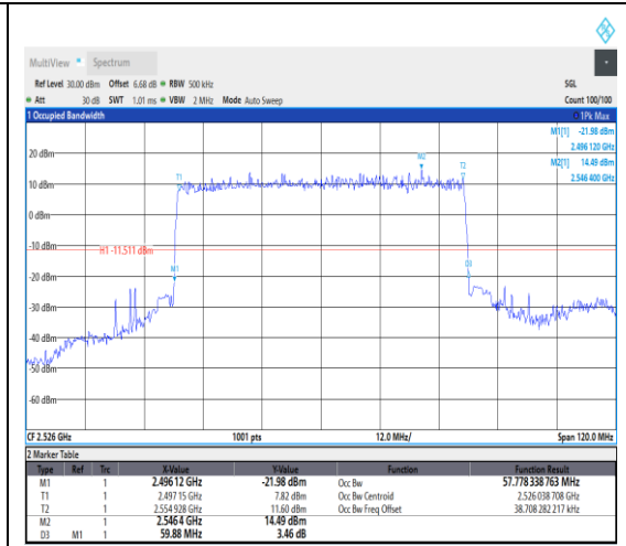
1-N41--30-60-L-2-DFT-PI2BPSK-Outer_Full-162 @0-Ant1-57.778-59.880-≤60-PASS
