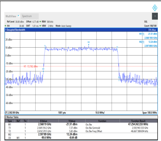
1-N41--30-50-M-8-CP-64QAM-Outer_Full-13 3@0-Ant1-47.254-49.600-≤50-PASS
