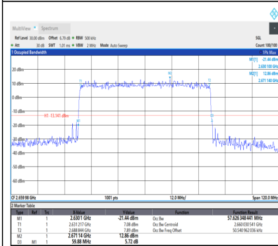
1-N41--30-60-H-3-DFT-16QAM-Outer_Full-1 62@0-Ant1-57.626-59.880-≤60-PASS
