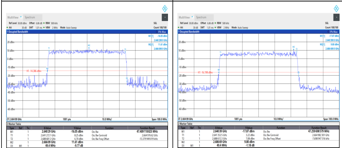
1-N41--30-50-H-8-CP-64QAM-Outer_Full-13 3@0-Ant1-47.409-49.400-≤50-PASS 1-N41--30-50-H-9-CP-256QAM-Outer_Full-1 33@0-Ant1-47.26-49.400-≤50-PASS
