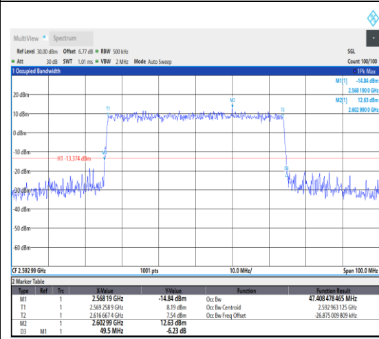
1-N41--30-50-M-6-CP-QPSK-Outer_Full-133 @0-Ant1-47.408-49.500-≤50-PASS
