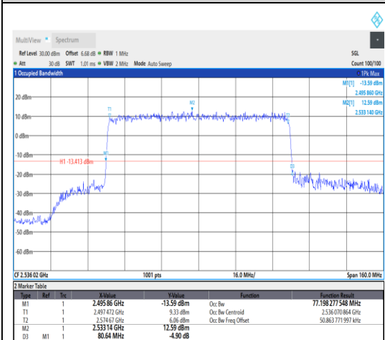
1-N41--30-80-L-8-CP-64QAM-Outer_Full-217 @0-Ant1-77.198-80.640-≤80-PASS
