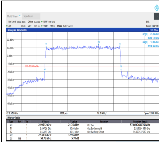
1-N41--30-60-L-1-DFT-QPSK-Outer_Full-162 @0-Ant1-57.67-59.760-≤60-PASS
