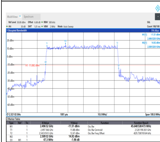
1-N41--30-50-L-2-DFT-PI2BPSK-Outer_Full-128 128@0-Ant1-45.649-47.300-≤50-PASS
