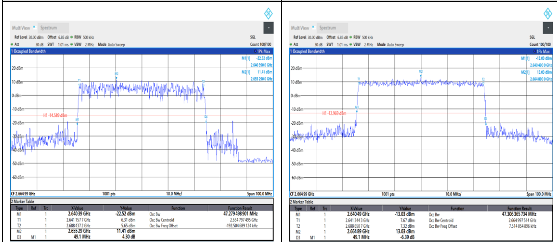
1-N41--30-50-H-6-CP-QPSK-Outer_Full-133 @0-Ant1-47.279-49.100-≤50-PASS 1-N41--30-50-H-7-CP-16QAM-Outer_Full-13 3@0-Ant1-47.306-49.100-≤50-PASS
