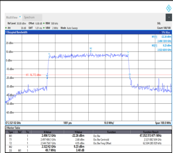
1-N41--30-50-L-9-CP-256QAM-Outer_Full-13 3@0-Ant1-47.352-49.700-≤50-PASS
