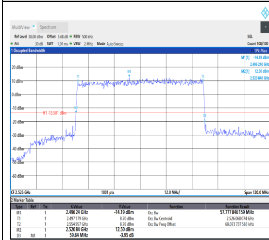
1-N41--30-60-L-3-DFT-16QAM-Outer_Full-16 2 @0-Ant1-57.778-59.640-≤60-PASS
