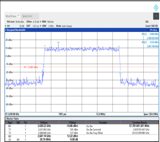
1-N41--30-60-H-4-DFT-64QAM-Outer_Full-1 62@0-Ant1-57.782-59.760-≤60-PASS
