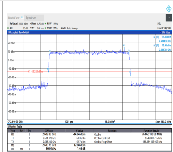
1-N41--30-80-H-5-DFT-256QAM-Outer_Full-216@0-Ant1-76.86-80.000-≤80-PASS
