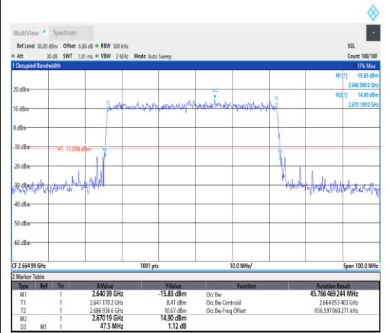
1-N41--30-50-H-1-DFT-QPSK-Outer_Full-12 8@0-Ant1-45.766-47.500-≤50-PASS
