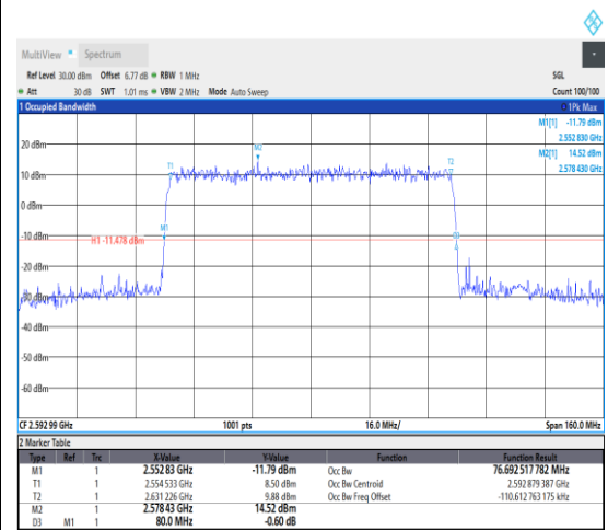
1-N41--30-80-M-4-DFT-64QAM-Outer_Full-2 16@0-Ant1-76.693-80.000-≤80-PASS
