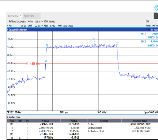
1-N41--30-50-L-1-DFT-QPSK-Outer_Full-128 @0-Ant1-45.663-47.700-≤50-PASS
