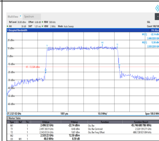
1-N41--30-50-L-3-DFT-16QAM-Outer_Full-12 8@0-Ant1-45.747-48.000-≤50-PASS
