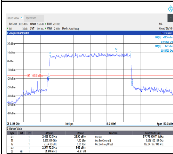
1-N41--30-60-L-5-DFT-256QAM-Outer_Full-1 62 @0-Ant1-57.776-59.880-≤60-PASS
