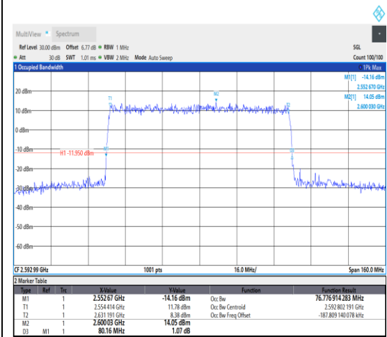
1-N41--30-80-M-3-DFT-16QAM-Outer_Full-2 16@0-Ant1-76.777-80.160-≤80-PASS
