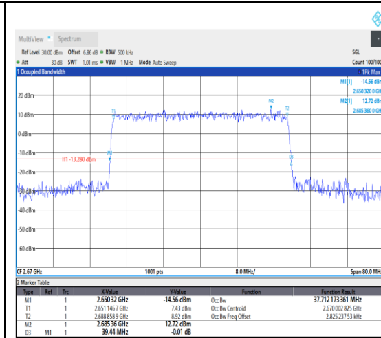
1-N41--30-40-H-8-CP-64QAM-Outer_Full-10 6@0-Ant1-37.712-39.440-≤40-PASS
