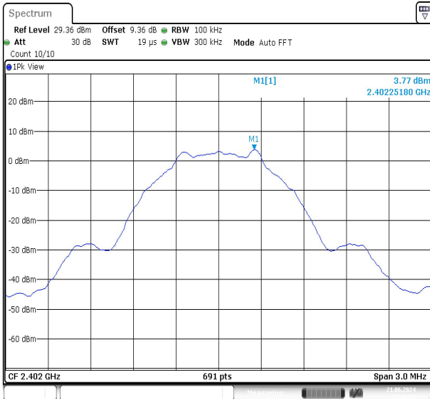
BLE_1M-Ant1-2402-0~Reference-PASS
