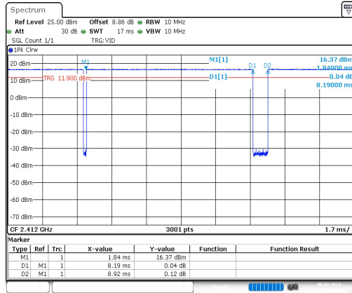
NTNV-11B-Ant1-2412
