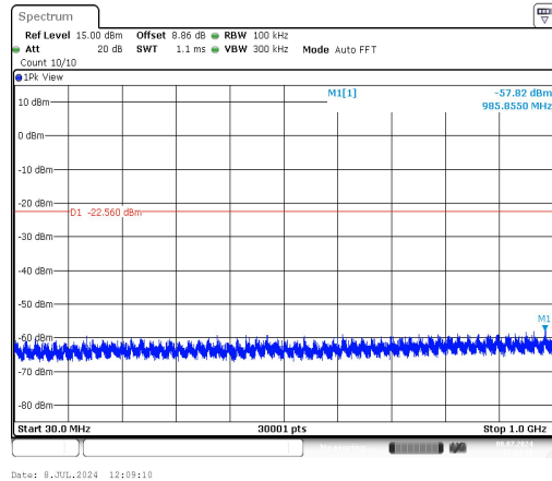
11N20SISO-Ant1-2412-30~1000-PASS
