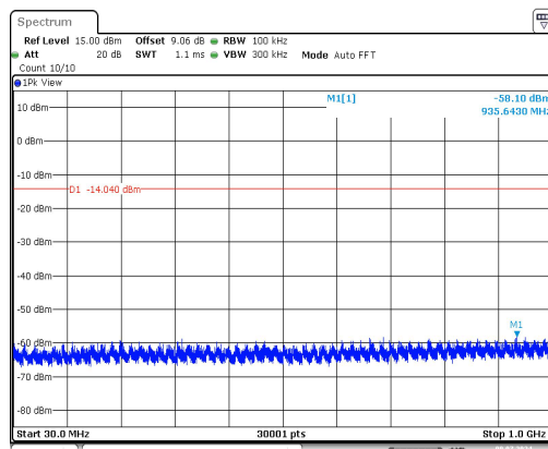
11B-Ant1-2462-30~1000-PASS
