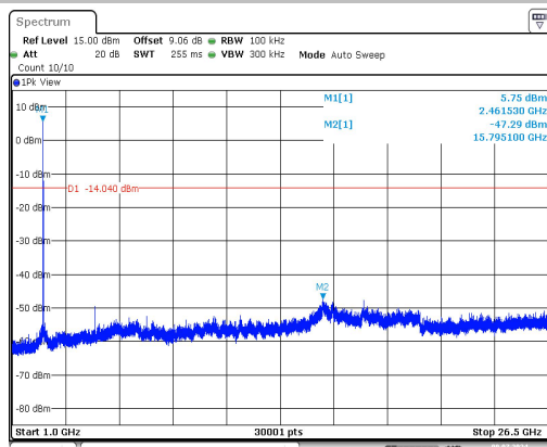
11B-Ant1-2462-0~Reference-PASS
