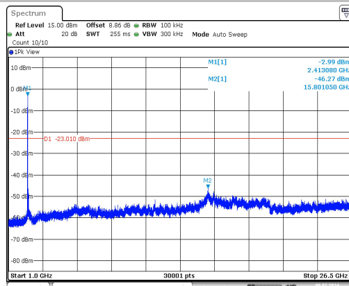
11G-Ant1-2412-0~Reference-PASS
