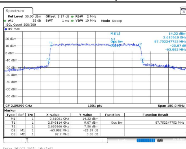
n41 SCS=30kHz CP_QAM64 BW=90MHz Channel=518598 RB=245@0
