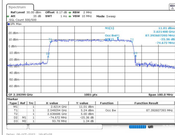
n41 SCS=30kHz CP_QAM256 BW=90MHz Channel=518598 RB=245@0
