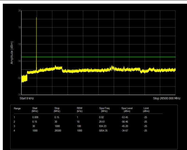
n38 SCS=30kHz DFT_BPSK BW=20MHz Channel=516000 RB=1@50
