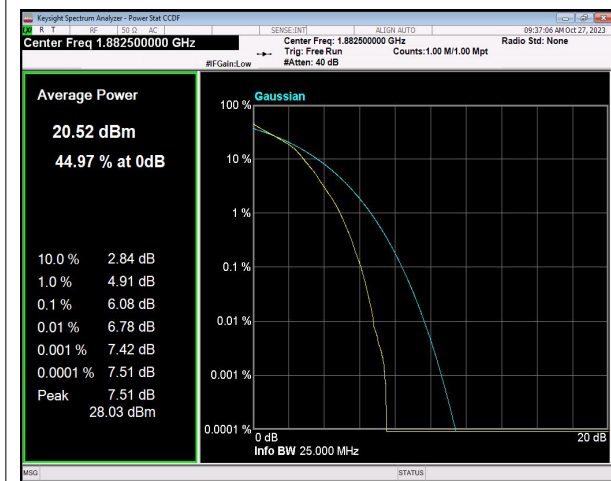
n25 SCS=15kHz DFT_QAM16 BW=20MHz Channel=376500 RB=100@0
