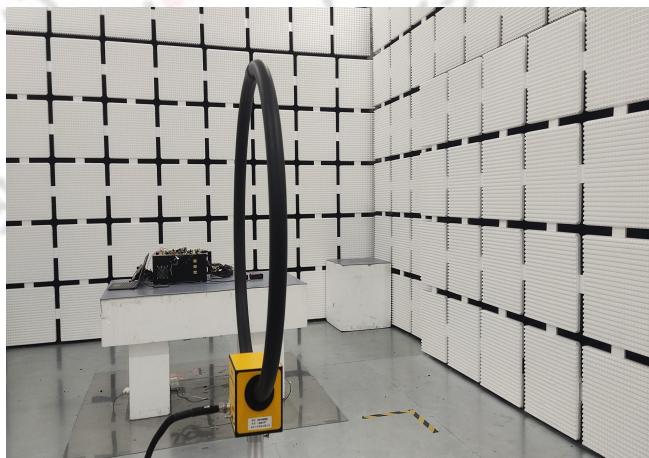
Radiated Emissions for 30MHz-1GHz
