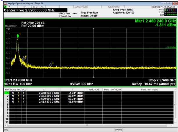
GFSK: Band Edge, Right Side
