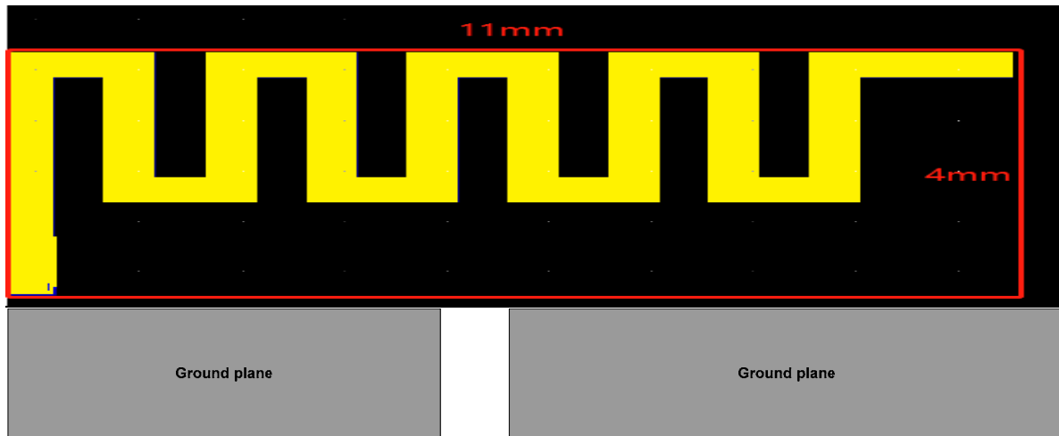
Figure 1. IFA Dimensions
