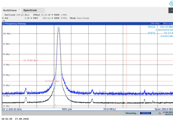
Figure 7.7-12: Radiated band edge spurious emissions at low band edge
