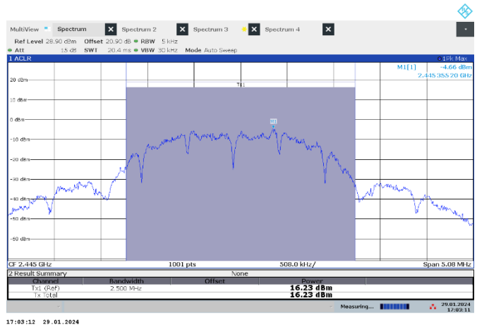
Figure 7.6-2: Output power on mid channel
