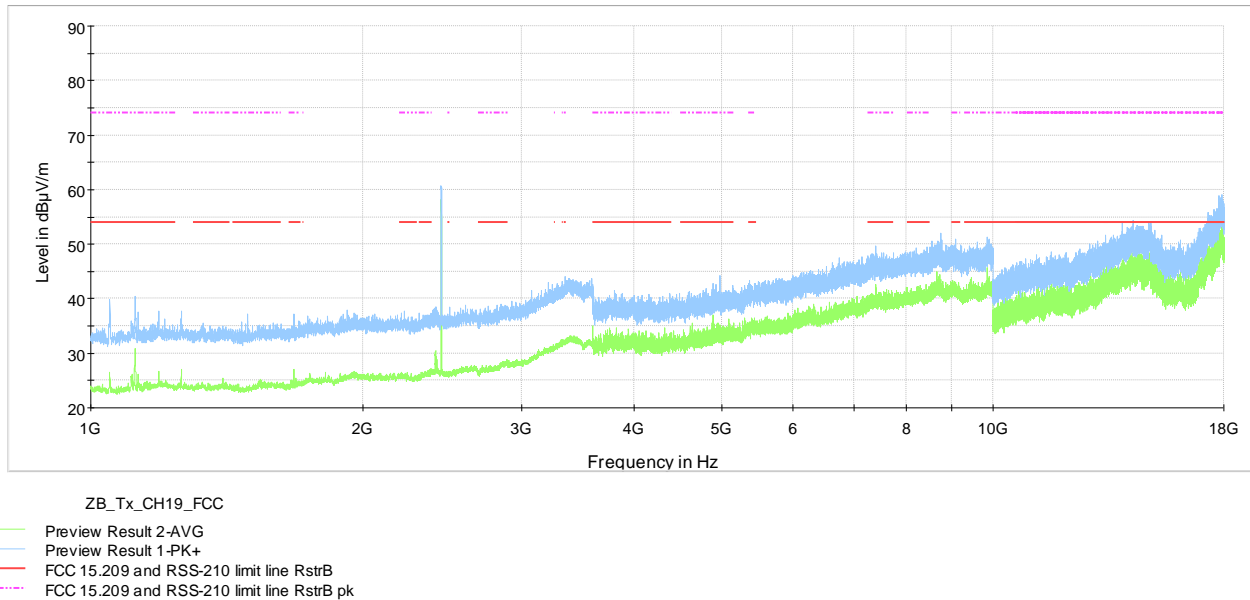
Figure 7.7-7: radiated spurious emissions from 1 GHz to 18 GHz at mid channel
