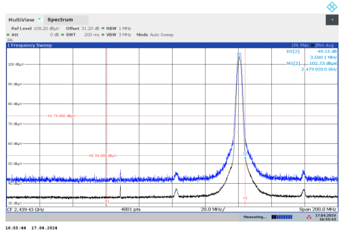
Figure 7.7-13: Radiated band edge spurious emissions at high band edge
