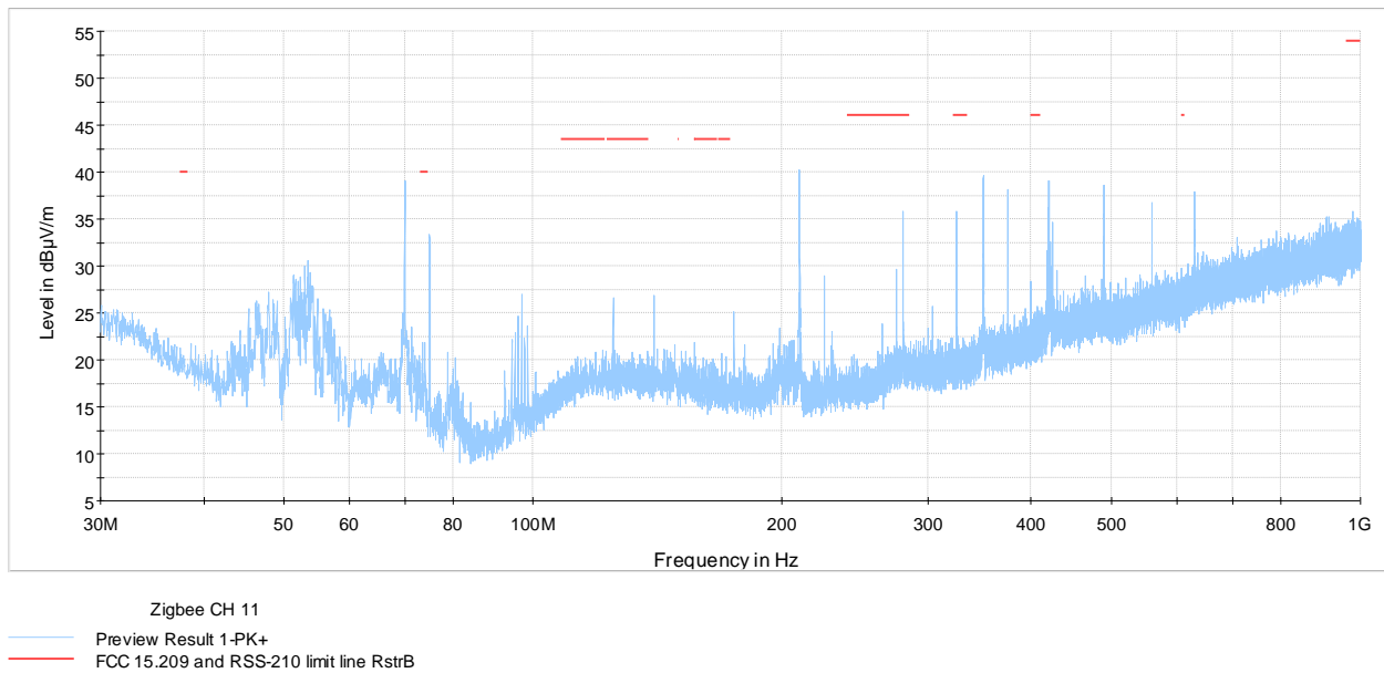
Figure 7.7-3: radiated spurious emissions from 30 MHz to 1000 MHz at low channel
