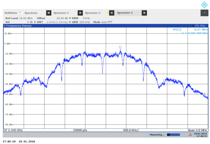
Figure 7.8-2: Power spectral density on mid channel
