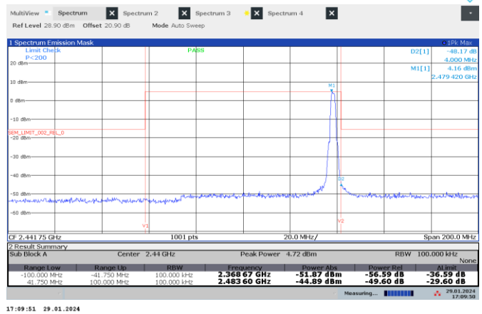
Figure 7.7-2: Conducted Band edge spurious emissions at high band edge
