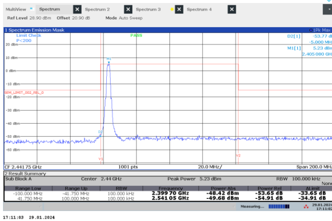
Figure 7.7-1: Conducted Band edge spurious emissions on at low band edge
