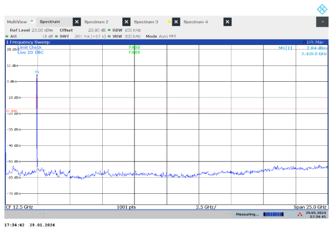
Figure 7.7-15: Conducted spurious emissions for 802.11b, 1 Mbps data rate, mid channel
