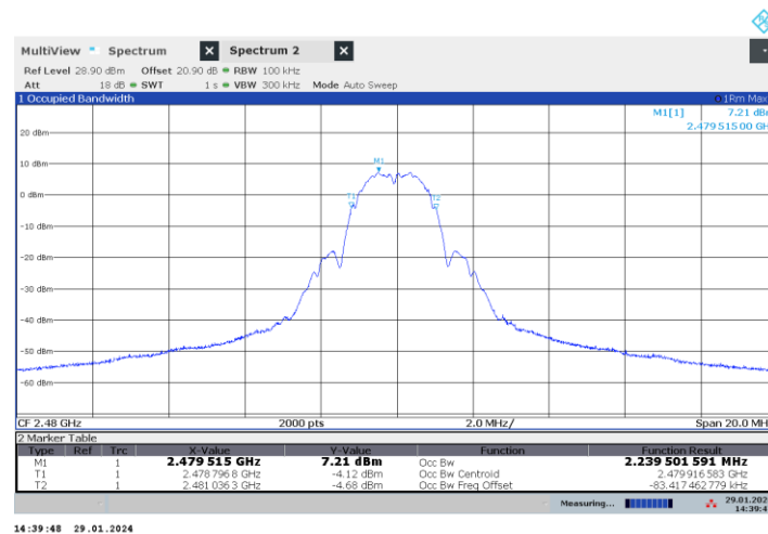
Figure 7.5-6: 99% occupied bandwidth on high channel
