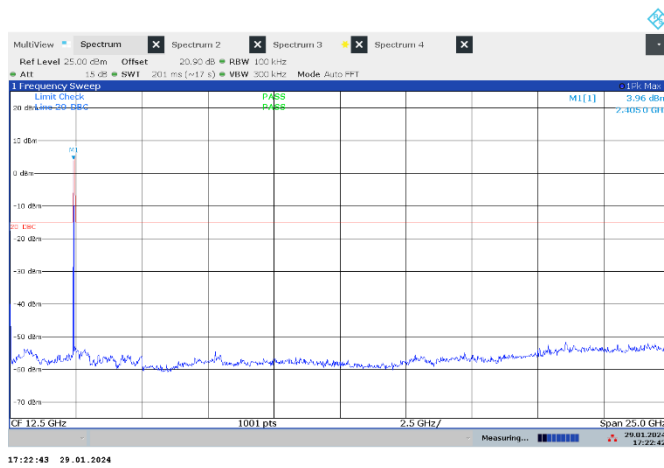
Figure 7.7-14: Conducted spurious emissions for 802.11b, 1 Mbps data rate, low channel
