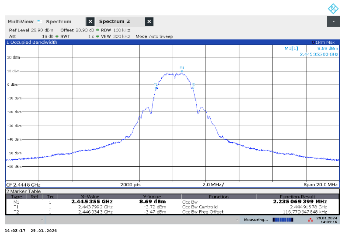
Figure 7.5-5: 99% occupied bandwidth on mid channel
