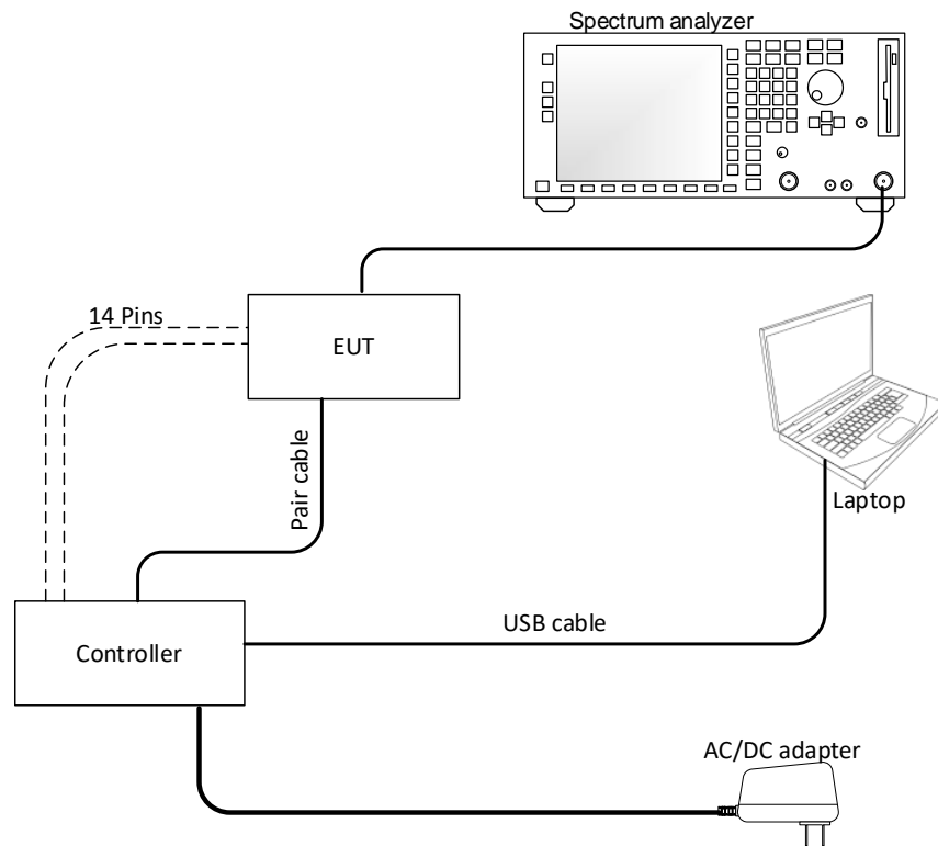
Figure 4.5-2: Antenna port testing block diagram
