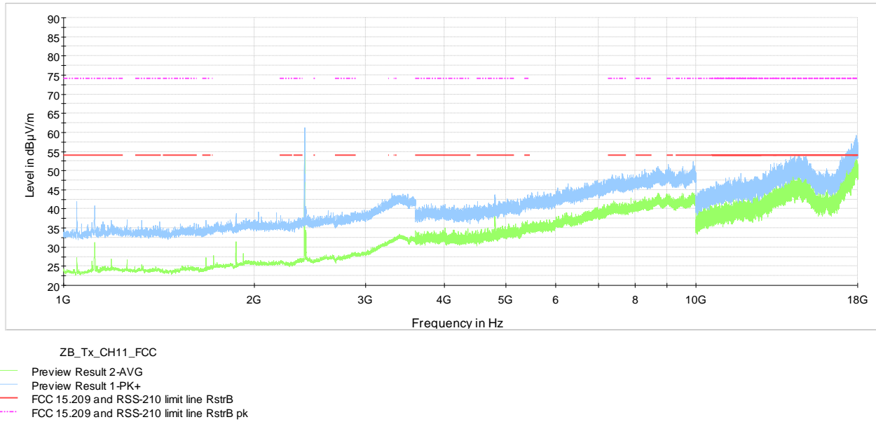
Figure 7.7-6: radiated spurious emissions from 1 GHz to 18 GHz at low channel
