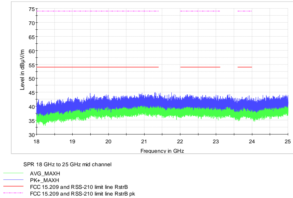
Figure 7.7-10: radiated spurious emissions from 18 GHz to 25 GHz at mid channel
