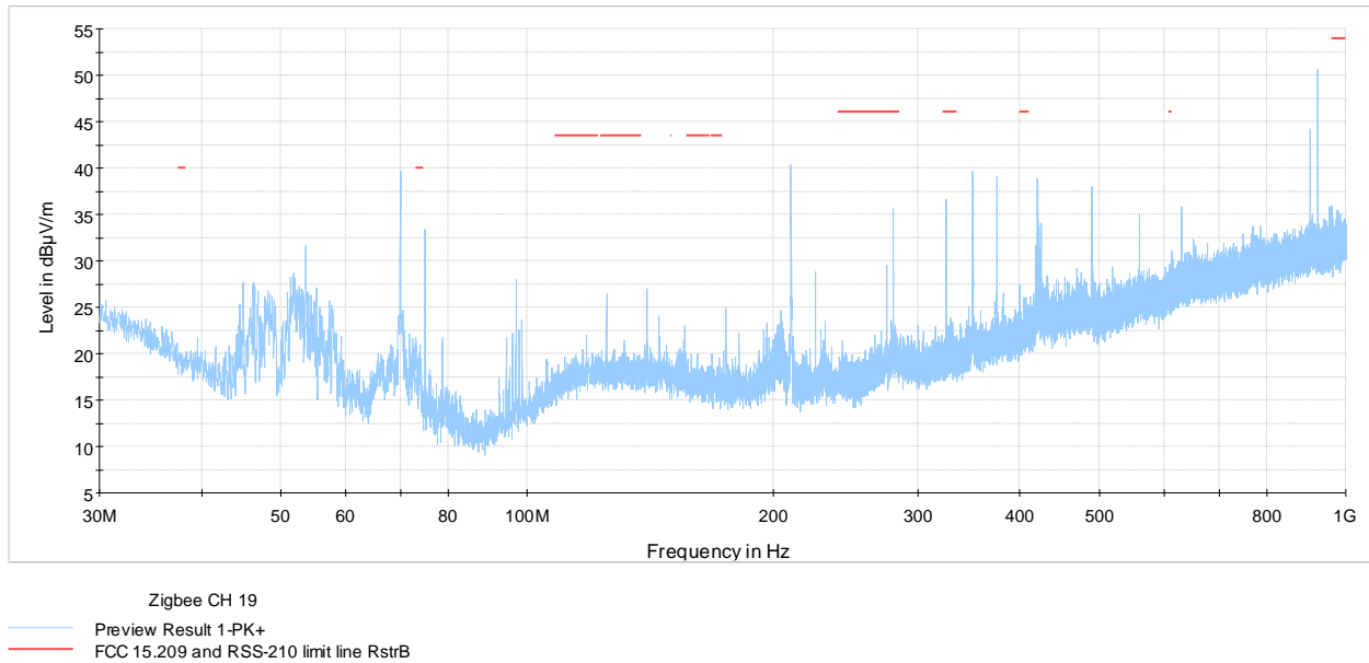
Figure 7.7-4: radiated spurious emissions from 30 MHz to 1000 MHz at mid channel
