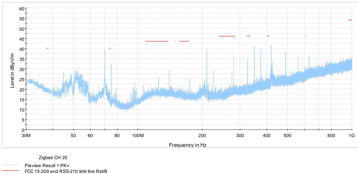
Figure 7.7-5: radiated spurious emissions from 30 MHz to 1000 MHz at high channel
