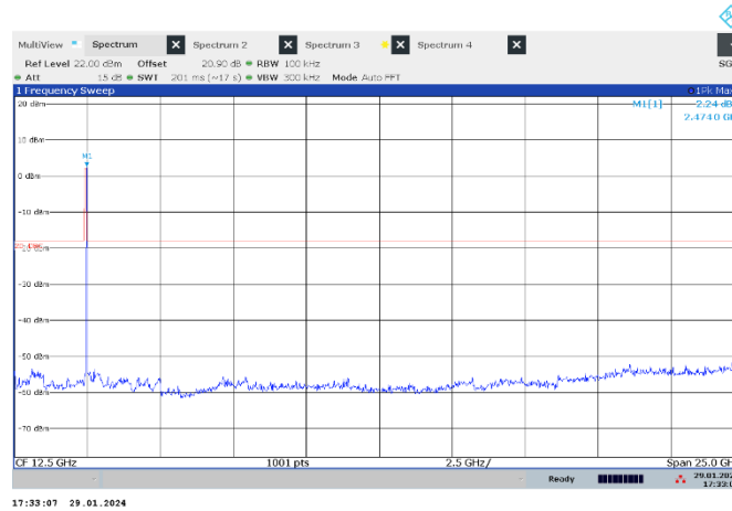
Figure 7.7-16: Conducted spurious emissions for 802.11b, 1 Mbps data rate, high channel
