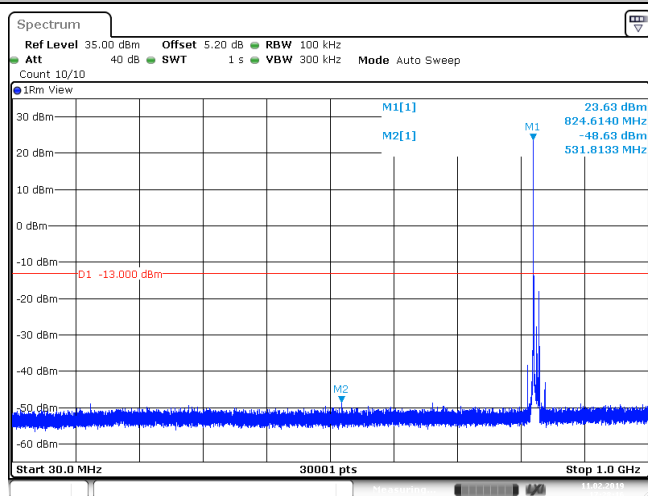
Band5_10MHz_QPSK_20450_1RB#0
