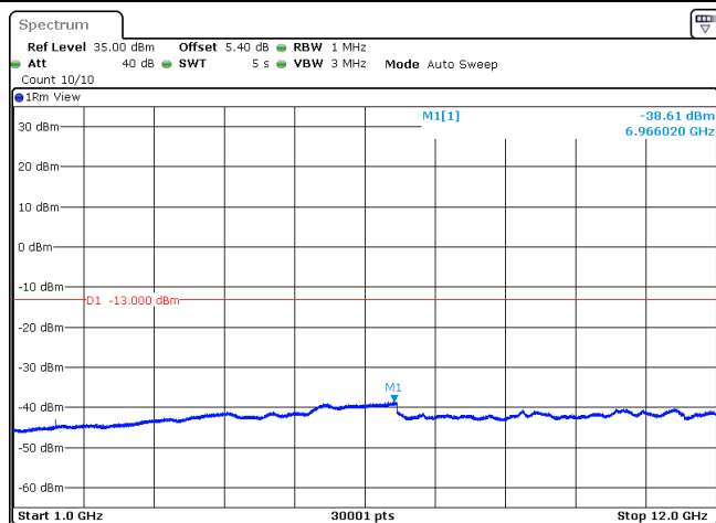
Band5_10MHz_QPSK_20450_1RB#0
