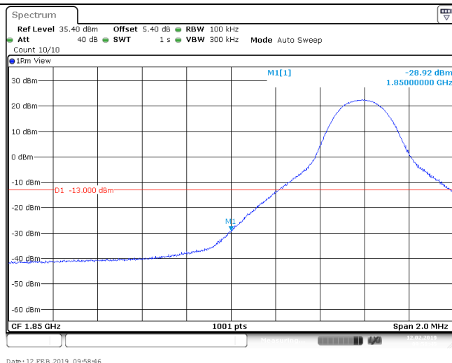
Band25 10MHz QPSK 26090 50RB#0
