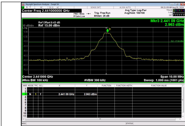
Out Of Band Emission GFSK_DH1_Channel 39
