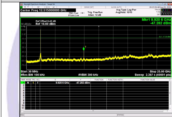
30.0 MHz - 25000.0 MHz GFSK_DH1_Channel 78
