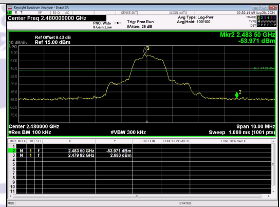
Out Of Band Emission n/4QPSK_2-DH1_Channel 78
