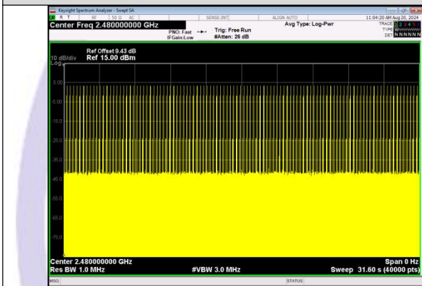
Number of Pulses in 31.6 seconds n/4DQPSK_2-DH5
