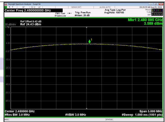
Peak Output Power n/4QPSK_Channel 78
