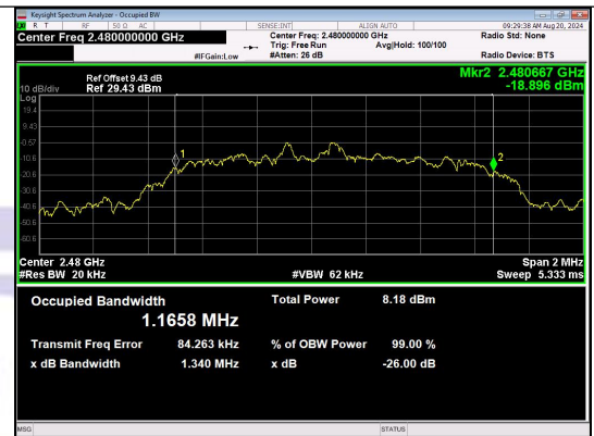
n/4QPSK_2-DH1_Channel 78
