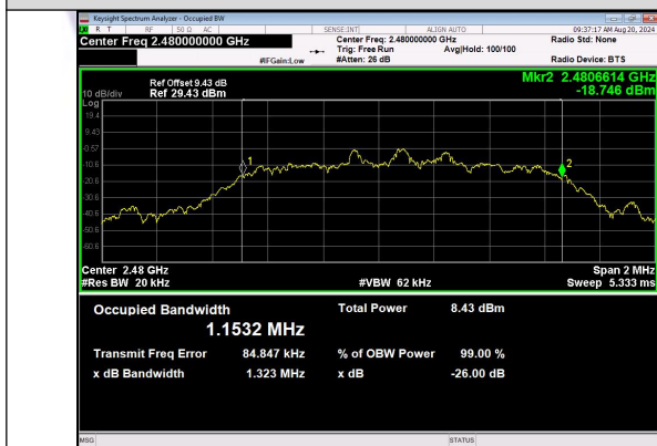
8DPSK_3-DH1_Channel 78
