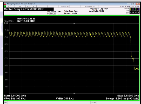
High End Spectrum Channel Hopping Plot n/4DQPSK
