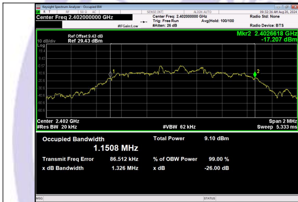
8DPSK_3-DH1_Channel 0
