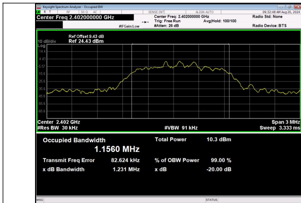
8DPSK_3-DH1_Channel 0
