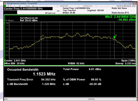
8DPSK_3-DH1_Channel 39
