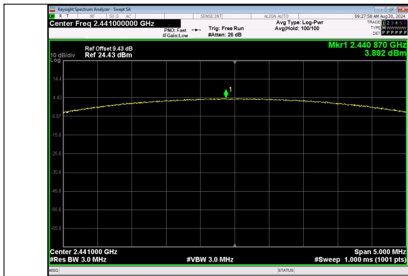
Peak Output Power n/4QPSK_Channel 39
