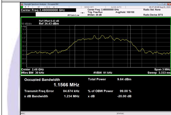
8DPSK_3-DH1_Channel 78
