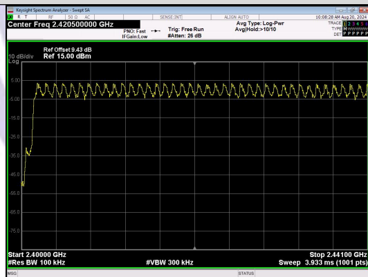
Low End Spectrum Channel Hopping Plot n/4DQPSK
