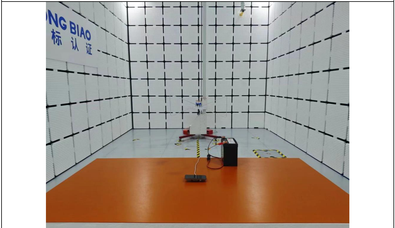
Radiated Emission Above 30MHz
