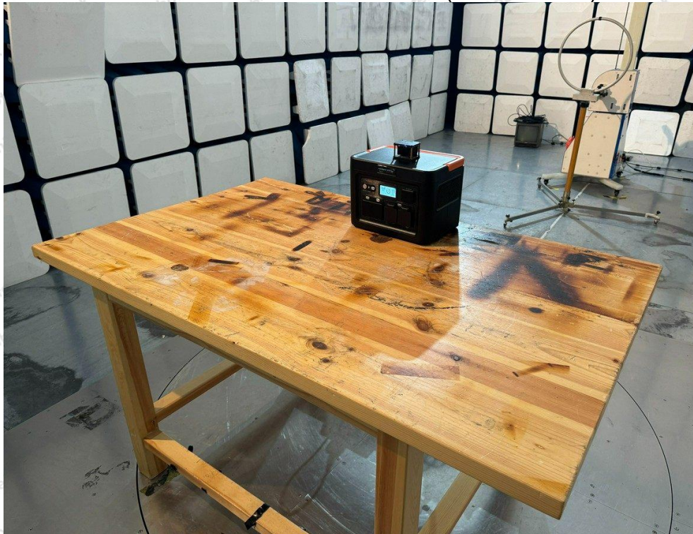
Photo of Radiation Emission Test (below 30MHz)
