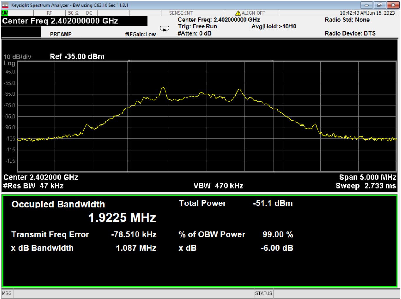
27 Occupied Bandwidth, Low Channel, GMSK
