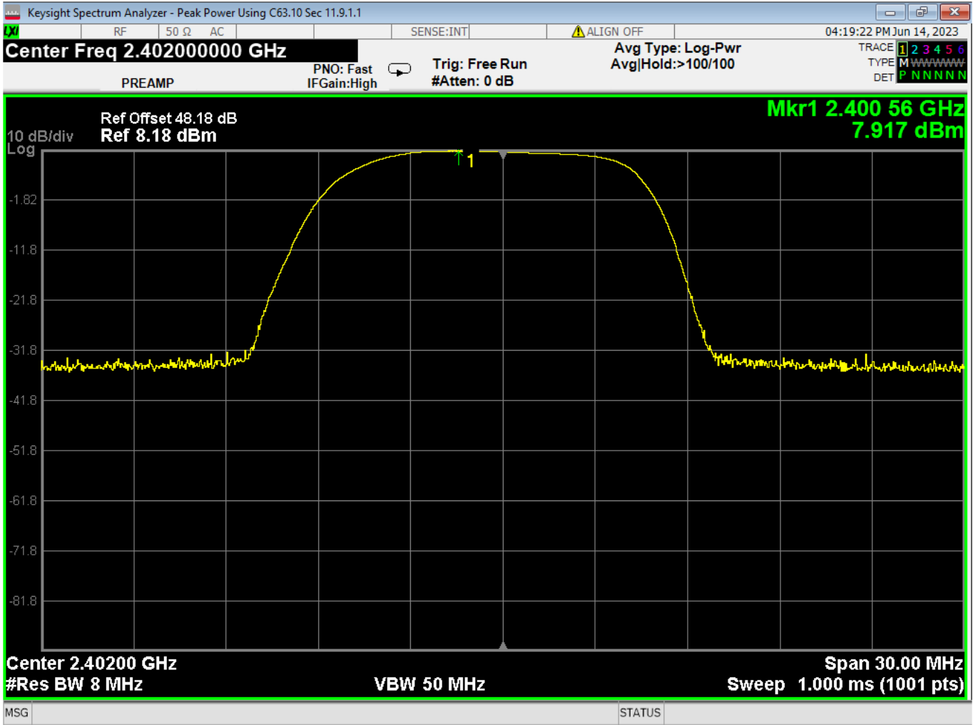
01 Peak Power, Low Channel, GMSK
