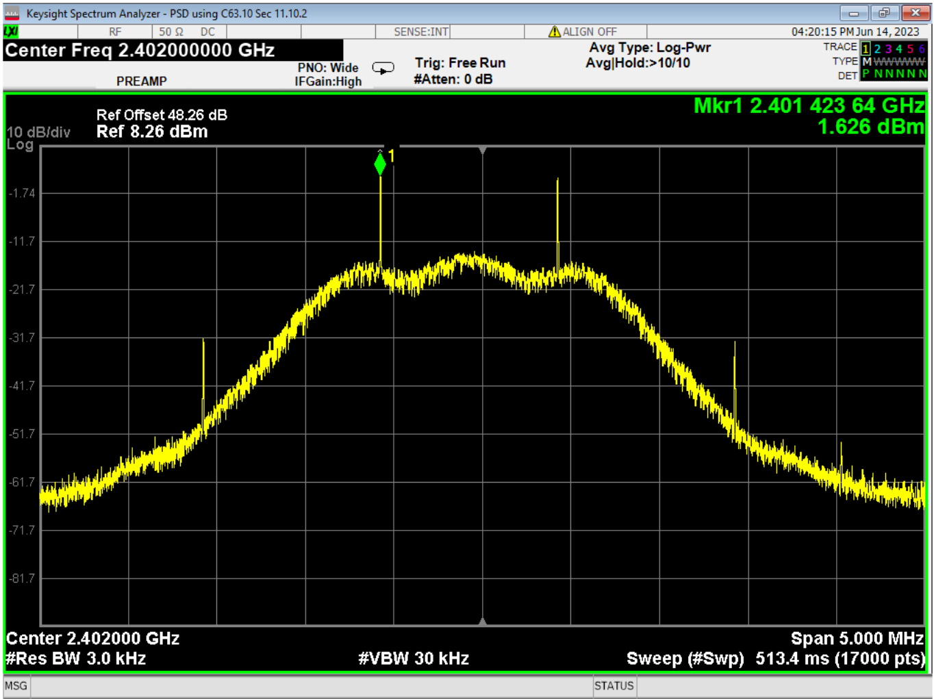
07 PSD, Low Channel, GMSK
