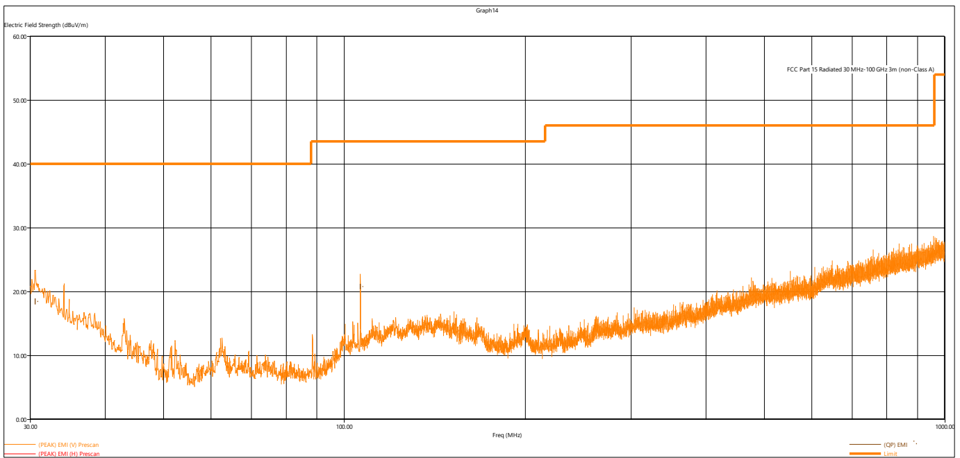
Figure 7 - Radiated Emissions Plot, GMSK, Vertical
