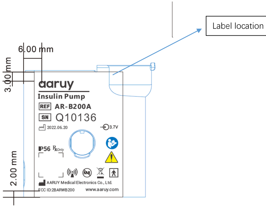
Backside view
