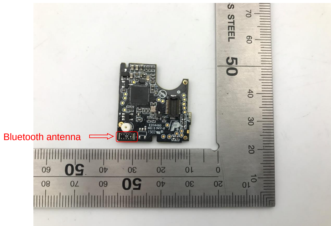
Photo 10 Inside of EUT
