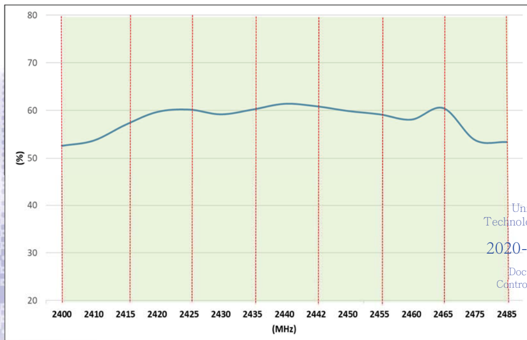
b) Efficiency (%)
