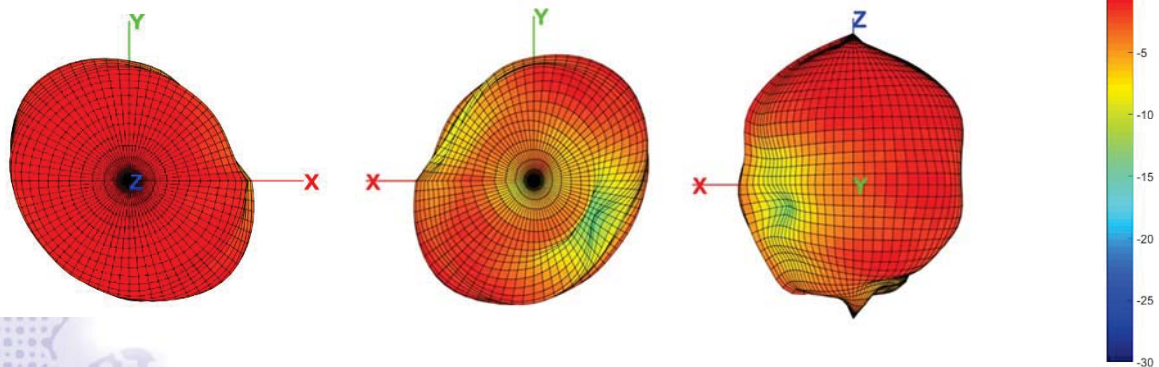
2450 MHz (unit: dBi)
