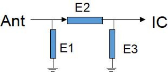
Description of antenna matching circuit
